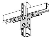
B273 10-HOLE DOUBLE WING CONNECTION
