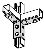
B121 8-HOLE DOUBLE CORNER CONNECTION
