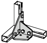
B346 L & R 8-HOLE DOUBLE CORNER GUSSETED CONNECTION
