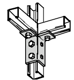
B120 6-HOLE CORNER CONNECTION
