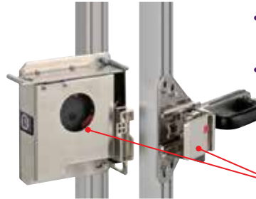
D4JL Slide Bolt Assembly with special slide key
