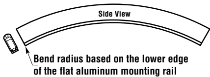
Figure 2 Flat Aluminum Mounting Channel
