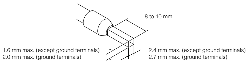
Finished Dimensions of Ferrules
