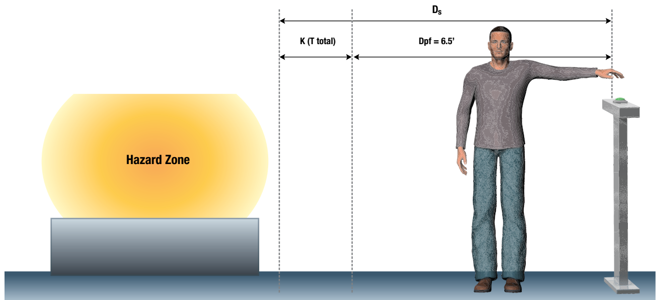
Figure 14: Single control applications
