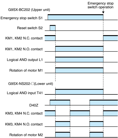
Timing Chart
