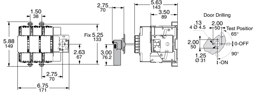
GS1EU3/GS1GU3, GS1 30 A/60 A J
