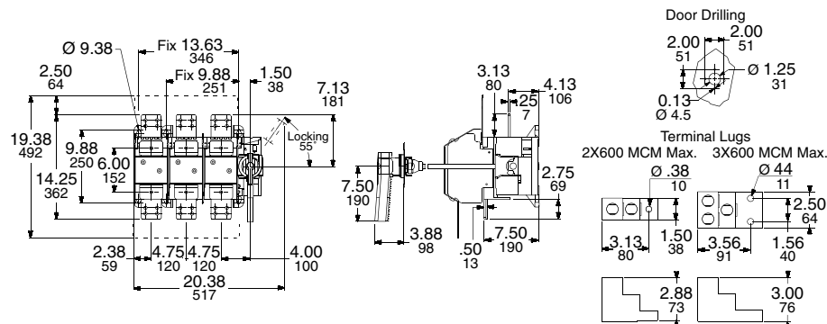
GS1SU3/GS1TU3, GS1 600 A J and 800 A L
