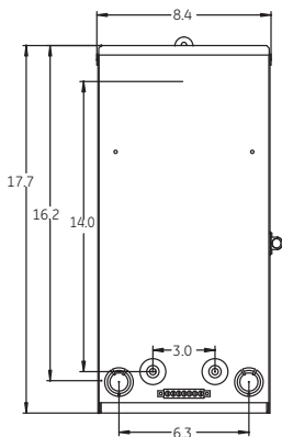
Outline Drawing
