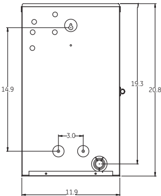
Outline Drawing
