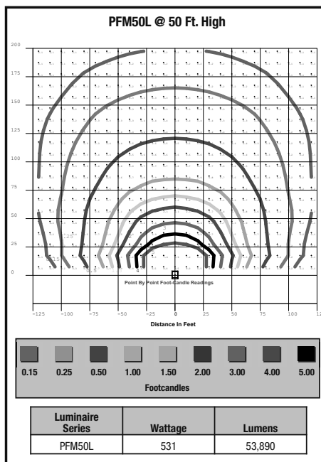
PFM50L Model
