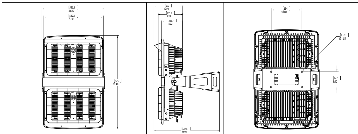
PFM50L Model
