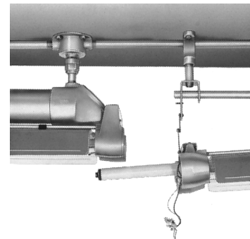
One cover removed and lamp partly withdrawn
