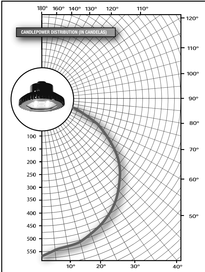
Vaporgard™ LED (22 Watt)
