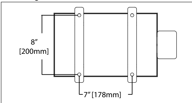
Mounting
