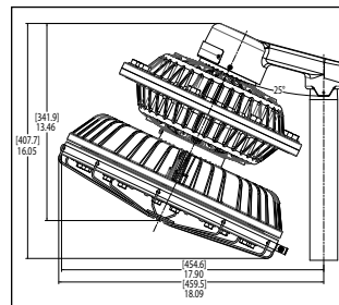
Stanchion Mount
