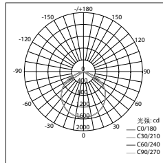
Standard 6000K, 100W Light LPL04-C60-100W
