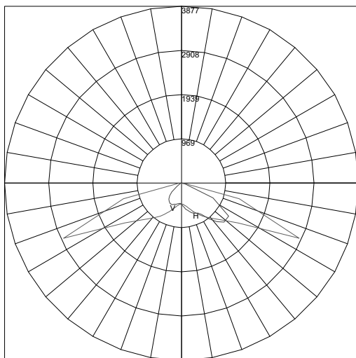
Lumen Multiplier (2 Bar)
