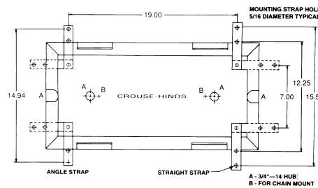
FVS Showing Mounting Strap Positioning
