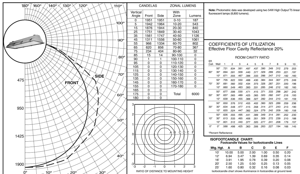
Luminaire with two 54W High Output T5 Linear Fluorescent Lamps FN4254
