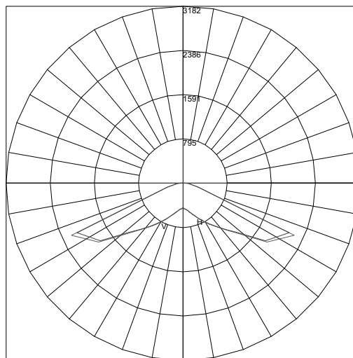
Type V Distribution
