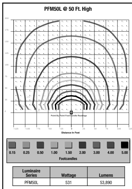
PFM50L Model
