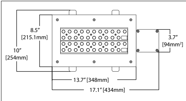
Mounting
