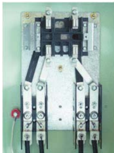
Test Block Bypass
