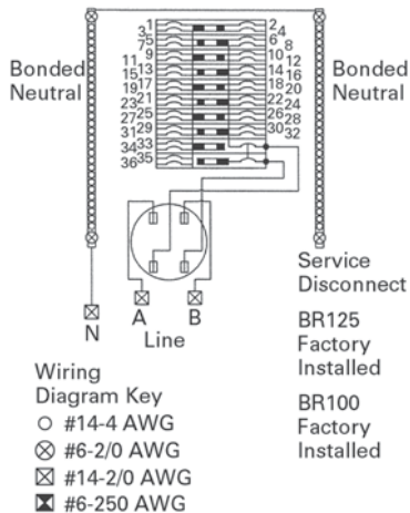
Typical Wiring Diagram for Catalog Numbers MBED1836B100BF, MBED1836B125BF
