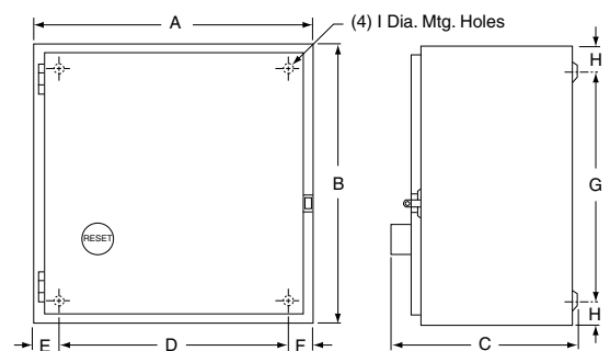
Figure 3—NEMA 1
