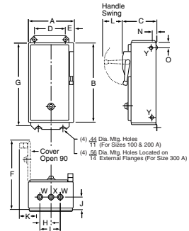
Figure 2 NEMA 1 Enclosure
