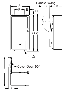
Figure 3 NEMA 12 Enclosure
