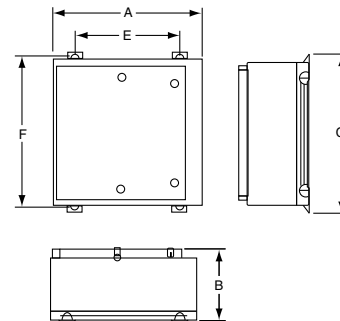
Figure 1 NEMA 4X
