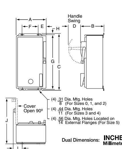
Figure 3: NEMA 12 Enclosure
