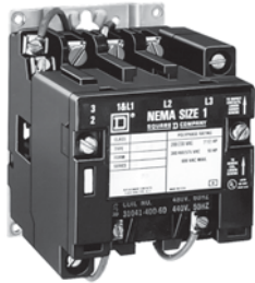
Type SCO2 Size 1, 3-Pole Contactor
