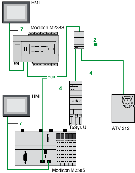
Non isolated link (Modicon M238/M258 master)
