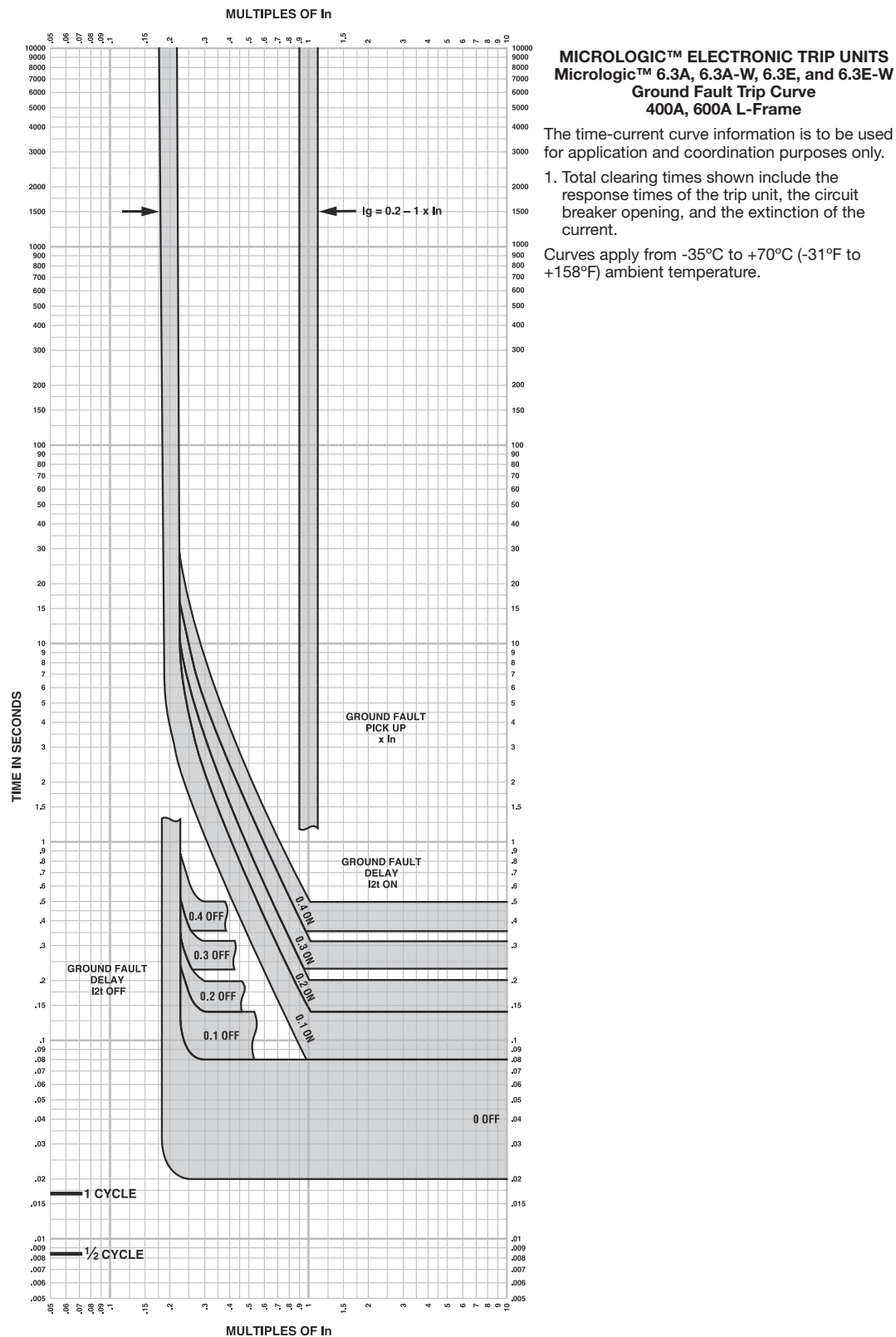
Figure 108: Micrologic 6.3A, 6.3A-W, 6.3E, and 6.3E-W Ground-Fault Trip Curve
