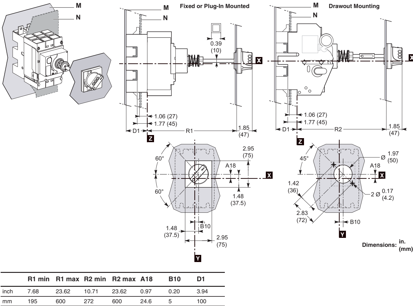
Figure 45: PowerPact L-Frame Circuit Breaker Extended Rotary Handle Mounting
