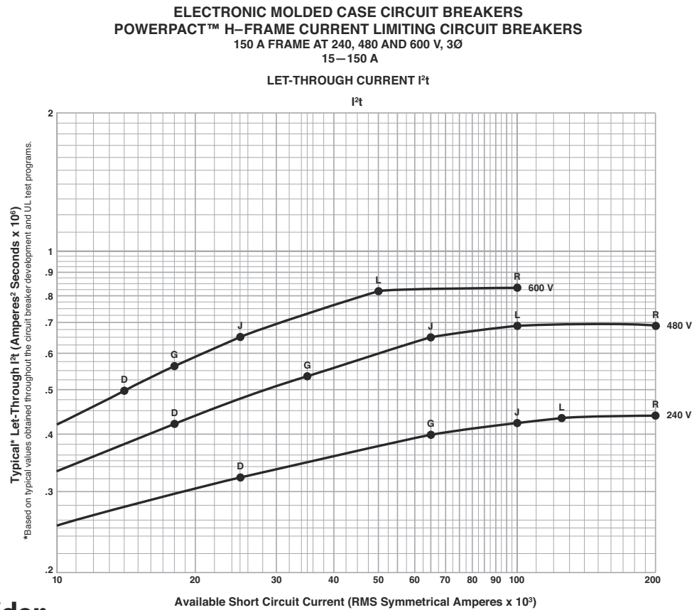
Figure 69: H-Frame 150 A Typical I²t Let-Through Curves
