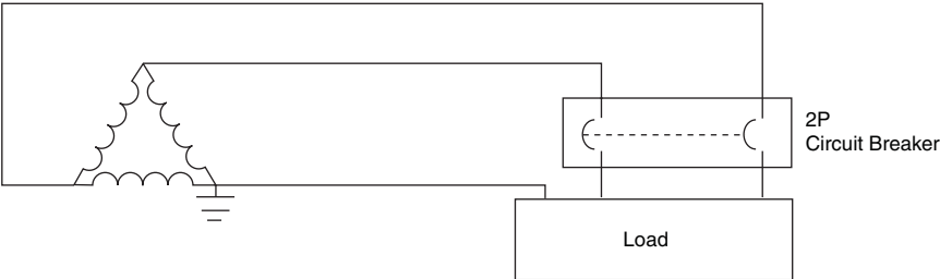
Figure 2: Three-Phase 240 Vac Corner-Grounded Delta System
