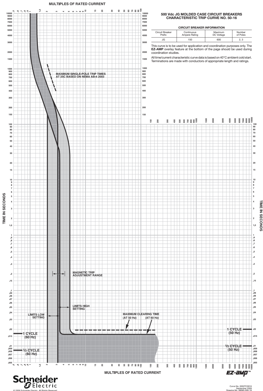
Figure 63: J-Frame 150 A (JG) 500 Vdc Thermal-Magnetic Trip
