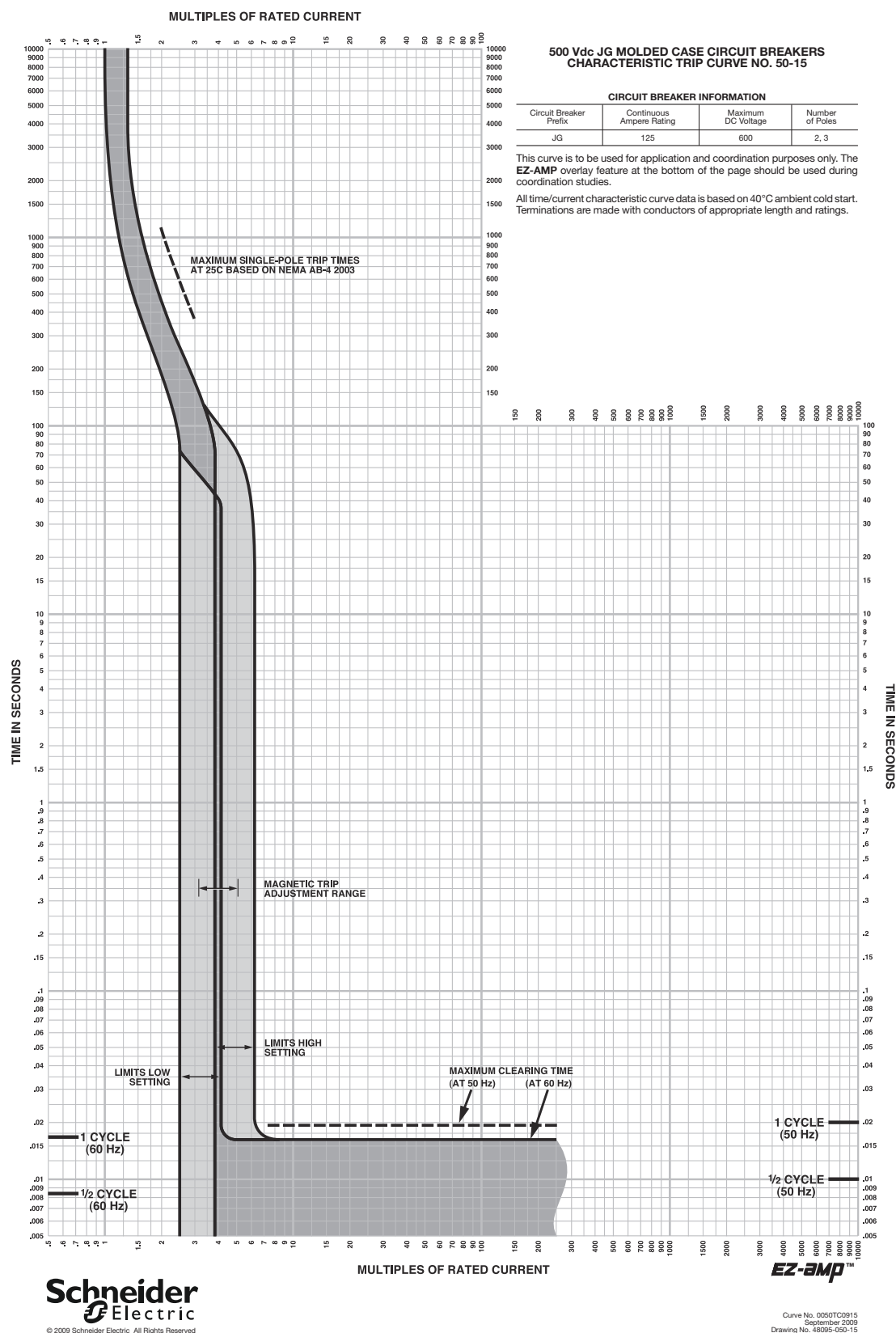
Figure 62: J-Frame 125 A (JG) 500 Vdc Thermal-Magnetic Trip
