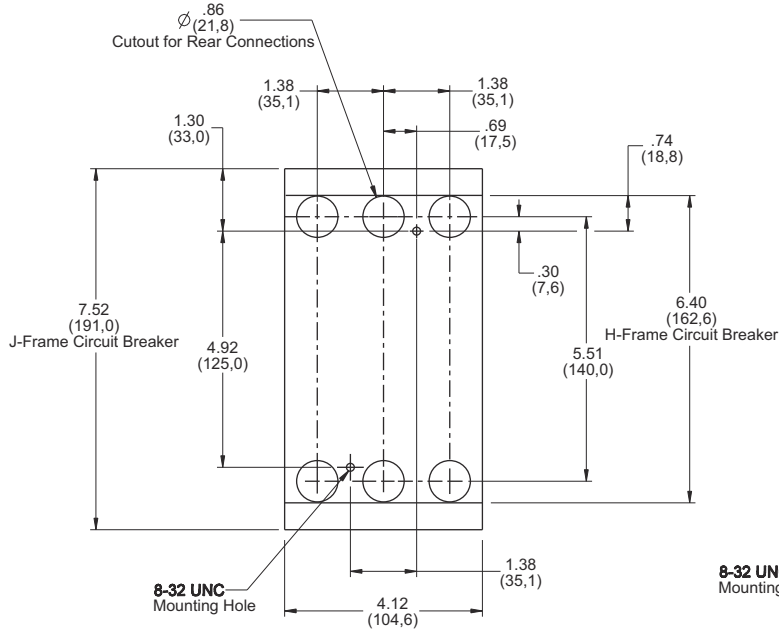
Figure 25: PowerPact H- and J-Frame 3P Circuit Breaker
