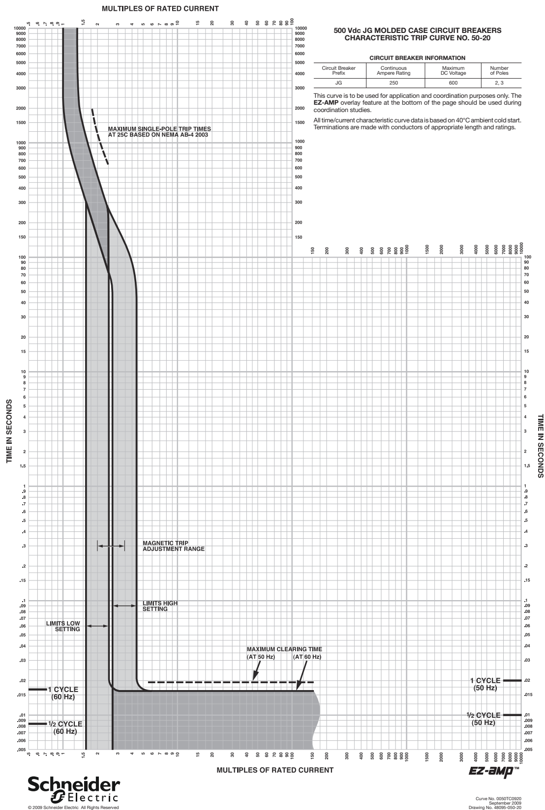
Figure 67: J-Frame 250 A (JG) 500 Vdc Thermal-Magnetic Trip
