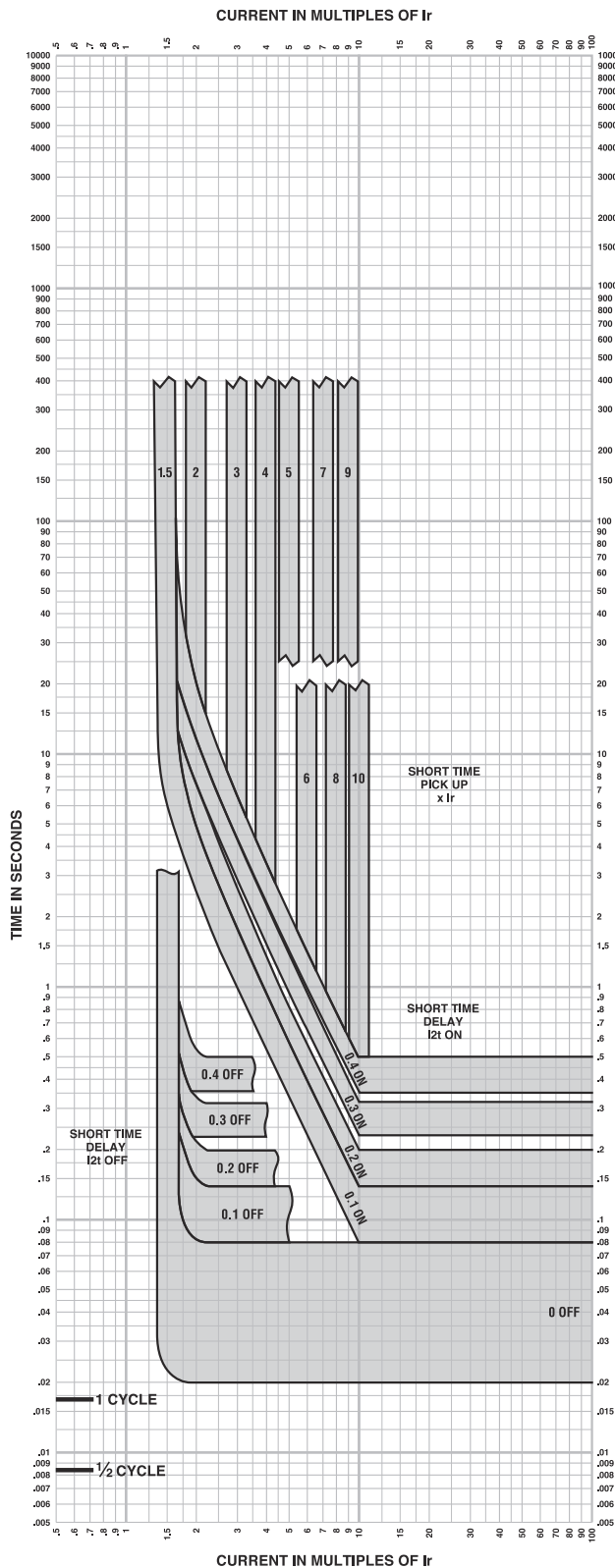
Figure 92: Micrologic 5.2A, 5.2A-W, 5.2E, 5.2E-W, 6.2A, 6.2A-W, 6.2E, and 6.2E-W Electronic Trip Unit Short Time Trip Curve
