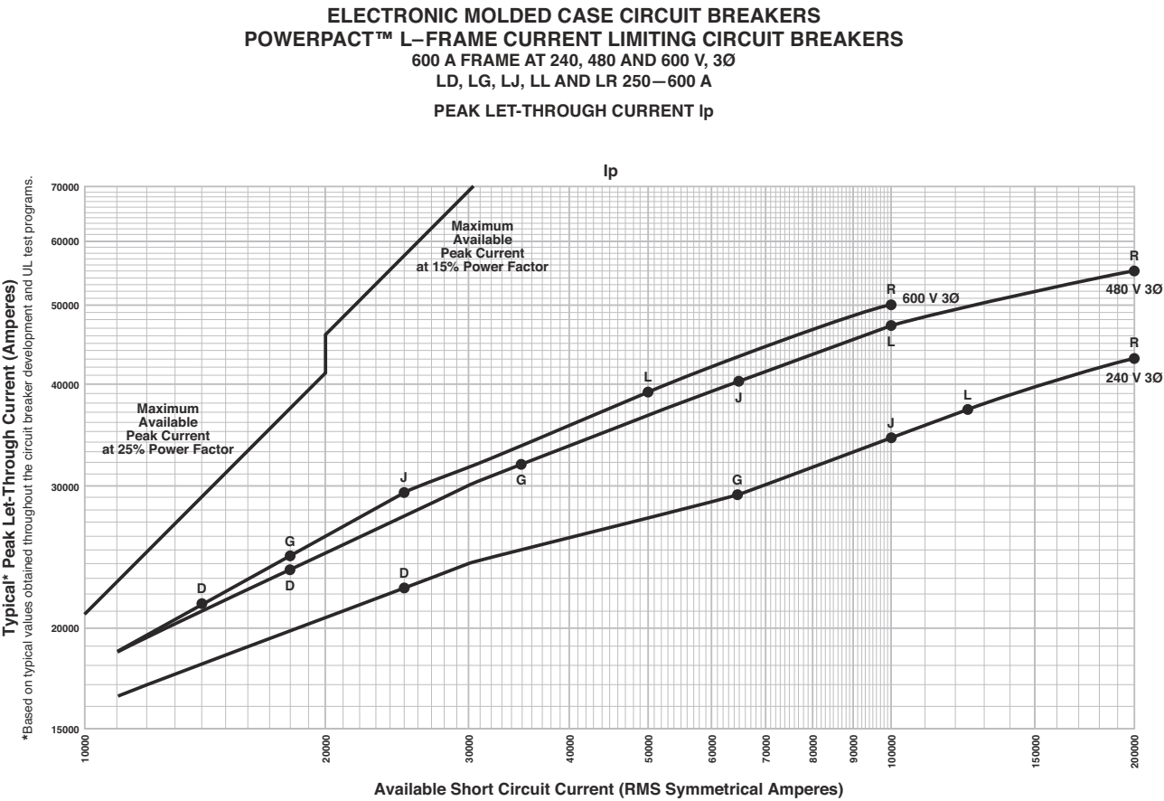
Figure 110: L-Frame 600 A Typical Peak Let-Through Curves
