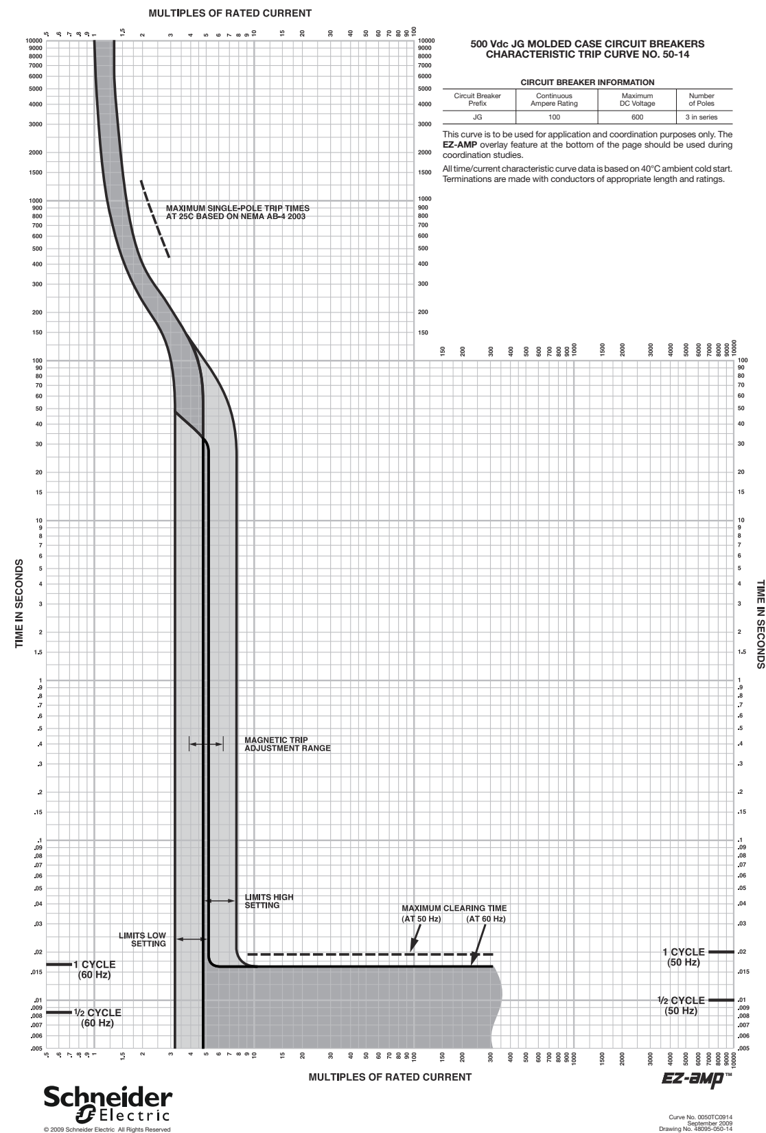
Figure 61: J-Frame 100 A (JG) 500 Vdc Thermal-Magnetic 500 Trip
