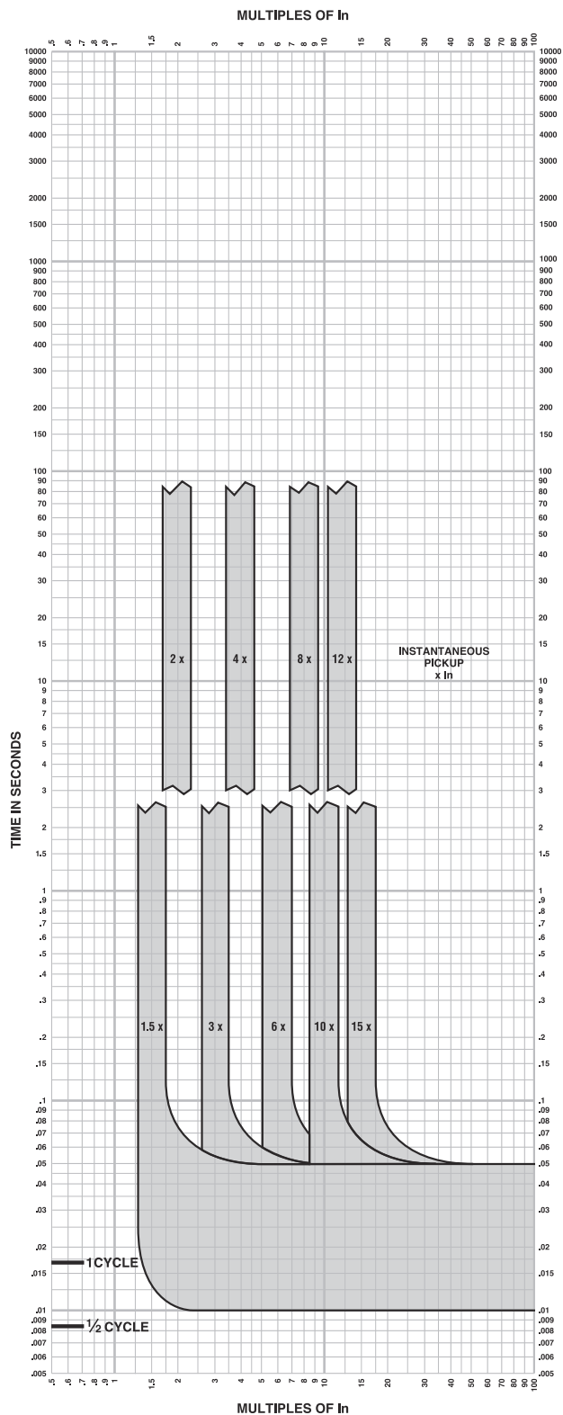
Figure 82: Micrologic 3.2/3.2S/5.2A/5.2E/6.2A/6.2E Electronic Trip Unit Instantaneous Trip Curve
