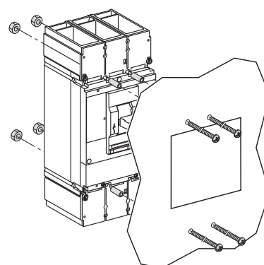
Flush Mounting
