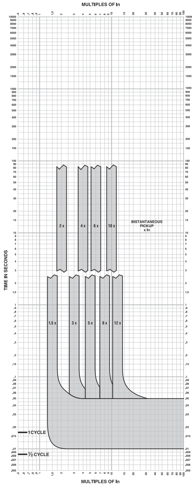
Figure 90: Micrologic 3.2, 3.2-W, 3.2S, 3.2S-W, 5.2A, 5.2A-W, 5.2E, 5.2E-W, 6.2A, 6.2A-W, 6.2E, and 6.2E-W Electronic Trip Curve Instantaneous Trip Curve
