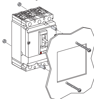
Flush Mounting
