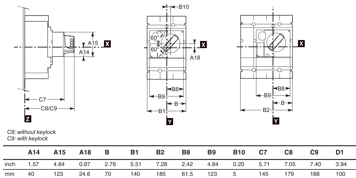
Figure 43: PowerPact L-Frame Circuit Breaker Rotary-Operating Handles
