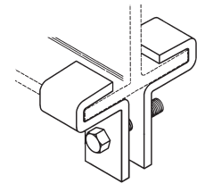
B3050 Beam Clamp Page 13
