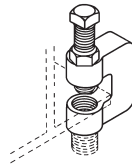
B3036L Malleable Iron C-Clamp With Locknut Page 12
