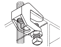
B3031-3/8 Light Duty Malleable C-Clamp Page 11
