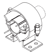
B3281 thru B3287 Pipe Alignment Guide Page 40
