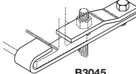
B3045 Side Beam Clamp Page 12
