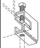
B303 thru B309 Steel Beam Clamp Page 10
