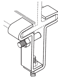
B3055 Steel Beam Clamp Page 13
