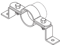
B3148 Offset Pipe Clamp Pages 24 & 25
