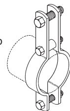
B3144 Double Bolt Pipe Clamp Page 24
