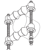
B3122A Adjustable Double Roller Guide Page 22
