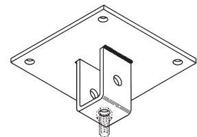
B3085 Rod Attachment Concrete Plate Page 15
