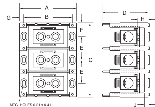
Dimensions - in
