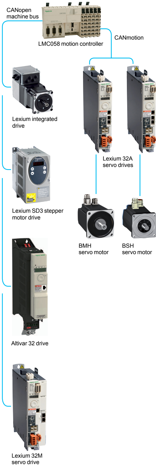
Example of control system architecture with CANopen and CANmotion machine bus
