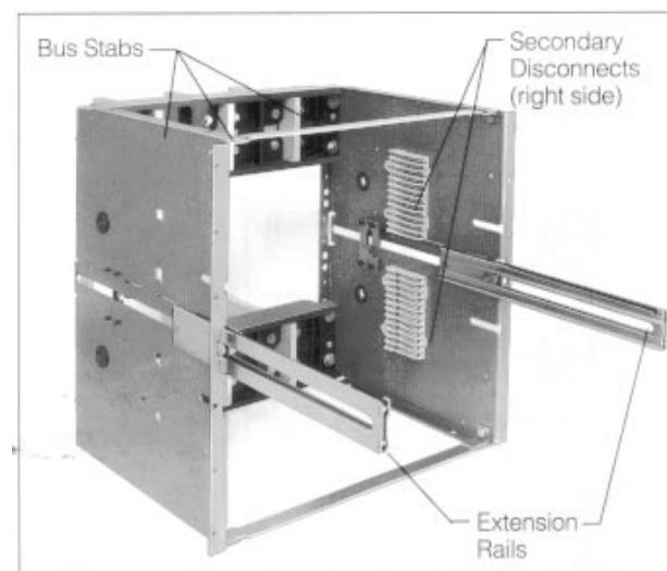
Stationary Drawout Element
