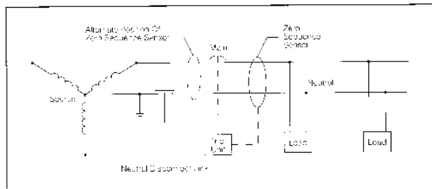
Zero Sequence Ground Fault Protection.
