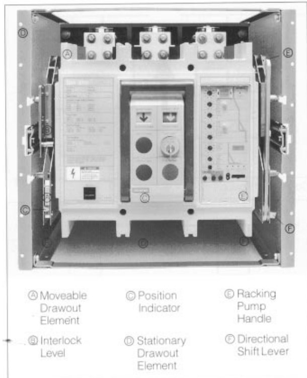
Racking Controls Locations
