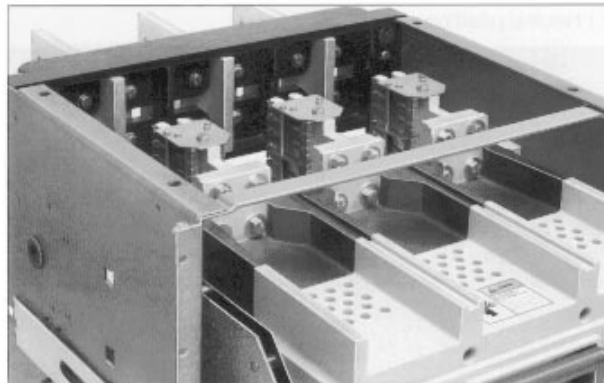
Moveable drawout element in the Withdrawn position
