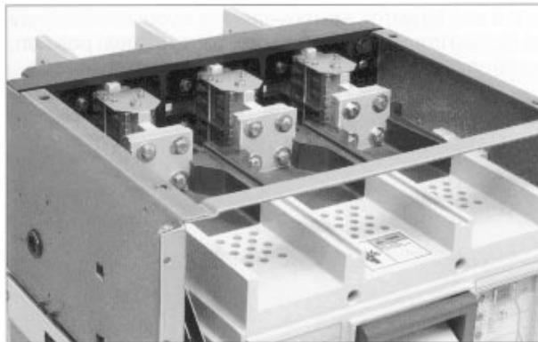
Moveable drawout element in the Connected position
