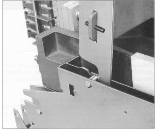
Lift by using rear guide post.
