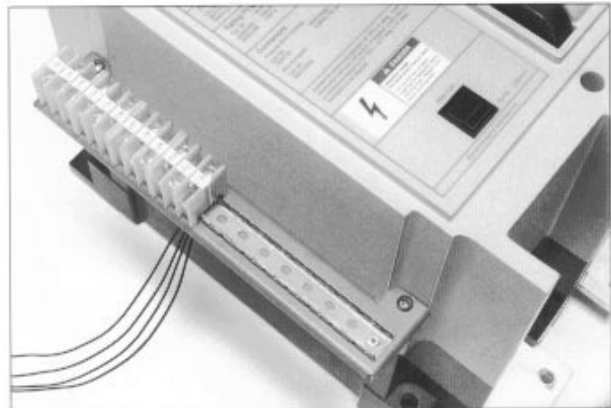
Control Terminal Block mounted on fixed-mounted breaker.
