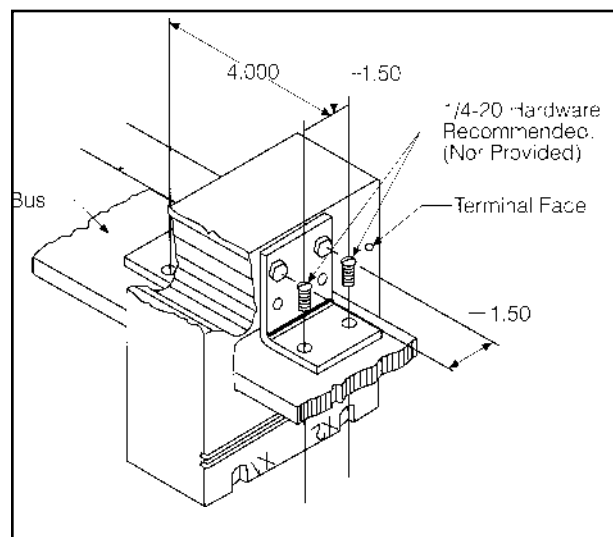
Bus Mounting
