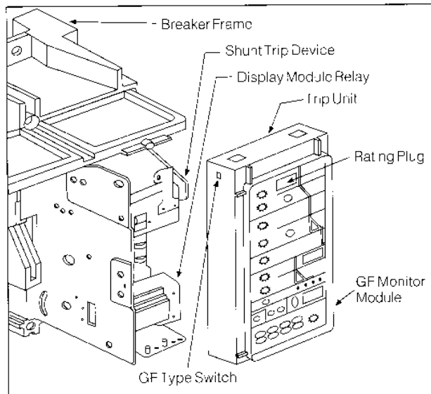
Ground Fault Relaying System
