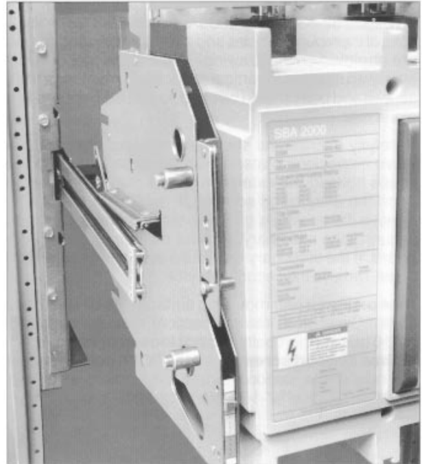
Support Bracket and Guide Rail
