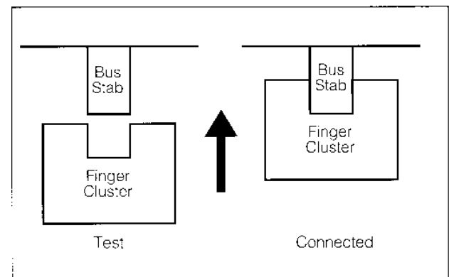
Connected Position
