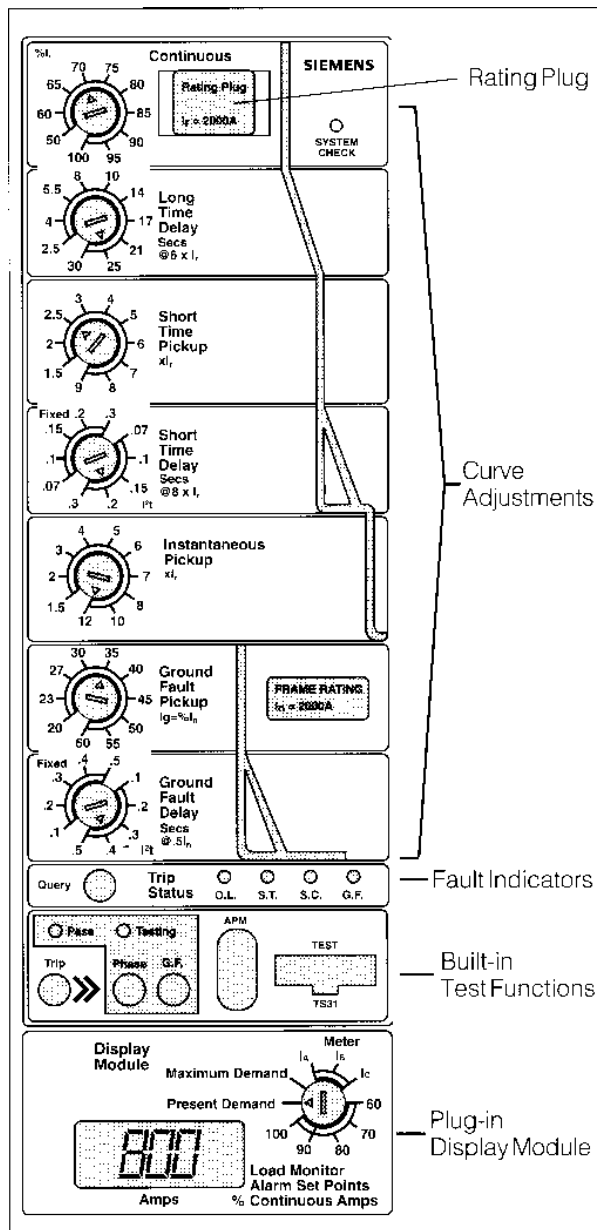
Electronic Trip Unit Adjustment Panel (2000A illustrated)
