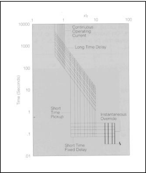
Instantaneous Override (Illustrated with Short Time Fixed Delay)
