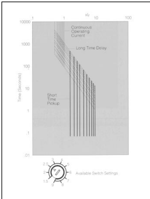
Short Time Pickup
