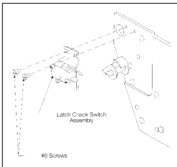
Figure 2. Latch Check Switch Adjustment
