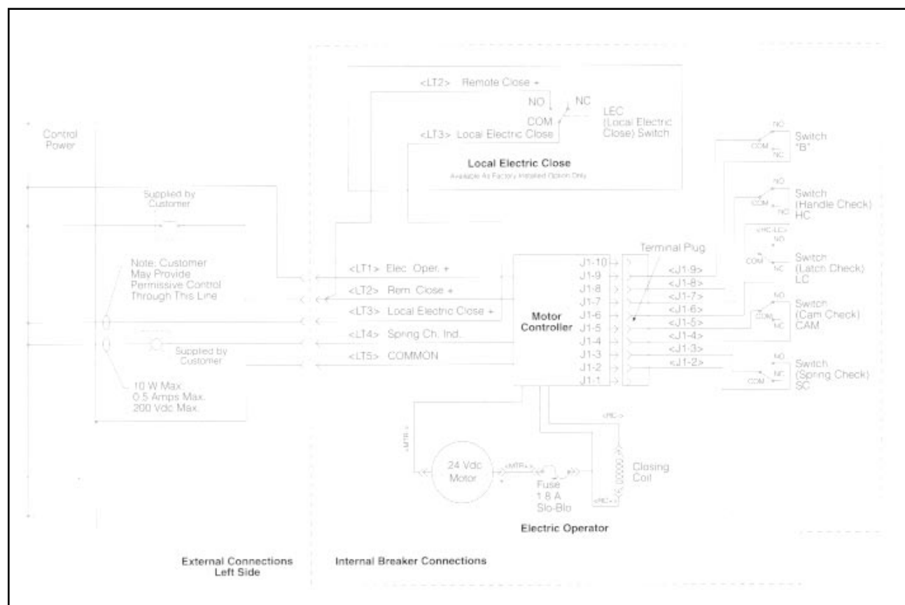
Electric Motor Operator Schematic Diagram
