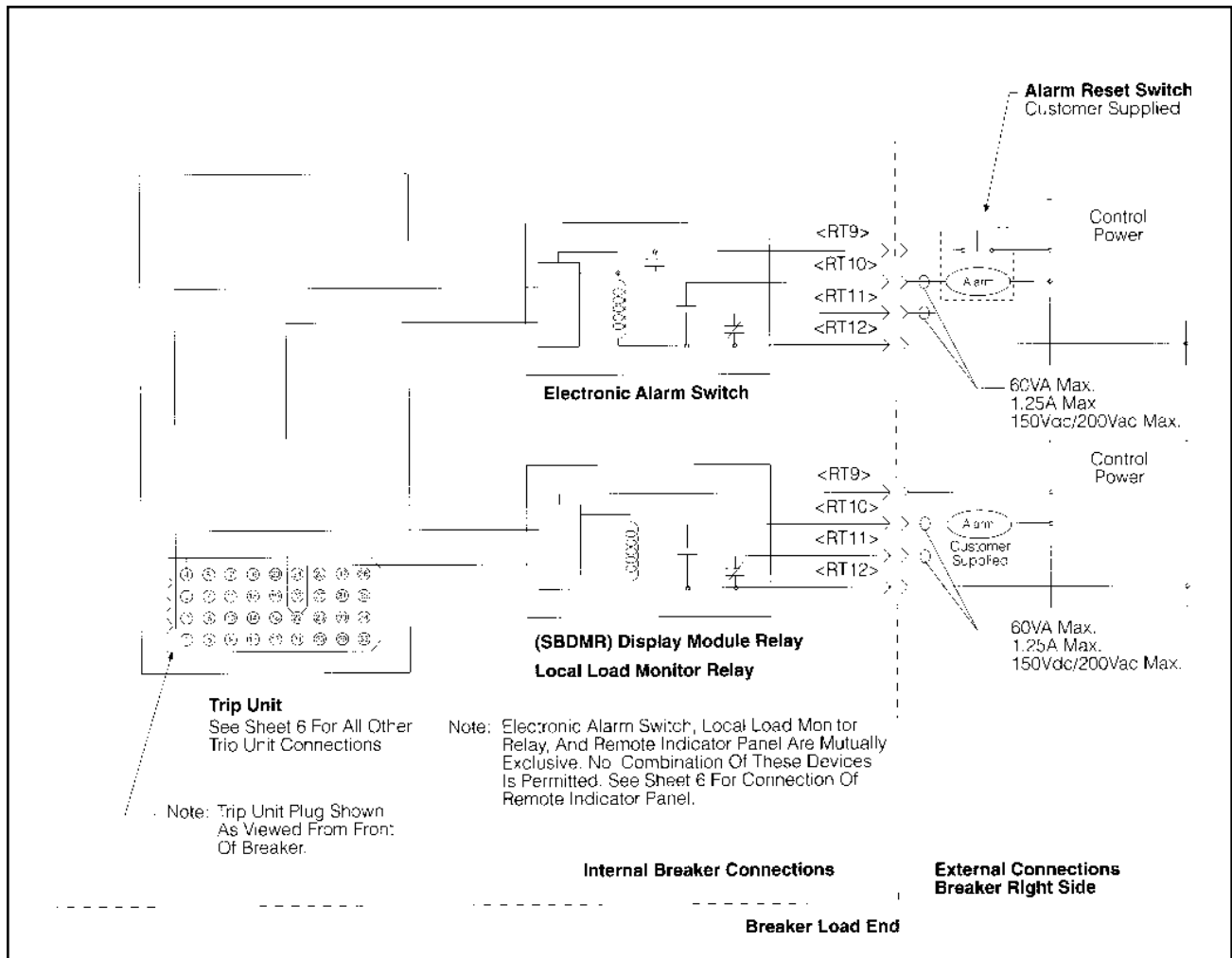
Electronic Bell Alarm or Display Module Relay Schematic Drawing (only 1 device per breaker)
