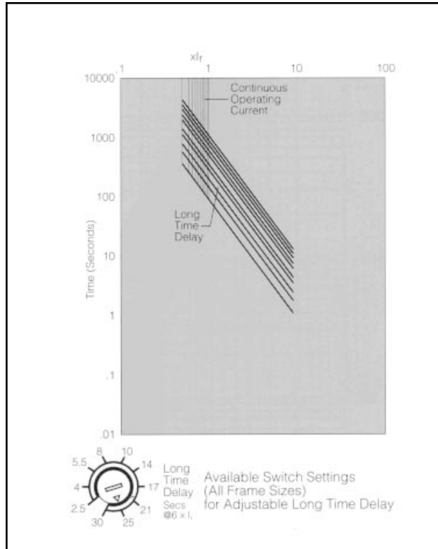
Long Time Delay
