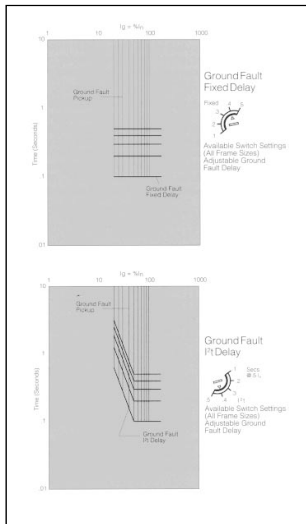
Ground Fault Delay
