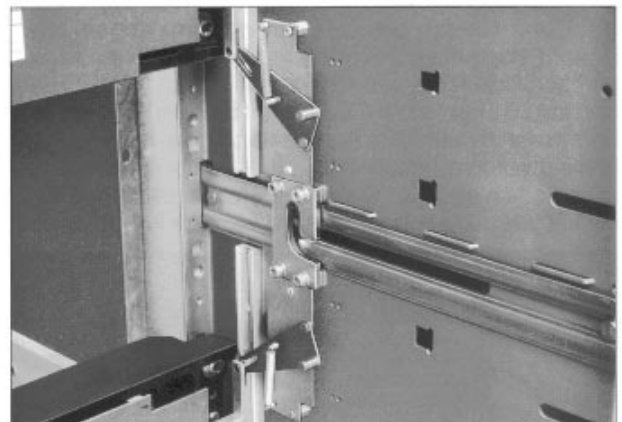
8.) Drawout Safety Shutters shown installed.
