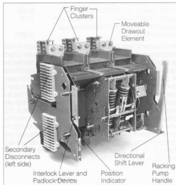
Moveable Drawout Element
