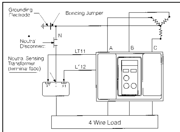
Standard Connection
