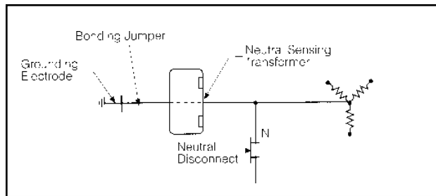
Installation of neutral transformer
