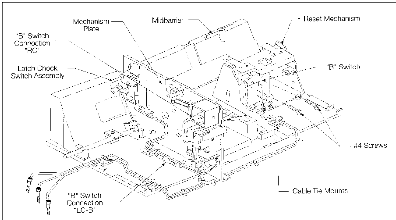
Figure 5. Mounting Of Remote Close Accessory and Wire Routing
