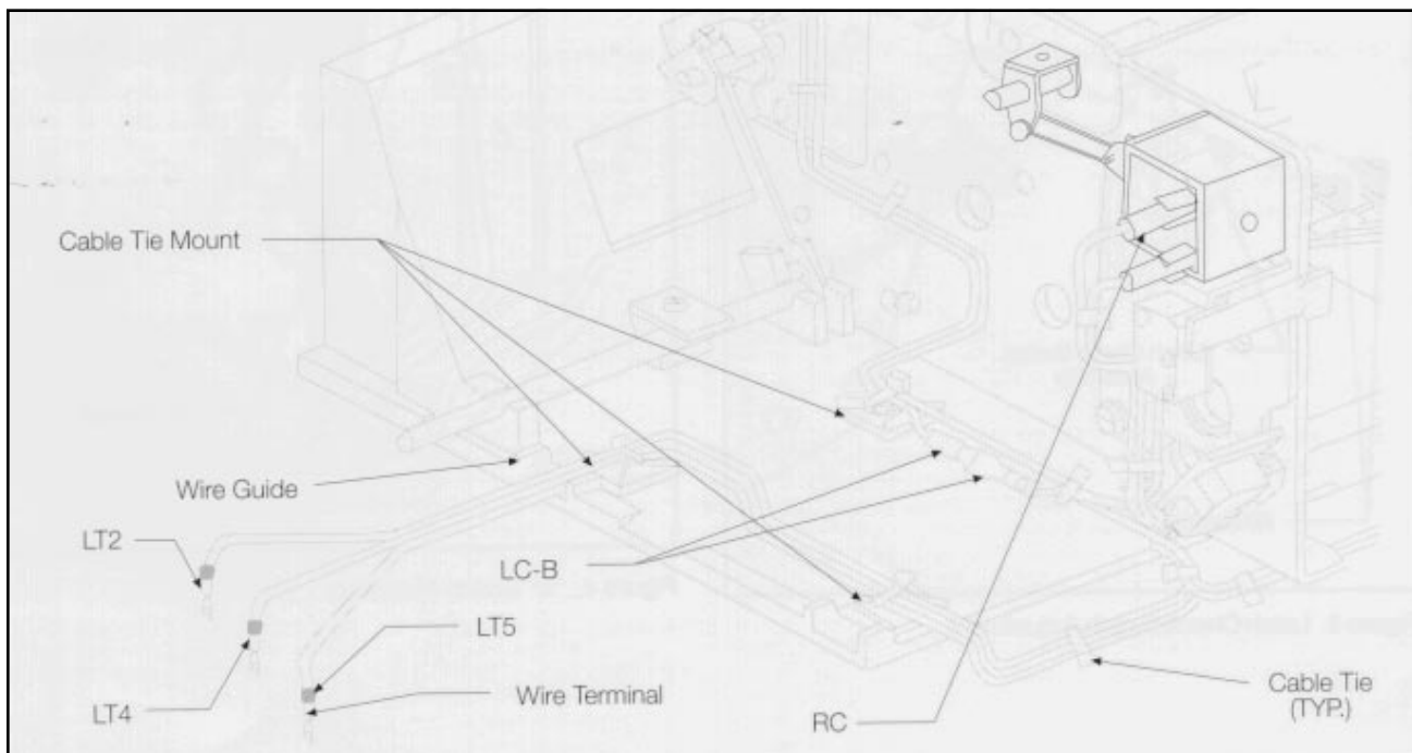
Figure 6. Wire Routing Assembly-Left Side
