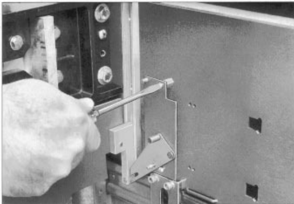
5.) Install top shutter section with #6-32 x 1/4" screws and lock washers, to the sides of the stationary drawout element.
