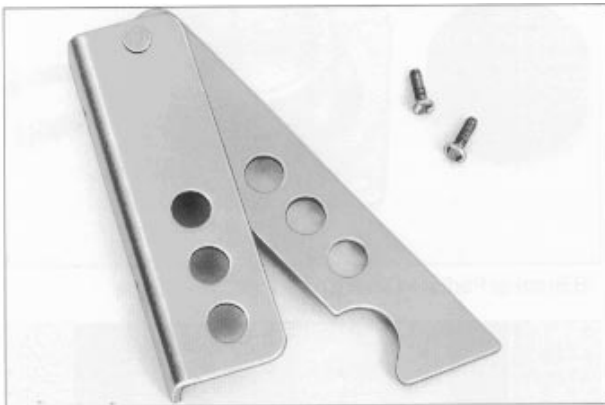
Drawout padlock device kit
