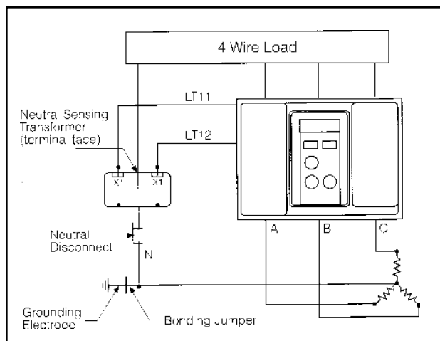
Reverse Connection
