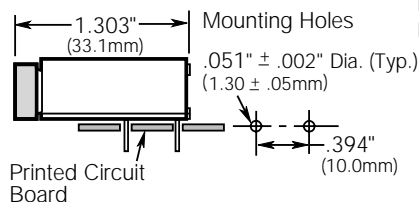
HTC-50M PCB Horizontal Mount 250V, 6.3A, 2.5W Bayonet Cap/Carrier See specifications below
