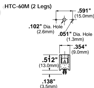
HTC-60M, HTC-65M 250V, 6.3A Body Material: Valox DR48 Terminals: Phosphor bronze
