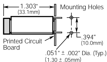
HTC-45M PCB Vertical Mount 250V, 6.3A, 2.5W Bayonet Cap/Carrier See specifications below
