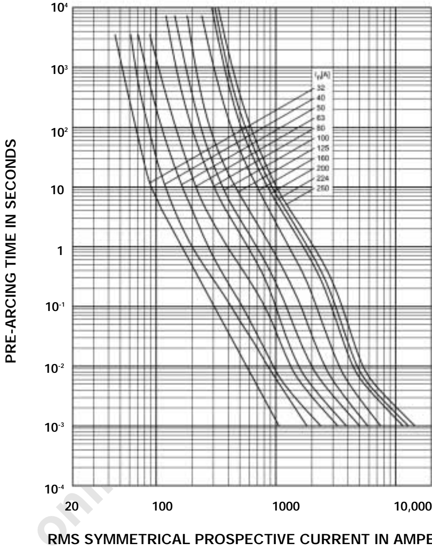
Time Current Characteristics
