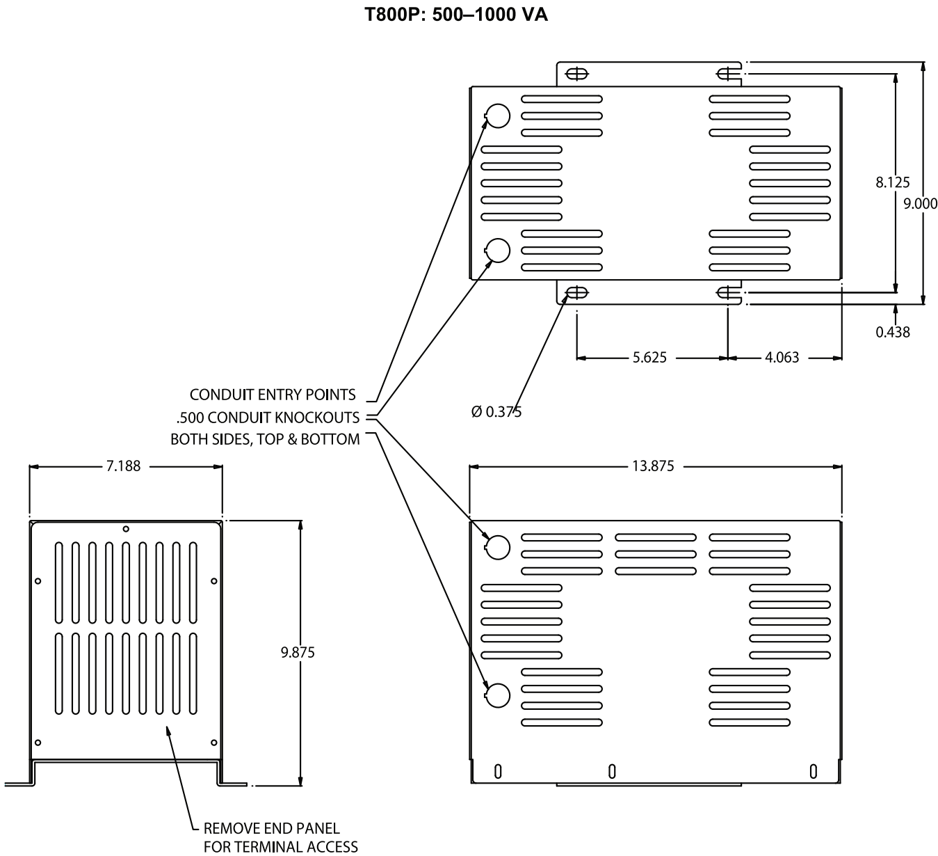
Figure 1-5: Cabinet dimensions T800P wall-/panel-mounted unit, 500–1000 VA
