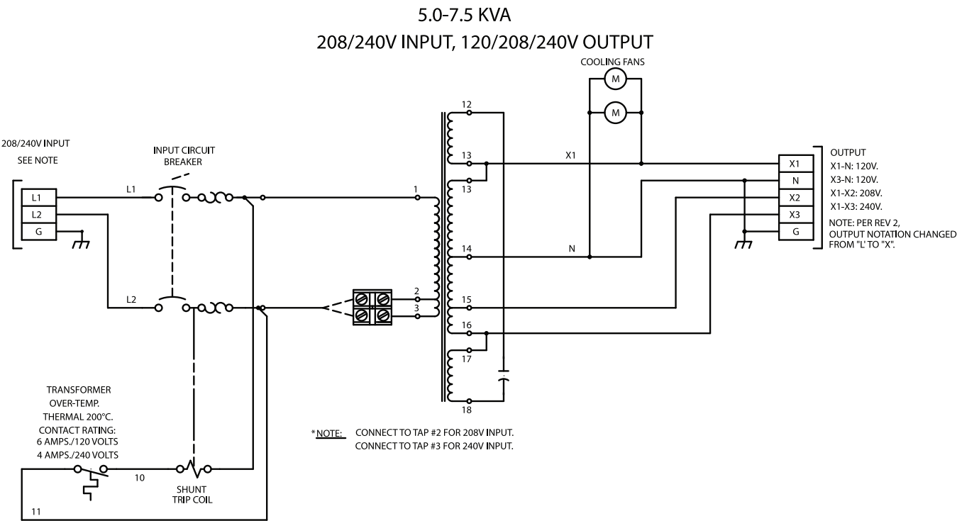
Figure 2-5: Wiring diagram for 5–7.5 kVA T800R (208/240 Vac input and 120/208/240 Vac output, 60 Hz)
