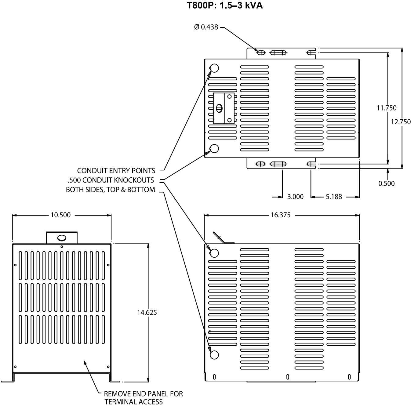
Figure 1-6: Cabinet dimensions T800P wall-/panel-mounted unit, 1500–3000 VA
