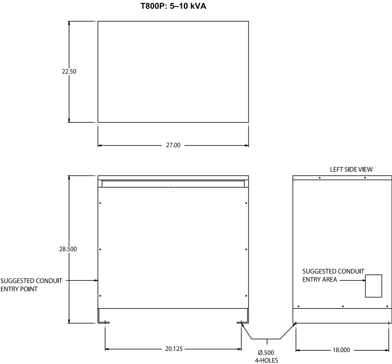
Figure 1-7: Cabinet dimensions T800P wall-/panel-mounted unit, 5000–10,000 VA
