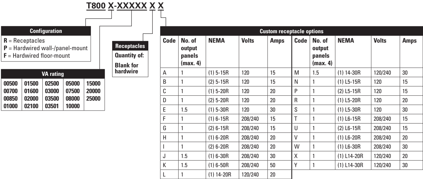
Figure 1-1: T800 product configuration
