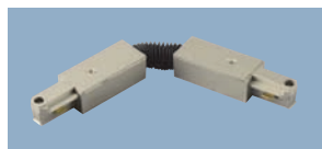
FLEX CONNECTOR P8736-09 Brushed Nickel, P8736-31 Black P9117-28 Bright White Flex connector permits a variety of track layouts at almost any angle and variation of planes including wall-to-ceiling or on cathedral ceilings. Can flex to 90°.
