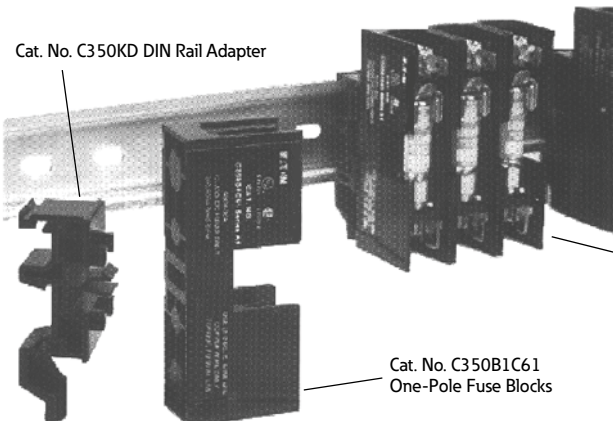
Cat. No. C350BD3C61 Three-Pole with Adapter (Mounted on DIN Rail)
