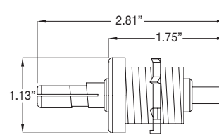
Male receptacle
