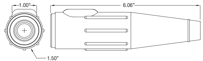
Female plug
