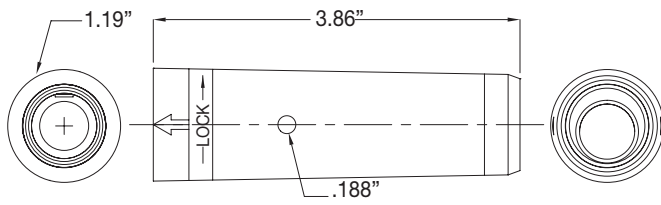
Male & female plug
