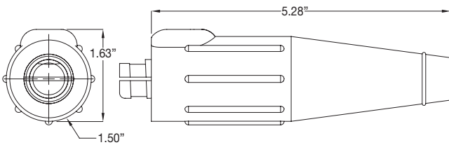
Male plug
