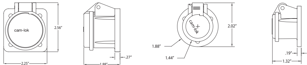
Snap back enclosure assembly
