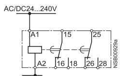
ON-delay
