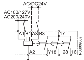
Star delta time relay with overtravel function (idling)
