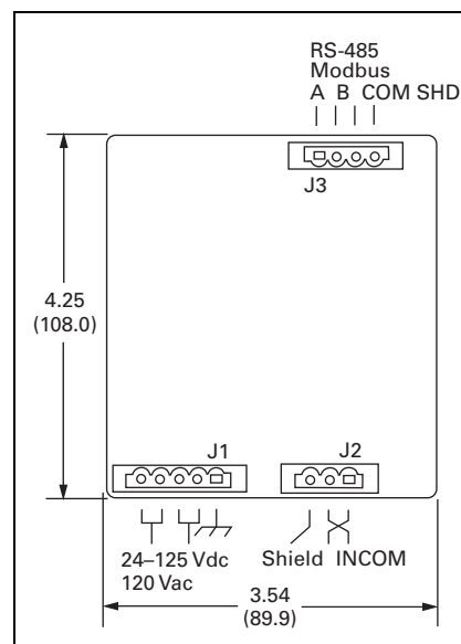
Figure 2.3-3. mMINT Module Dimensions
