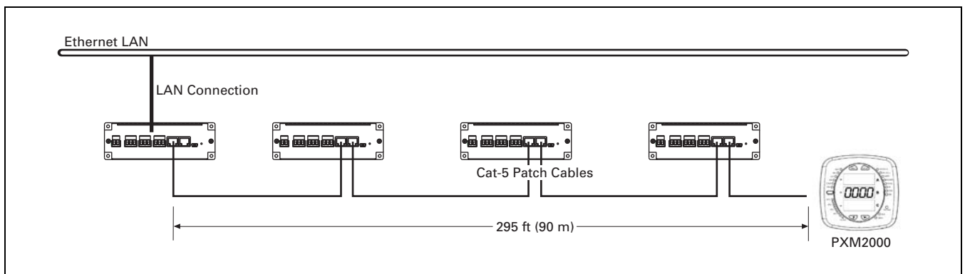
Figure 2.2-6. PXG Daisy Chain Application
