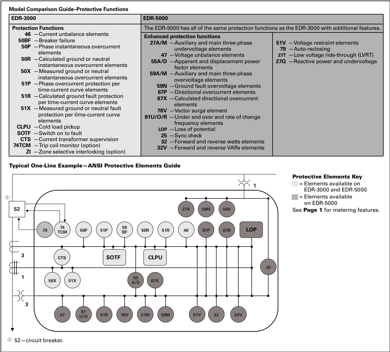
Figure 2.1-2. Protection Feature Comparison
