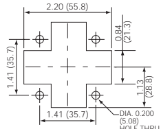
279-PM Recommended Panel Cutout
