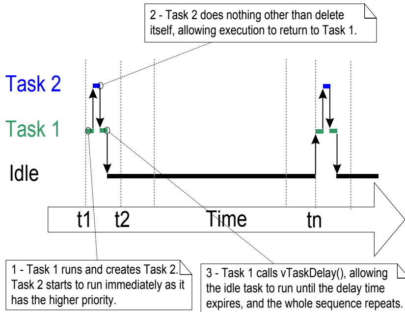
Figure 25. The execution sequence for example 9
