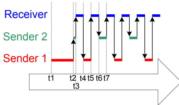
Figure 36. The sequence of execution produced by Example 11
