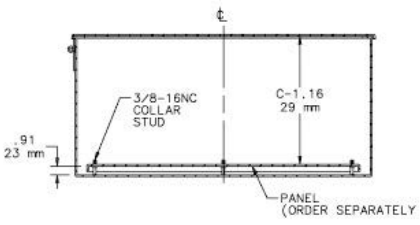
SECTION X-X
