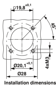
Installation dimensions
