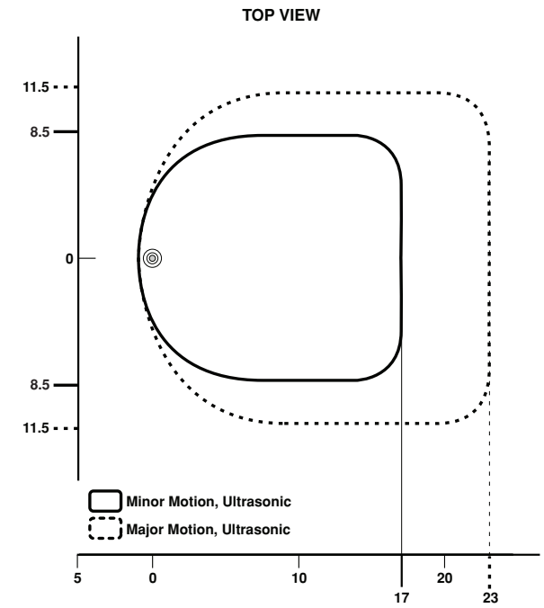
Figure 7 (Cat. No. ODC10) Field-of-View Ranges
