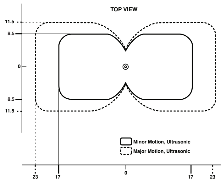
Figure 7 (Cat. No. ODC10) Field-of-View Ranges
