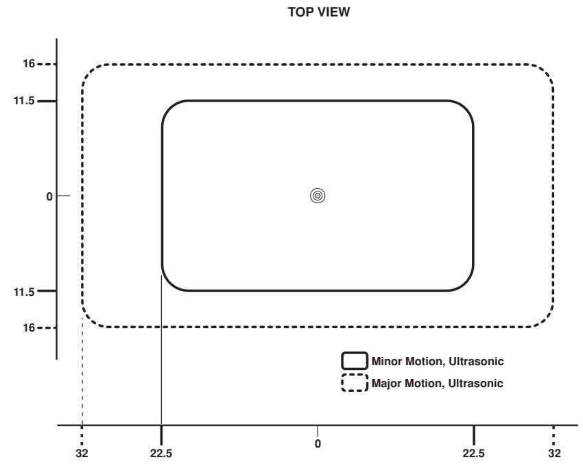
Figure 8 (Cat. No. ODC20) Field-of-View Ranges
