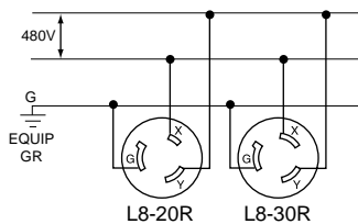
480V AC — 2-POLE, 3-WIRE GROUNDING
