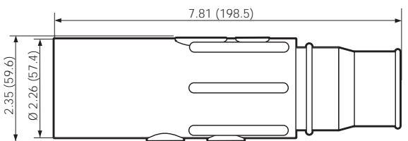
MALE VULCANIZED PLUG—CRIMPED
