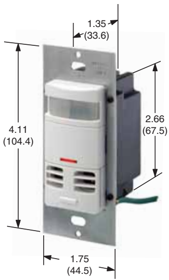
OSSMT-MD Multi-Tech Sensor
