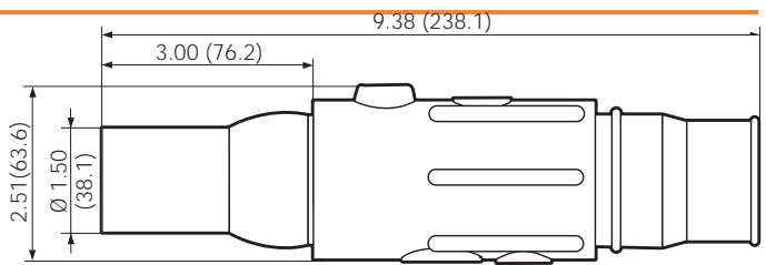
FEMALE DETACHABLE PLUG—DOUBLE SET SCREW
