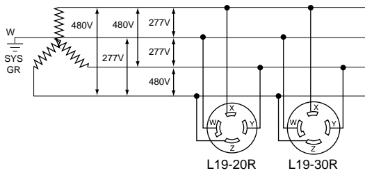
3ØY 277/480V — 4-POLE, 4-WIRE
