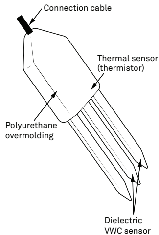
Figure 5 5TM components
