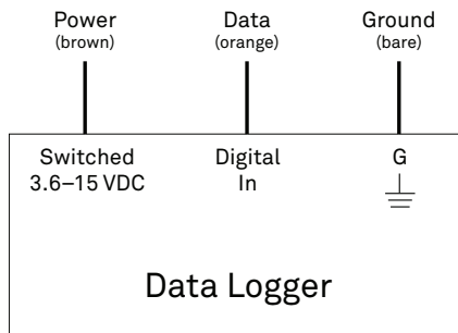
Figure 4 Wiring diagram
