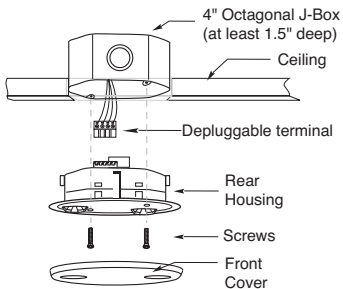
J-Box Mount
