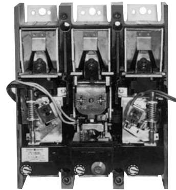
J Frame Circuit Breaker with Internal Accessories Mounted in Each Pole
