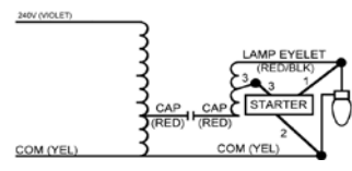
Wiring Diagram 14
