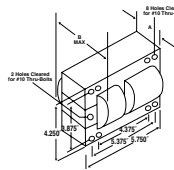
REFERENCE DRAWING PC3
