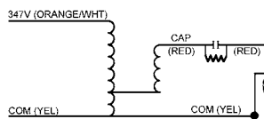
Wiring Diagram 6
