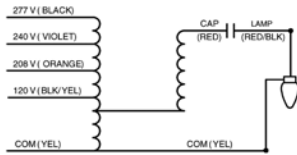
Wiring Diagram 1
