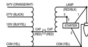
Wiring Diagram 3
