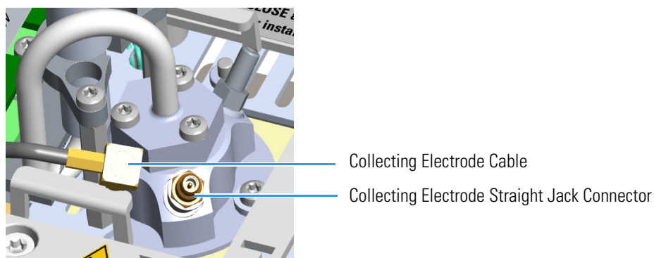
Figure 267. Reinstall Thermionic Source (2)
