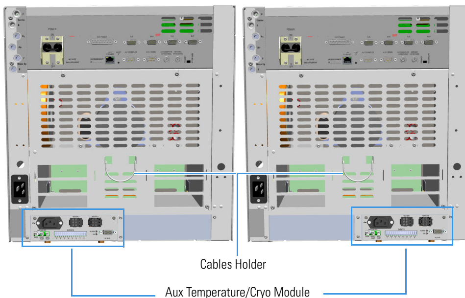
Figure 572. Aux Temperature/Cryo Module Installed into the GC
