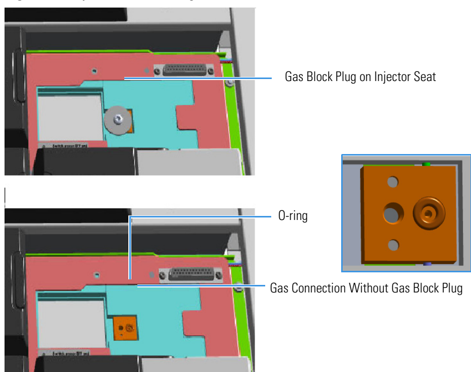
Figure 455. Injector Gas Block Plug
