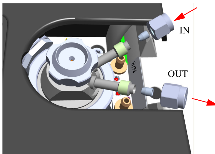
Figure 422. Hot Injection Adapter (5)
