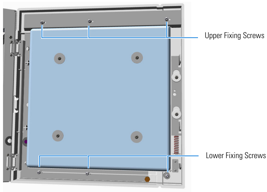
Figure 619. Door Cover Fixing Screws Removal
