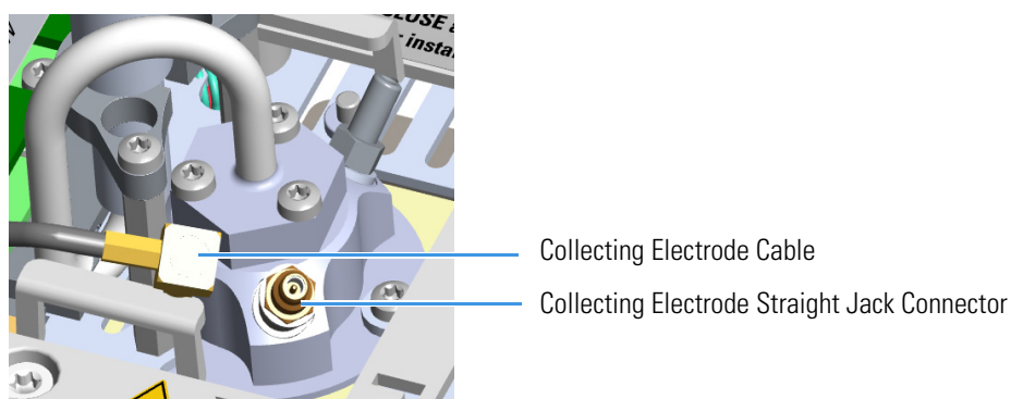
Figure 136. Replace NPD Thermionic Source (2)
