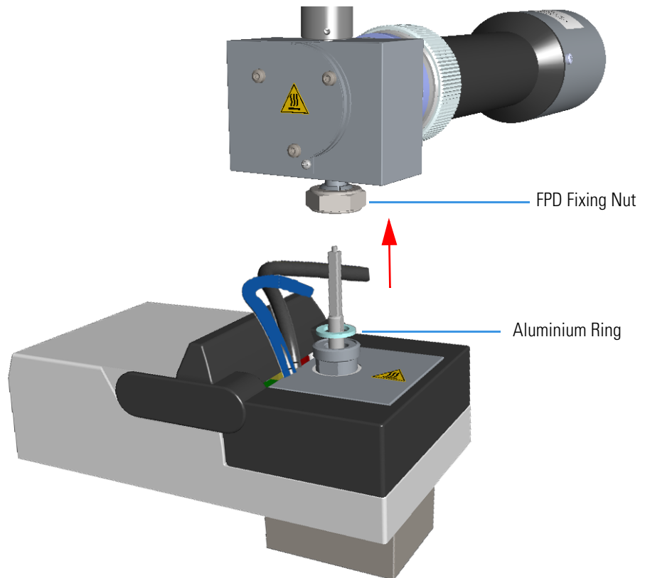
Figure 284. FPD Detector Removal
