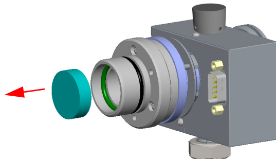
Figure 304. Filter Removal
