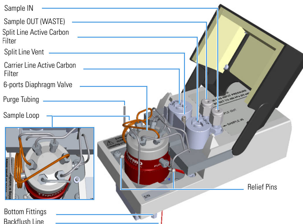
Figure 92. GSV Module Components
