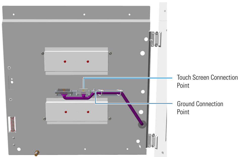
Figure 622. Cables Connections Points
