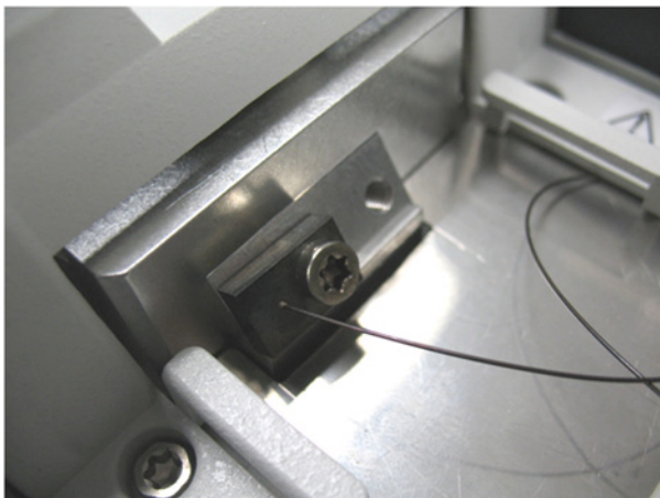
Figure 491. Removing the Helium Tube from the Gas Delivery Block
