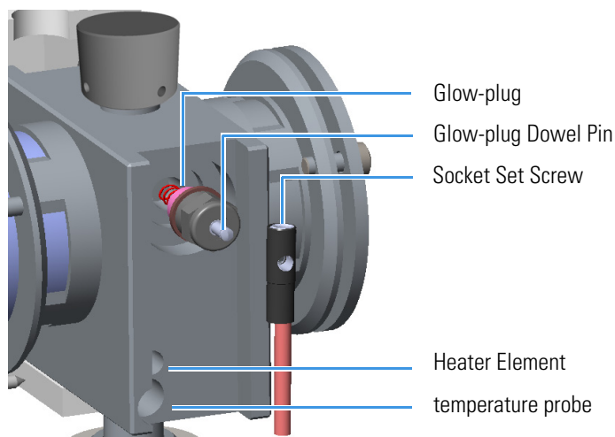
Figure 181. Glow-plug Replacing
