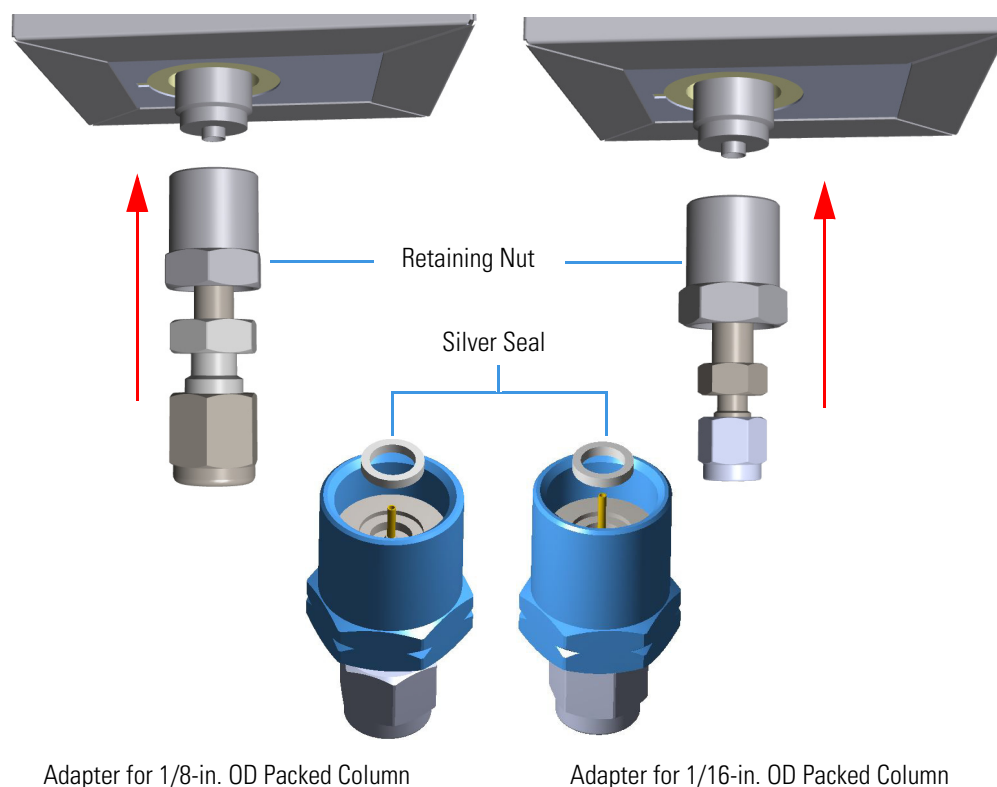
Figure 345. Adapter Installation on the Bottom of the Detector
