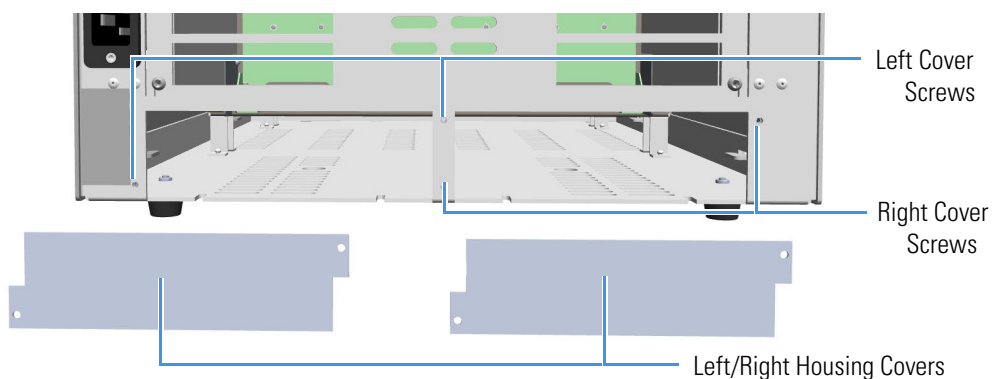
Figure 598. Housing Cover Removal
