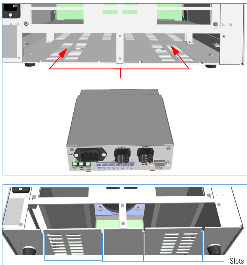
Figure 571. Module Installation (2)
