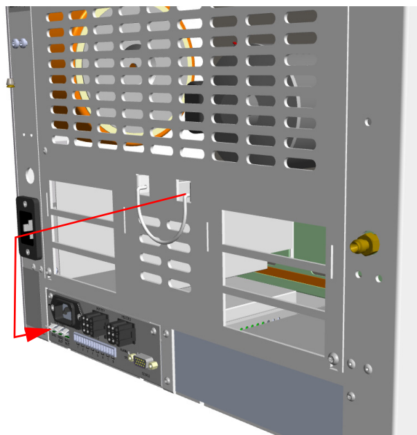
Figure 562. Solenoid Valve Cable Connection
