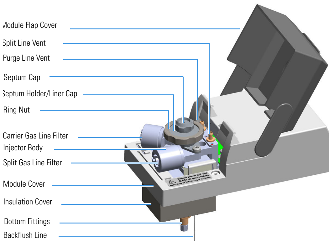
Figure 85. SSLBKF Module Components
