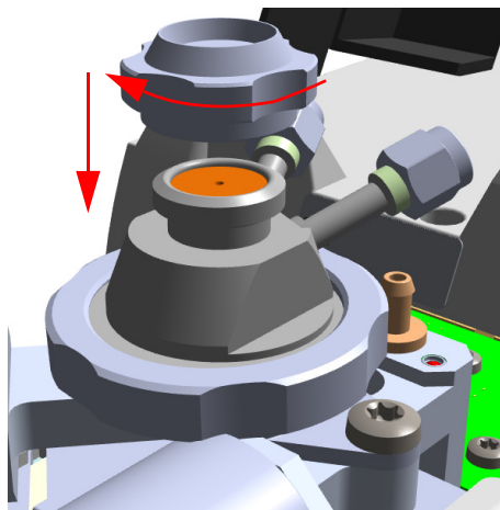
Figure 340. Purge & Trap Adapter (5)
