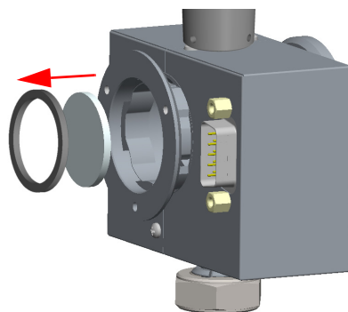
Figure 430. Filter-side Heat Shield Removal
