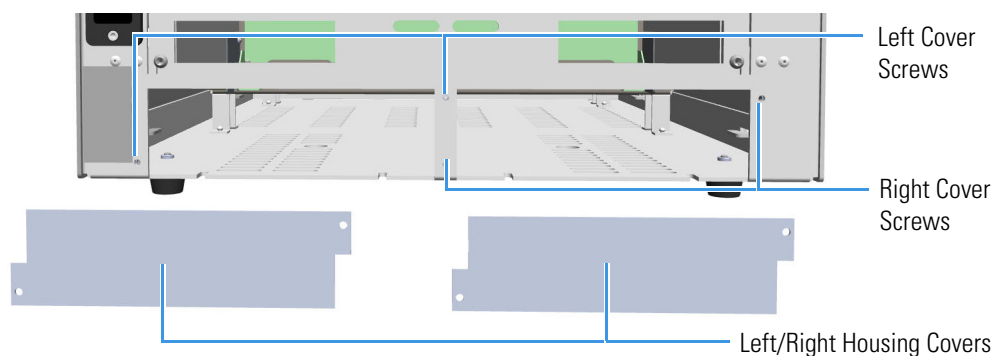
Figure 469. Housing Cover Removal
