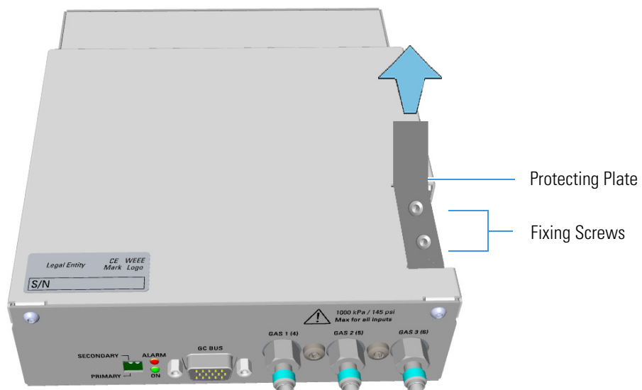
Figure 599. Manifold Protecting Plate
