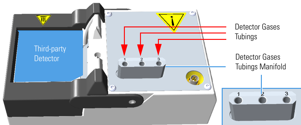
Figure 531. Detector Gas Tubings Connections
