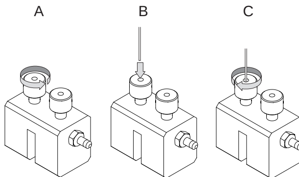
Figure 358. Using a Flowmeter for Leak Check
