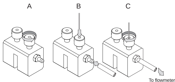
Figure 69. Column Flowmeter Connector
