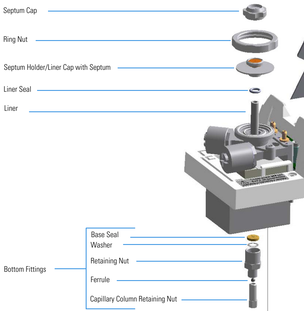
Figure 89. SSLBKF Injector: Broken Liner Replacement
