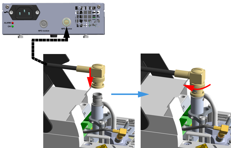
Figure 473. Thermionic Source Assembly Cable Connection
