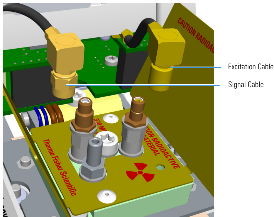
Figure 155. ECD Cables Disconnection
