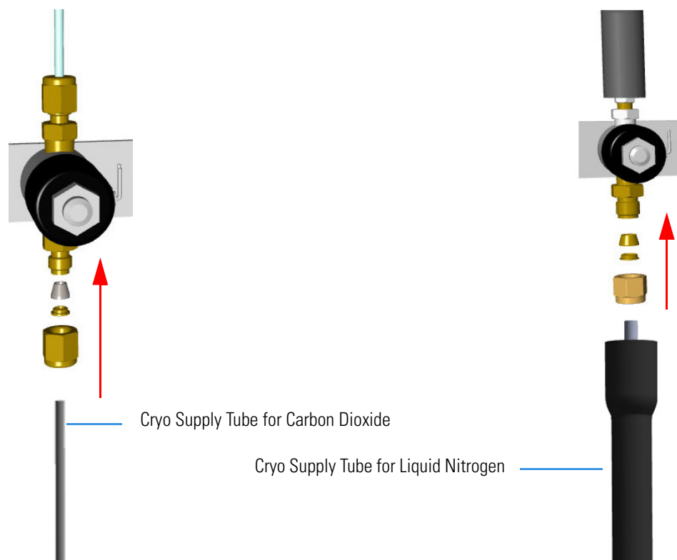
Figure 578. Cryo Supply Tube Connection to the Solenoid Valve
