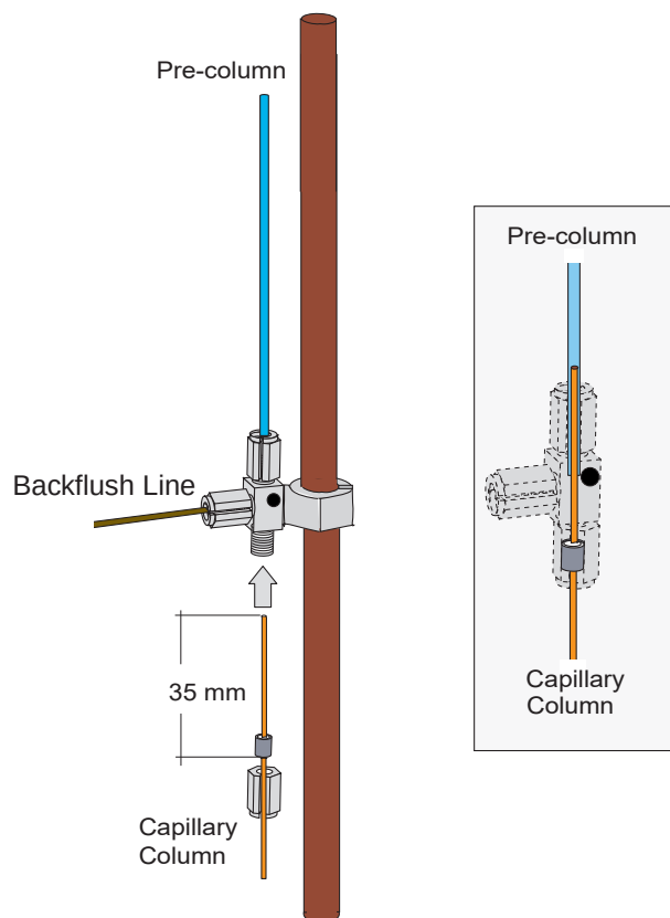
Figure 372. Precolumn and Capillary Column Connection
