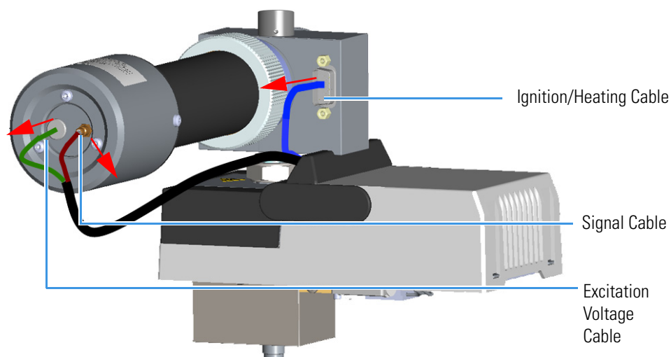
Figure 424. FPD Cable Disconnection
