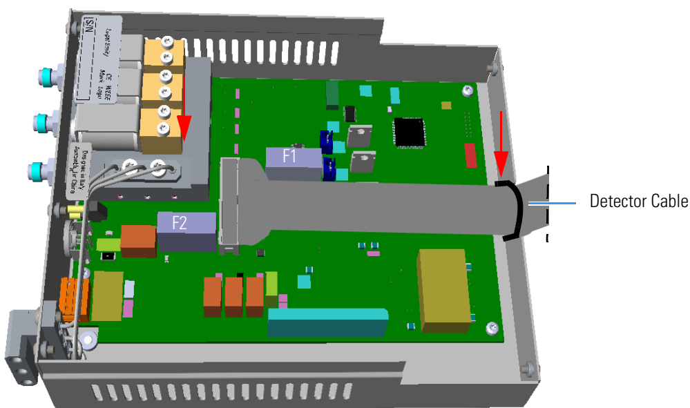
Figure 516. Assemble GDI Electrical Interface (3)
