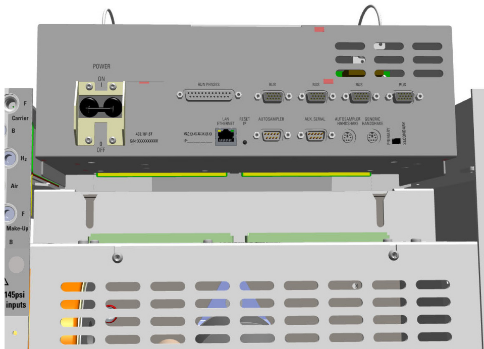
Figure 203. Electronic Module Replacement (2)
