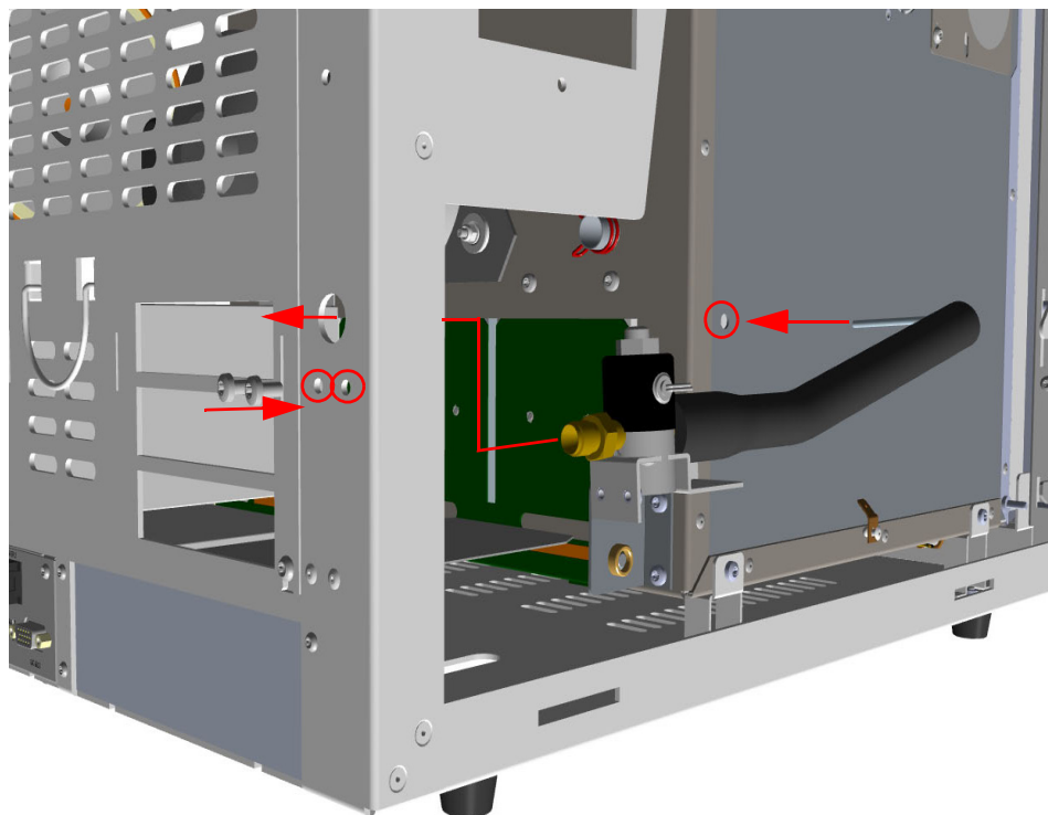
Figure 558. Installation of Solenoid Valve Assembly for Liquid Nitrogen
