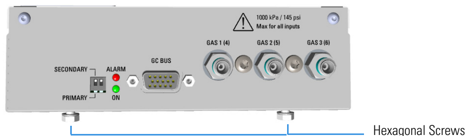
Figure 600. Module Installation (1)
