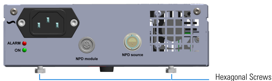
Figure 470. Module Installation (1)
