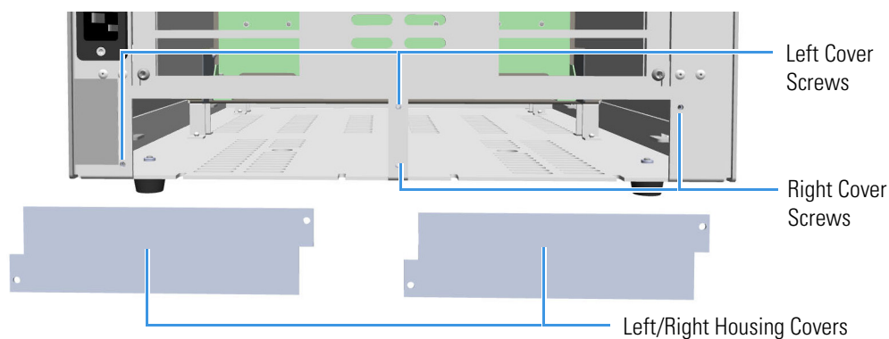
Figure 478. Housing Cover Removal
