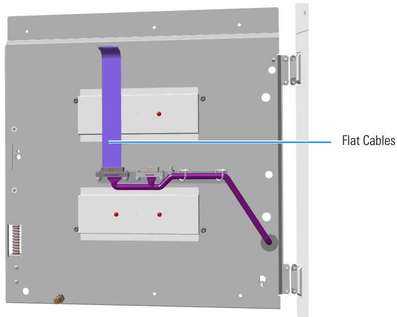
Figure 198. TRACE 1310 Front Door Cables Removal
