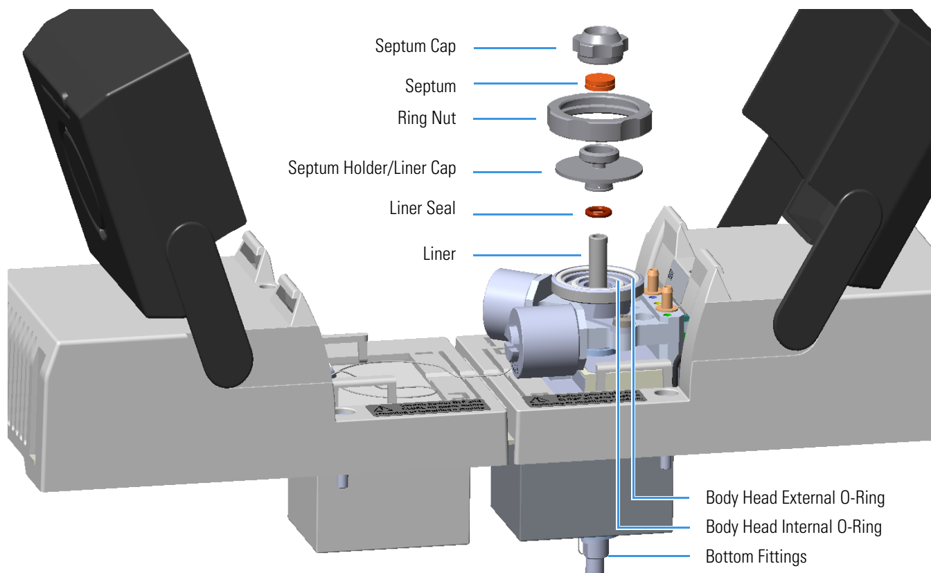
Figure 100. HeS-S/SL Module Components
