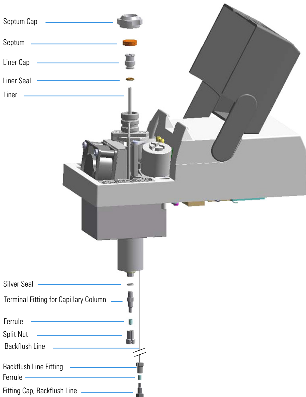
Figure 112. PTVBKF Injector Components
