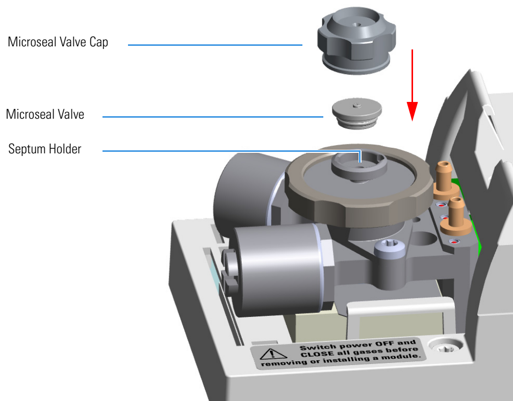
Figure 330. SSL/SSLBKF and HeS-S/SL Injector: Microseal Valve Installation
