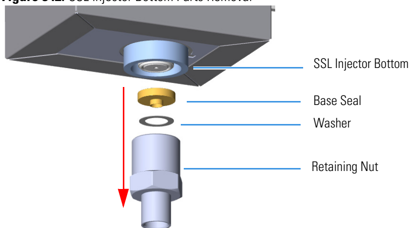
Figure 342. SSL Injector Bottom Parts Removal
