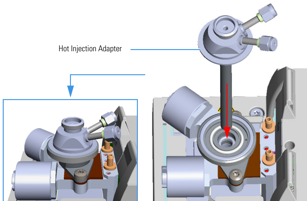
Figure 418. Hot Injection Adapter (1)
