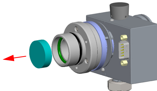
Figure 427. Filter Removal
