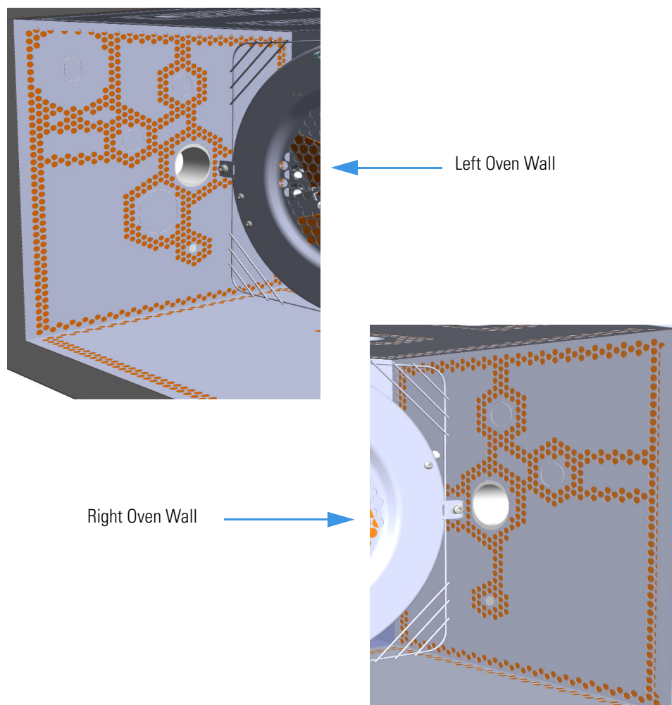
Figure 597. Left/Right Interior Oven Wall Box View
