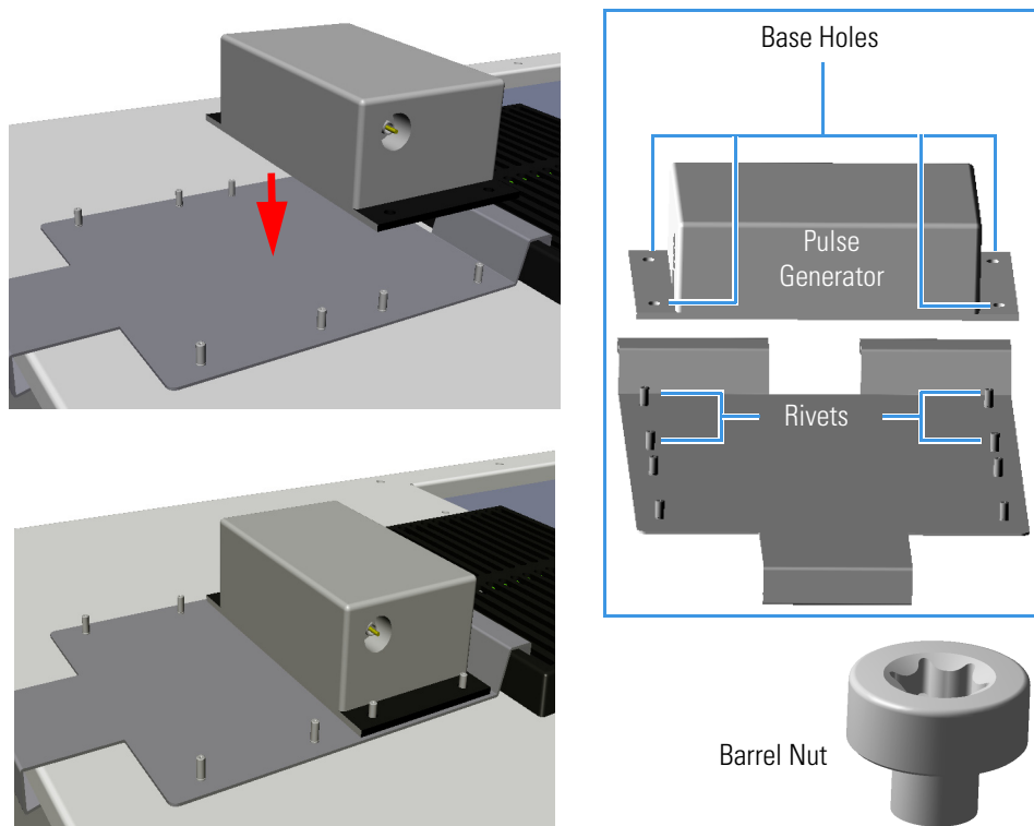
Figure 501. Pulse Generator Installation
