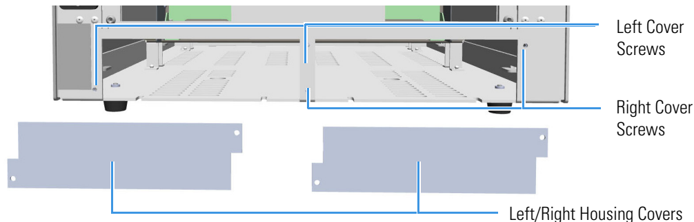
Figure 520. Housing Cover Removal
