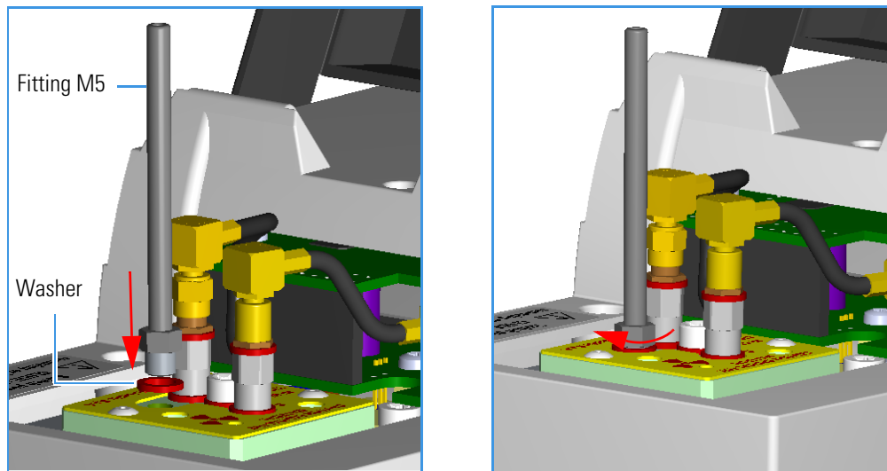
Figure 452. ECD Exhaust Vent Kit Installation (2)
