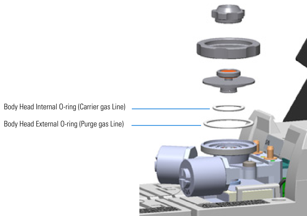
Figure 104. HeS-S/SL Injector: Body Head O-Rings Replacement
