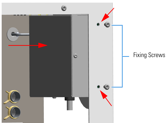
Figure 614. Hydrogen Sensor Installation (2)
