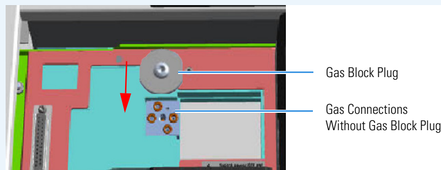
Figure 529. Detector Gas Block Plug (2)
