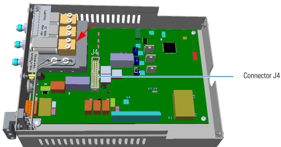
Figure 515. Assemble GDI Electrical Interface (2)
