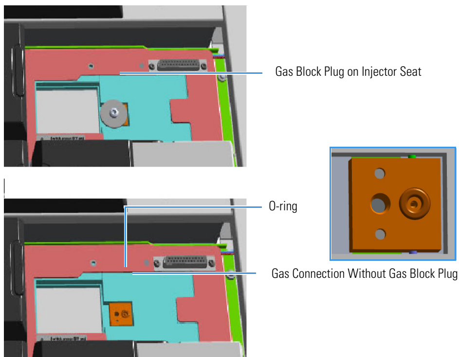
Figure 457. Injector Gas Block Plug
