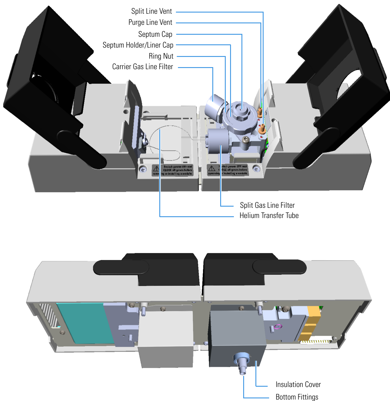
Figure 99. HeS-S/SL Module Components
