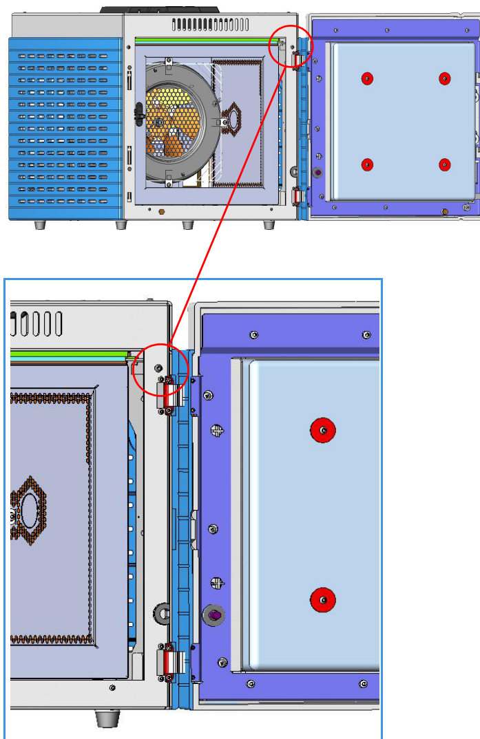
Figure 189. Right Panel Fixing Screw
