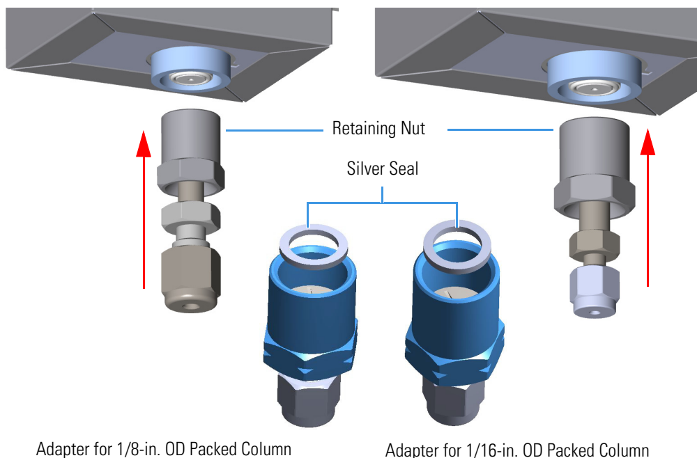
Figure 343. Adapter Installation on SSL Injector Bottom
