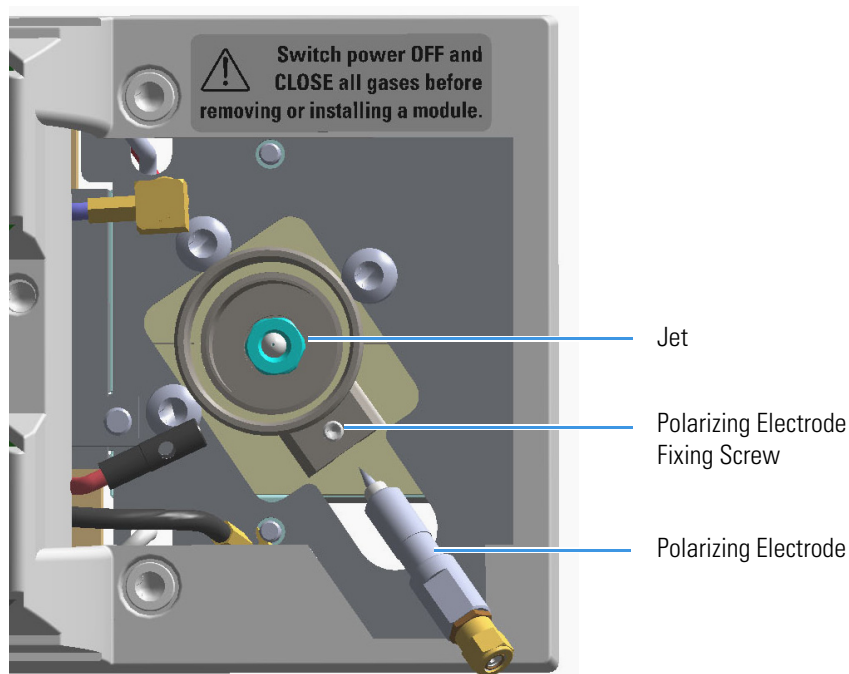
Figure 255. FID Jet (2)
