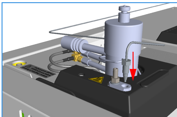
Figure 503. Gas Supply Connections
