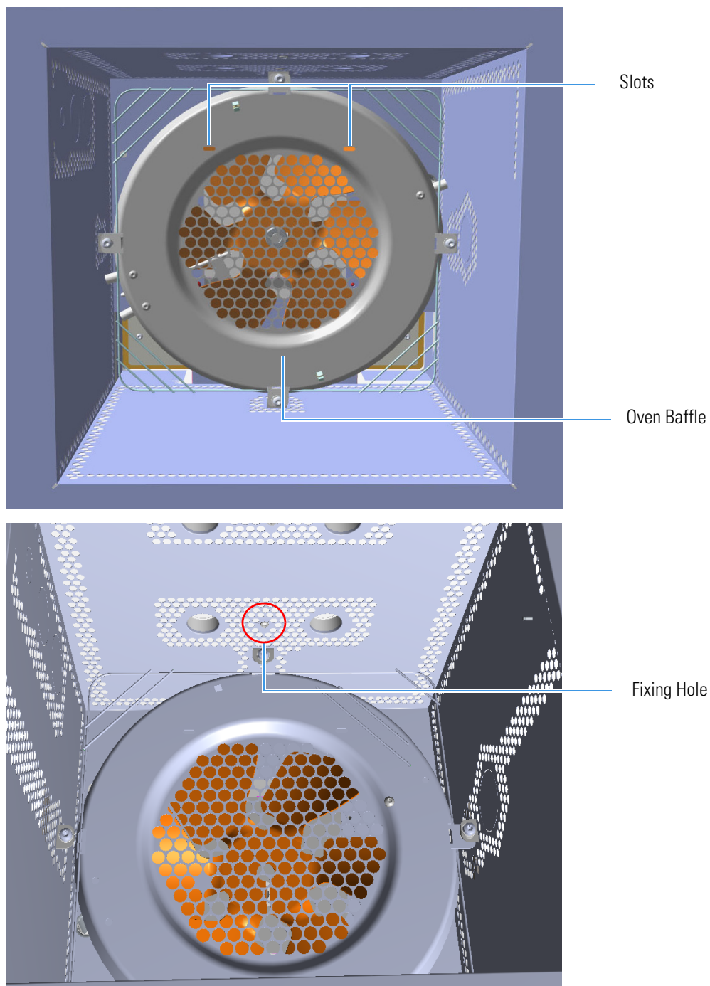
Figure 445. Kit Installation (1)
