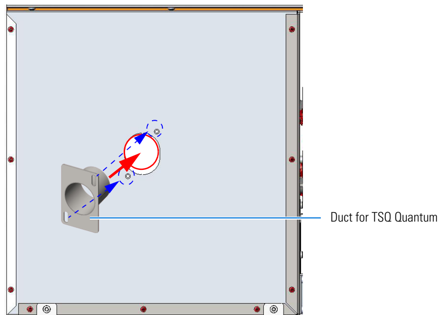
Figure 650. Perform the Duct for TSQ Quantum (2)
