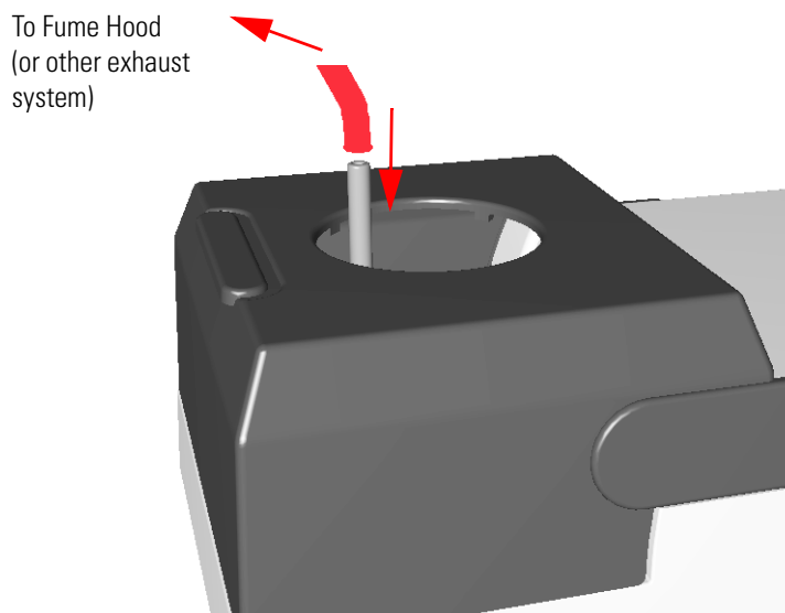
Figure 453. ECD Exhaust Vent Kit Installation (3)
