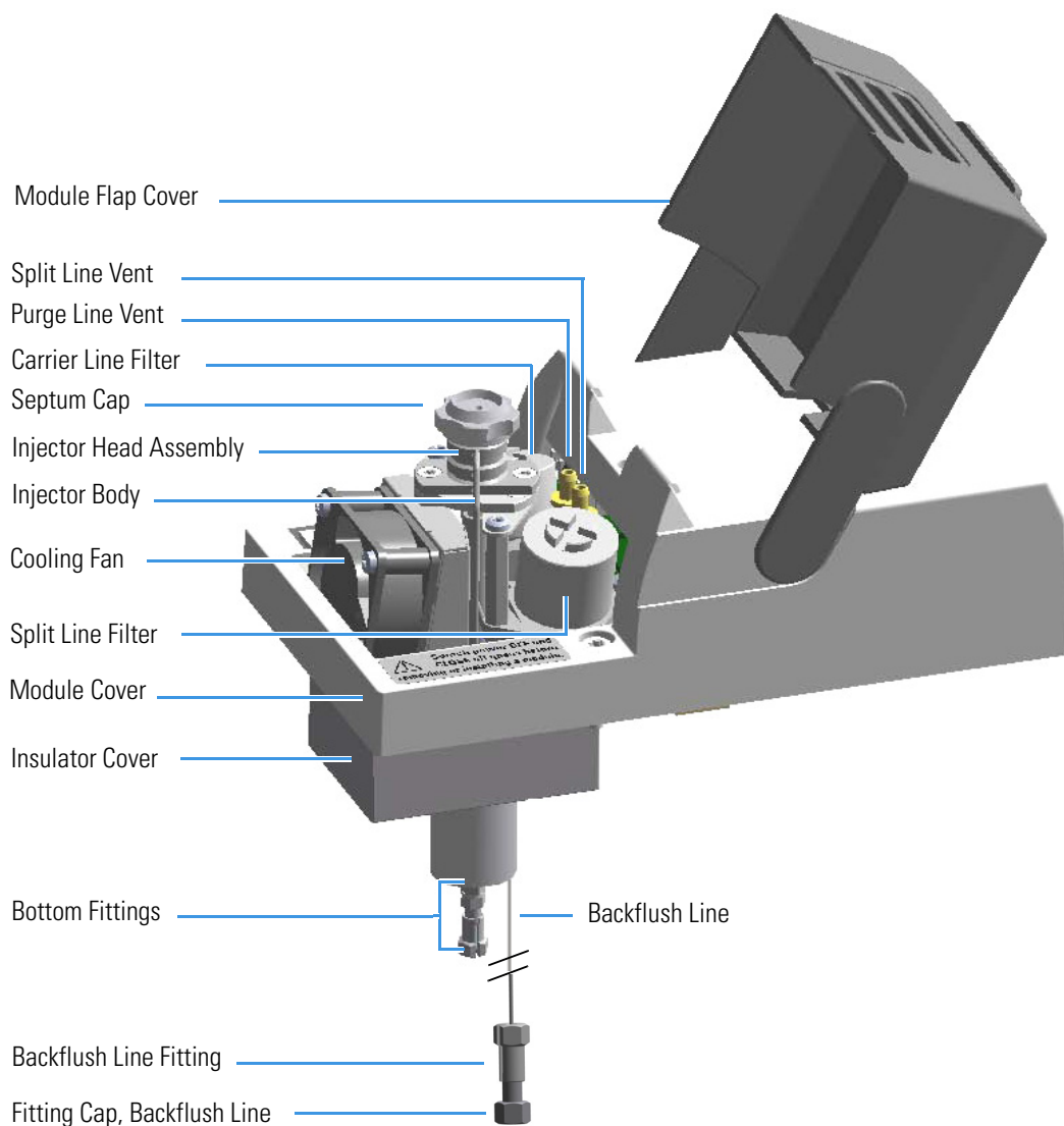
Figure 111. PTVBKF Module Components
