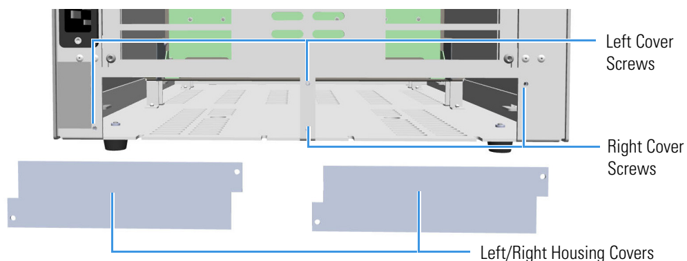
Figure 569. Housing Cover Removal
