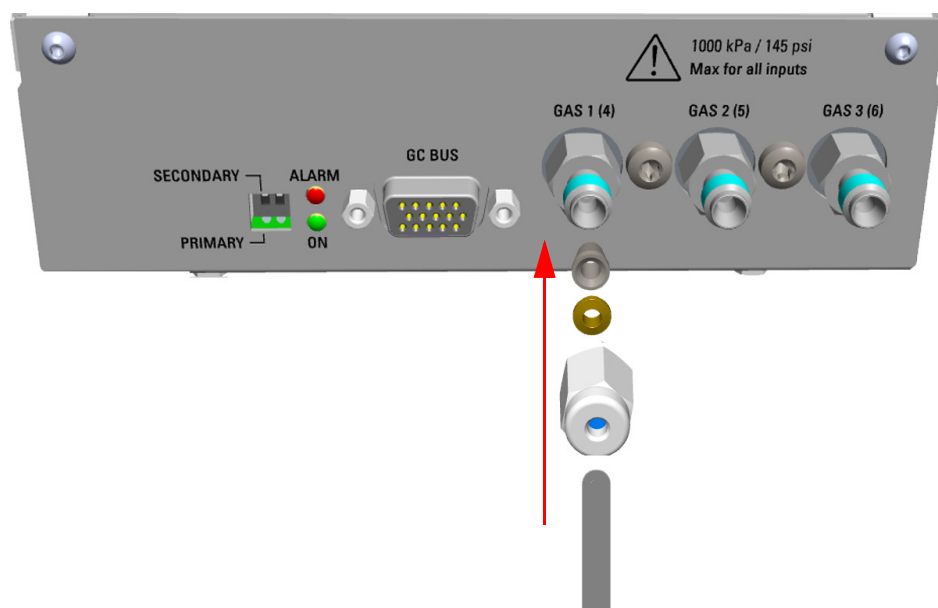
Figure 608. Gas Line Connection to the Auxiliary Gas Interface
