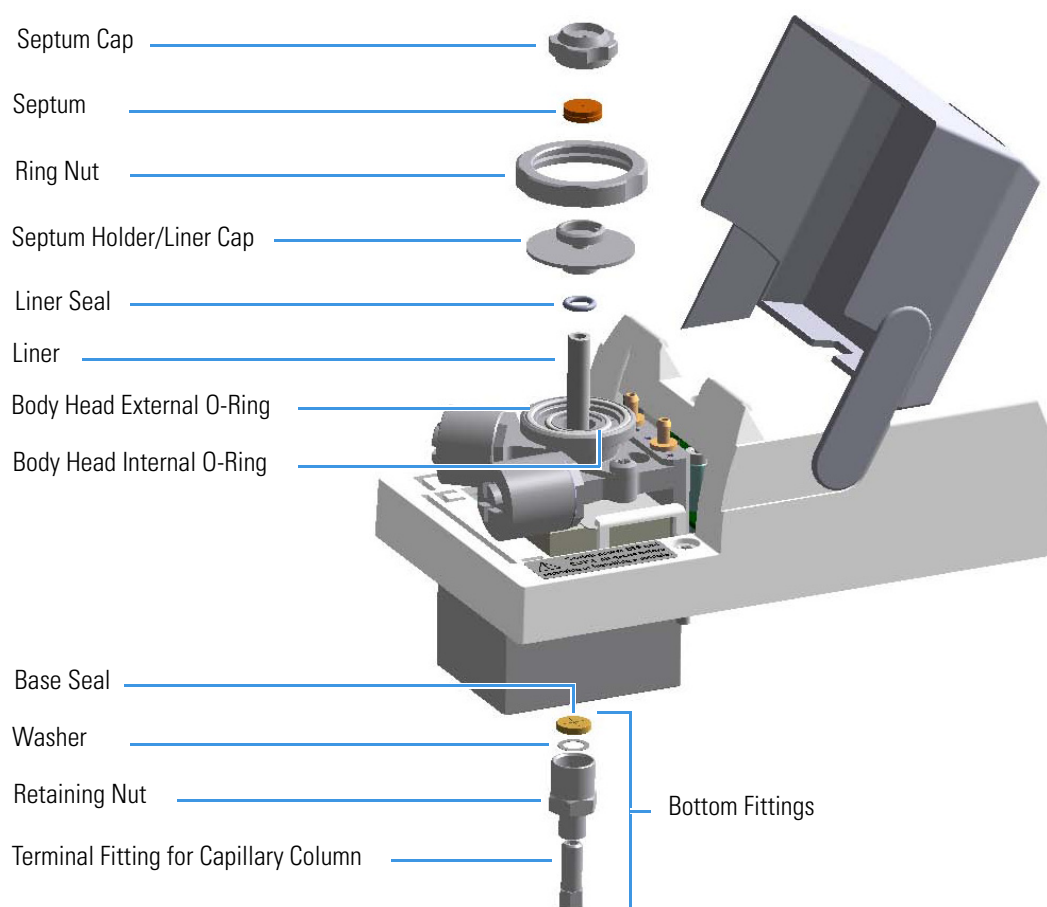
Figure 79. SSL Injector: Components
