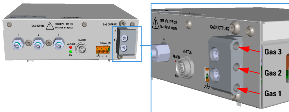
Figure 534. Detector Gas Tubings Connection to the GDI Electrical Interface - External View (1)
