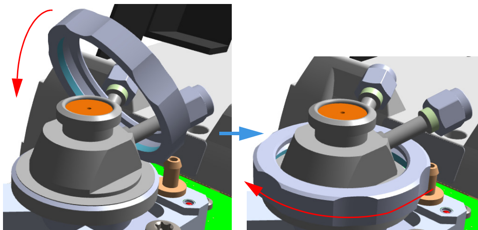
Figure 339. Purge & Trap Adapter (4)
