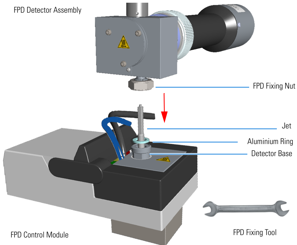
Figure 161. FPD Installation
