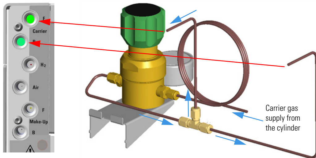
Figure 443. Front and Back Gas Carrier Inlets Connection
