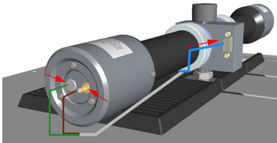
Figure 439. Primary FPD Detector Cables Connection
