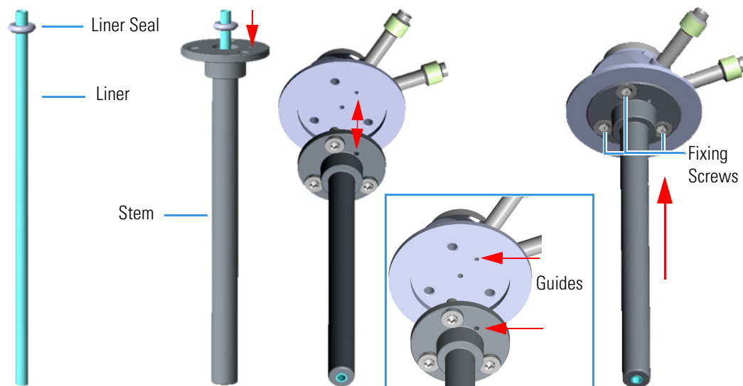
Figure 412. Adapter Assembly
