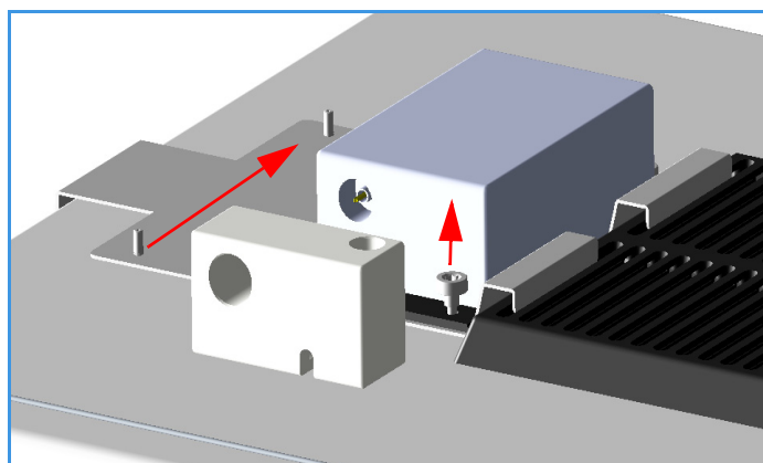
Figure 505. High Voltage Discharge Cable Connection (1)
