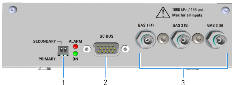
Figure 581. Auxiliary Gas Module Connections
