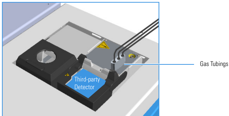
Figure 533. Bending of the Detector Gas Tubings on the TRACE 1310 Auxiliary Oven
