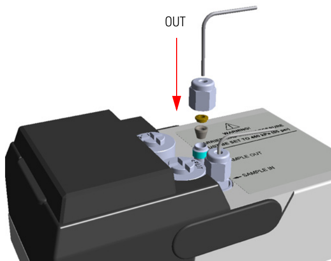
Figure 460. Sample Out Line Connection
