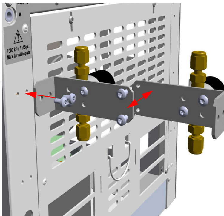
Figure 574. Double Solenoid Valve Assemble Installation
