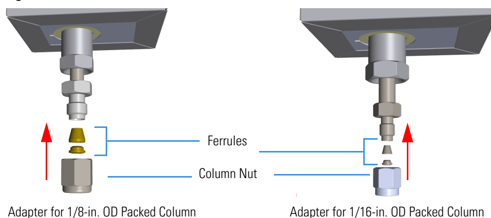
Figure 347. Column Nut and Ferrules (2)
