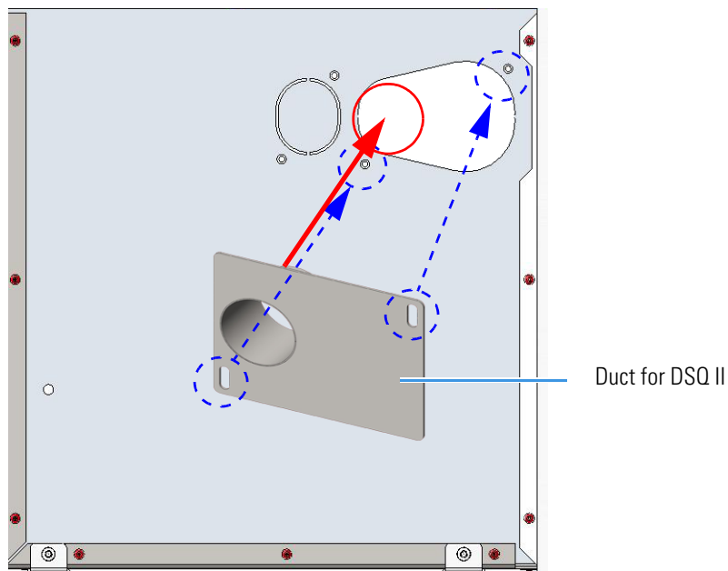
Figure 634. Perform the Duct for DSQ II (2)
