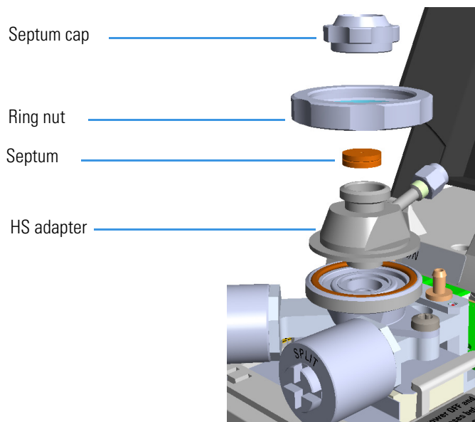
Figure 351. HS Adapter (1)
