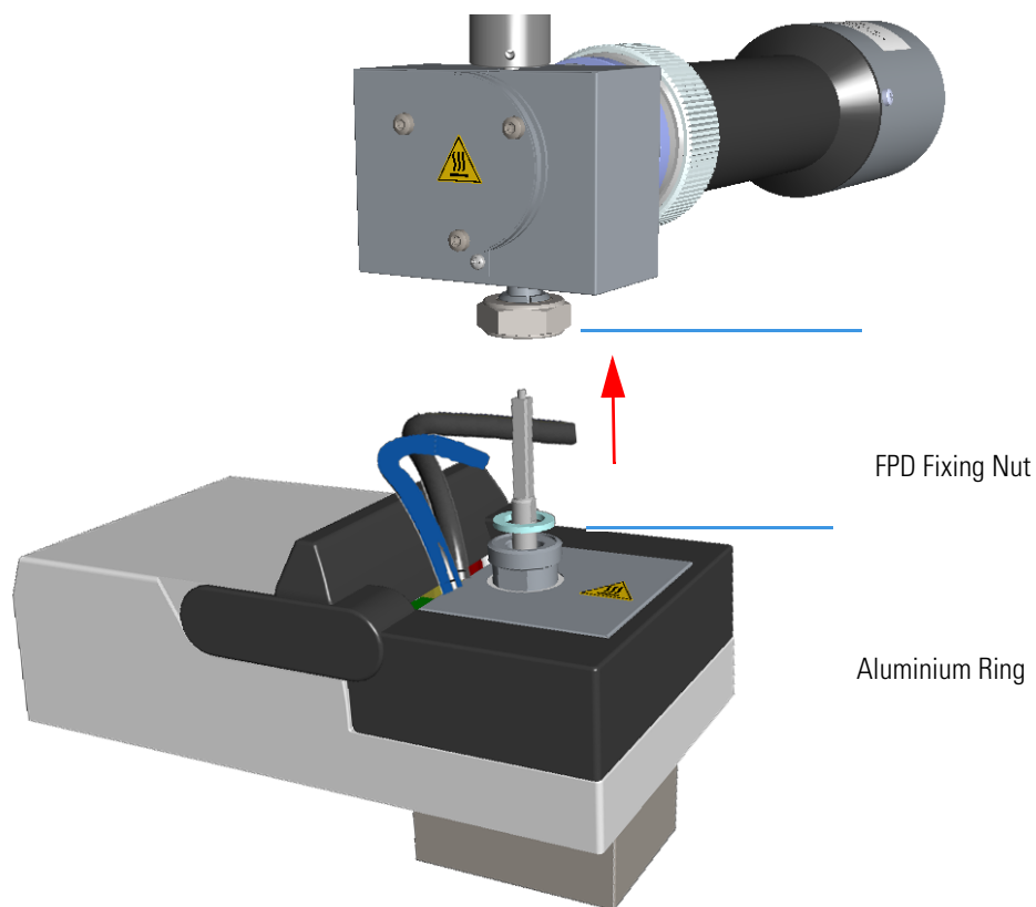
Figure 290. FPD Detector Removal
