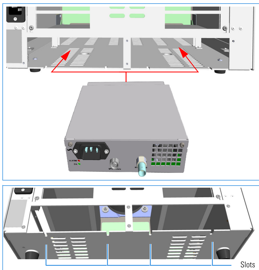
Figure 471. Module Installation (2)
