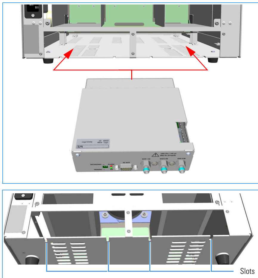
Figure 601. Module Installation (2)
