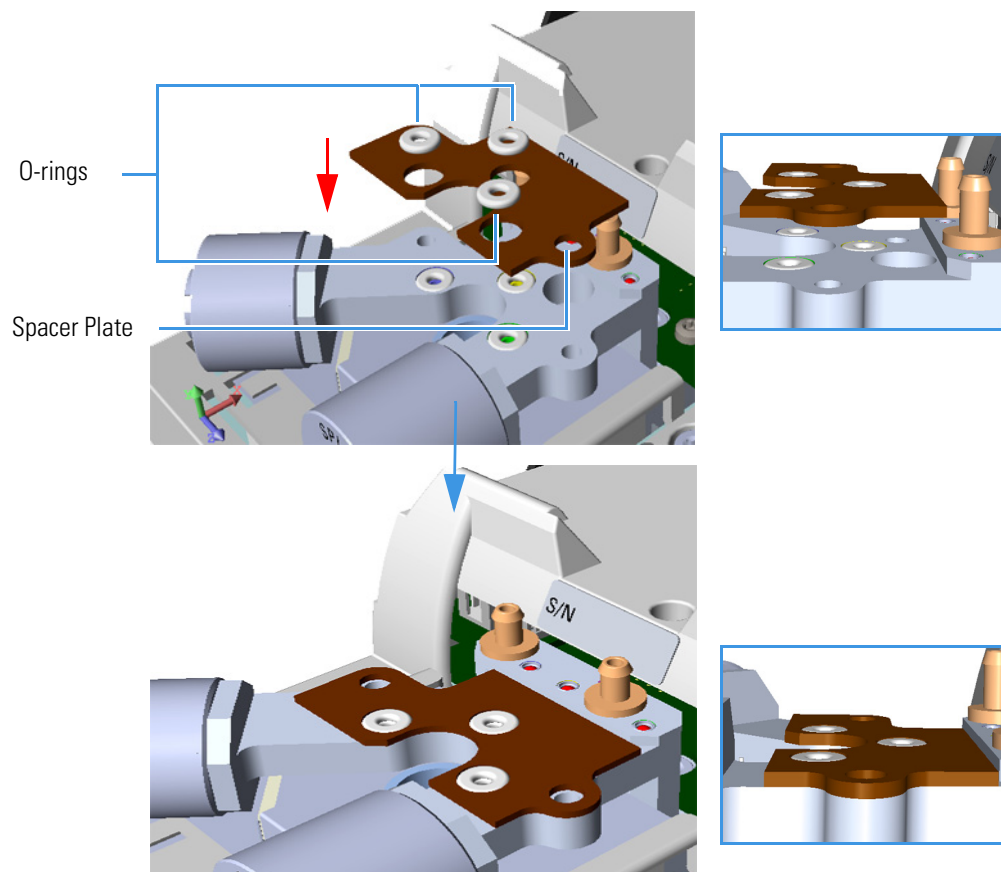
Figure 416. Spacer Plate
