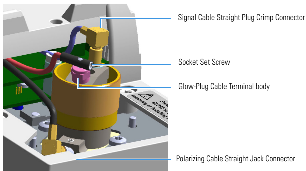
Figure 247. FID Cables Disconnection
