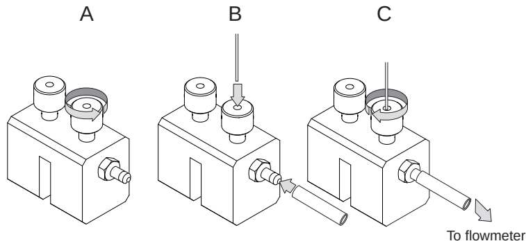
Figure 359. Column Flowmeter Connector
