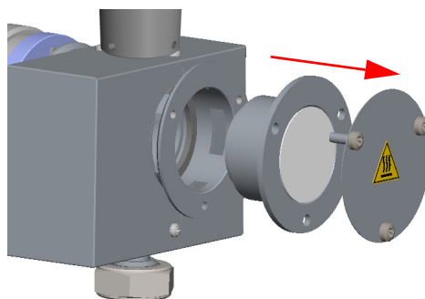
Figure 429. Mirror Plug Removal
