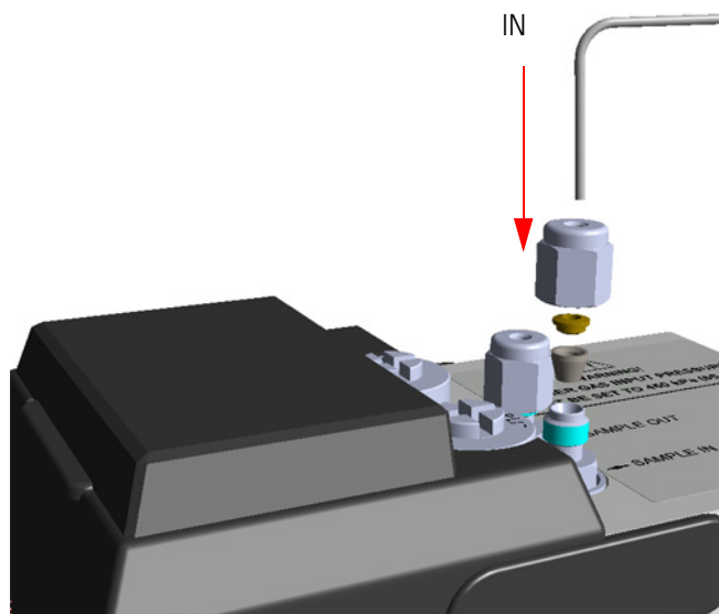
Figure 459. Sample In Line Connection
