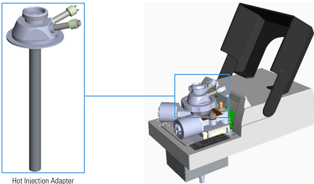
Figure 410. Hot Injection Adapter
