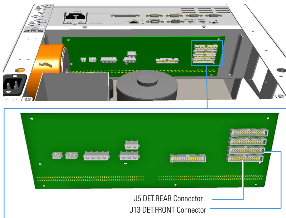
Figure 523. GC Backplane Board Layout
