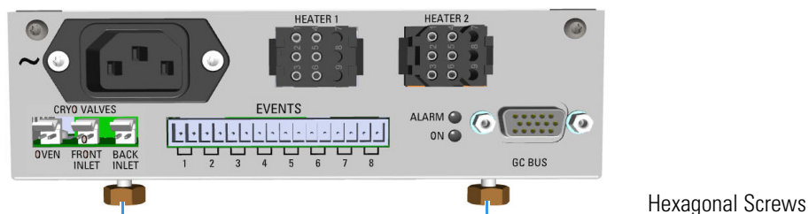
Figure 552. Module Installation (1)
