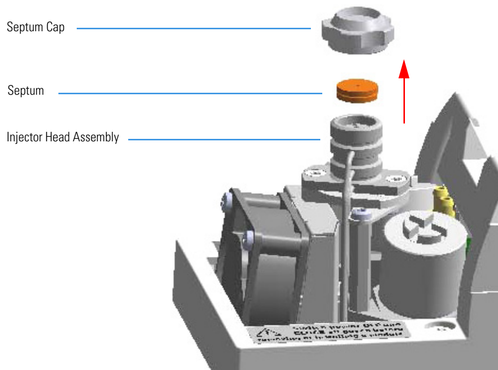
Figure 331. PTV/PTVBKF Injector: Septum Replacement
