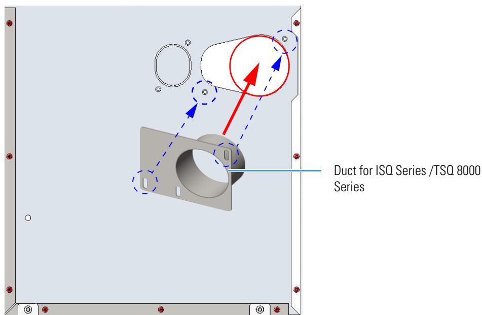
Figure 627. Perform the Duct for ISQ Series / TSQ 8000 Series (2)
