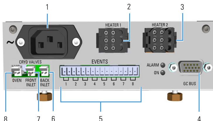
Figure 476. Aux Temperature/Cryo Module Connections
