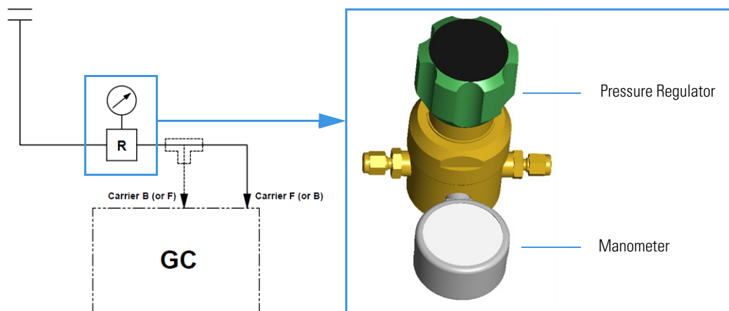
Figure 441. Schematic Diagram
