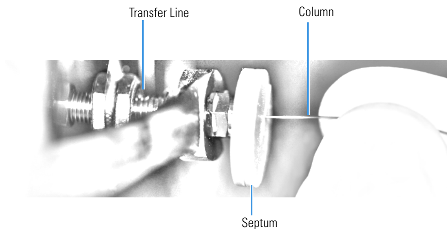
Figure 398. Positioning the Column in the Transfer Line
