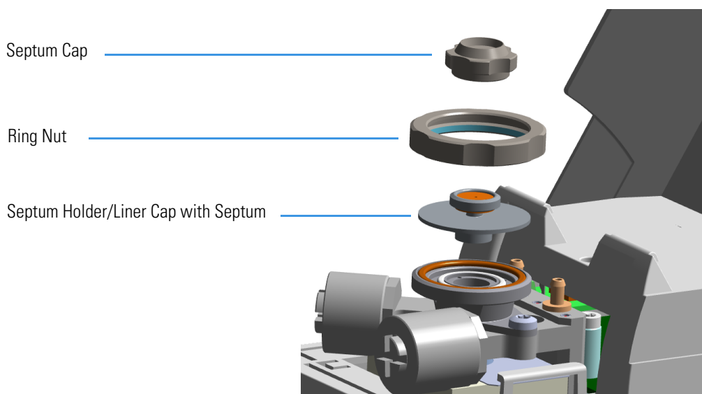
Figure 335. Injector Top Parts Removal
