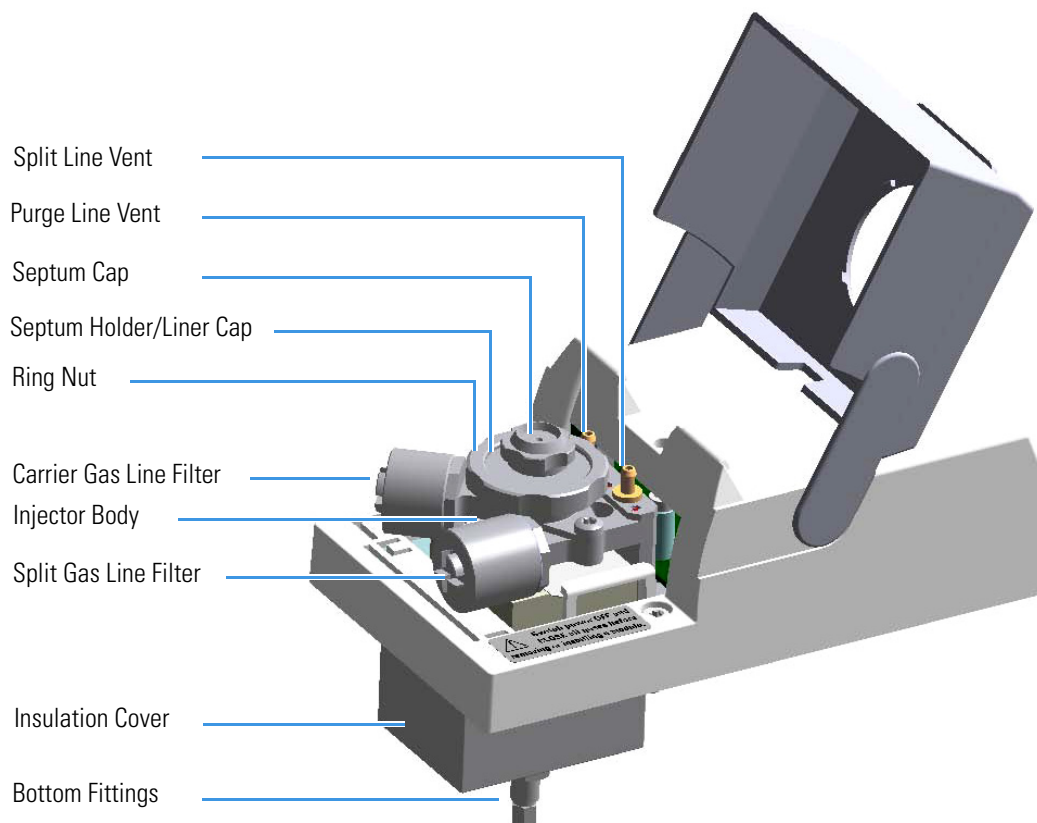
Figure 78. SSL Module Components
