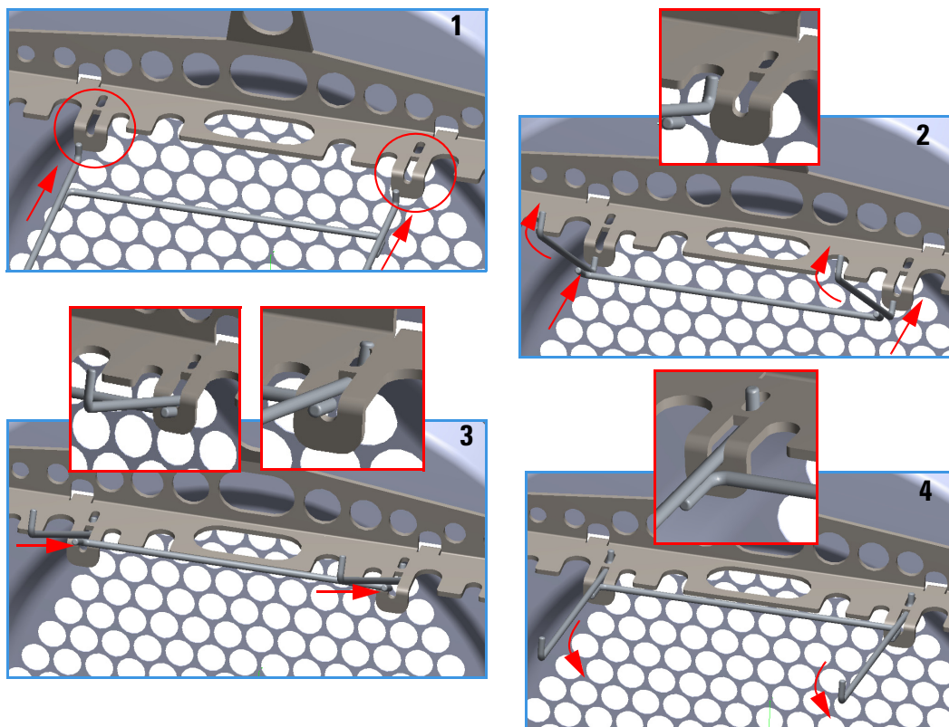
Figure 449. Hooking the Removable rack for Capillary Column
