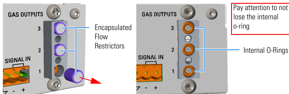
Figure 519. Flow Restrictor Replacement
