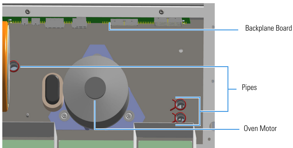
Figure 209. Pipes
