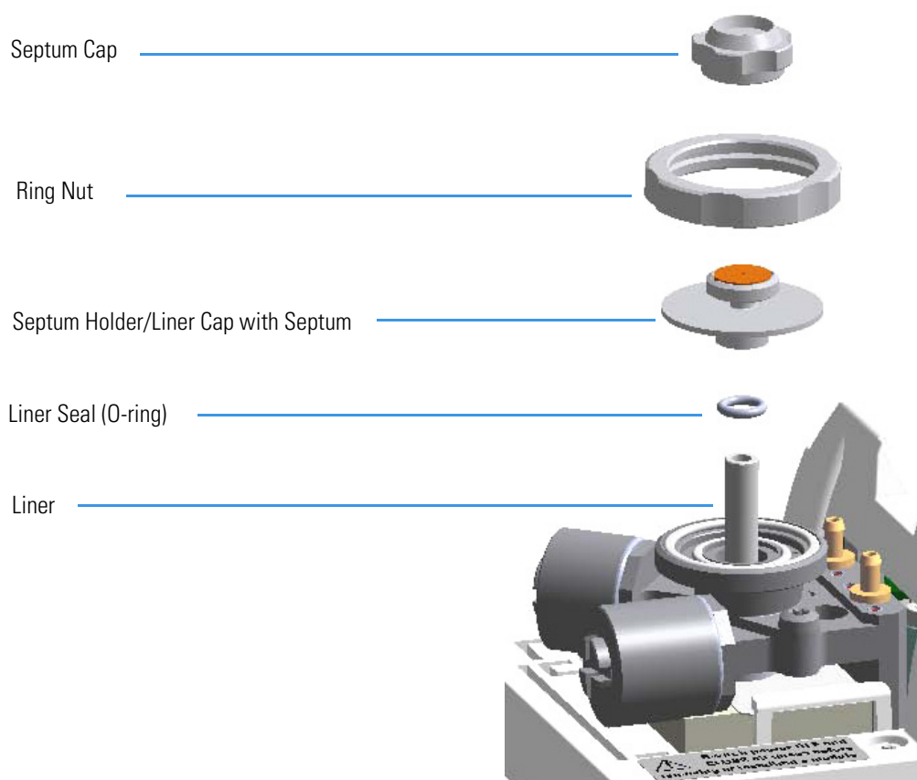
Figure 414. Injector Top Parts Removal
