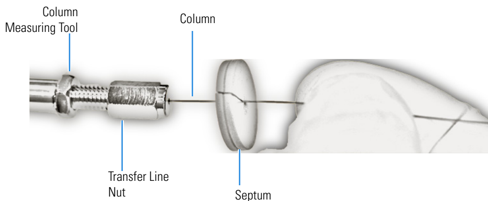
Figure 396. Pulling the Column Back from the Transfer Line Nut
