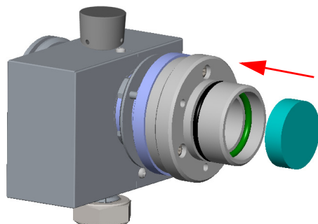
Figure 433. Filter Remounting
