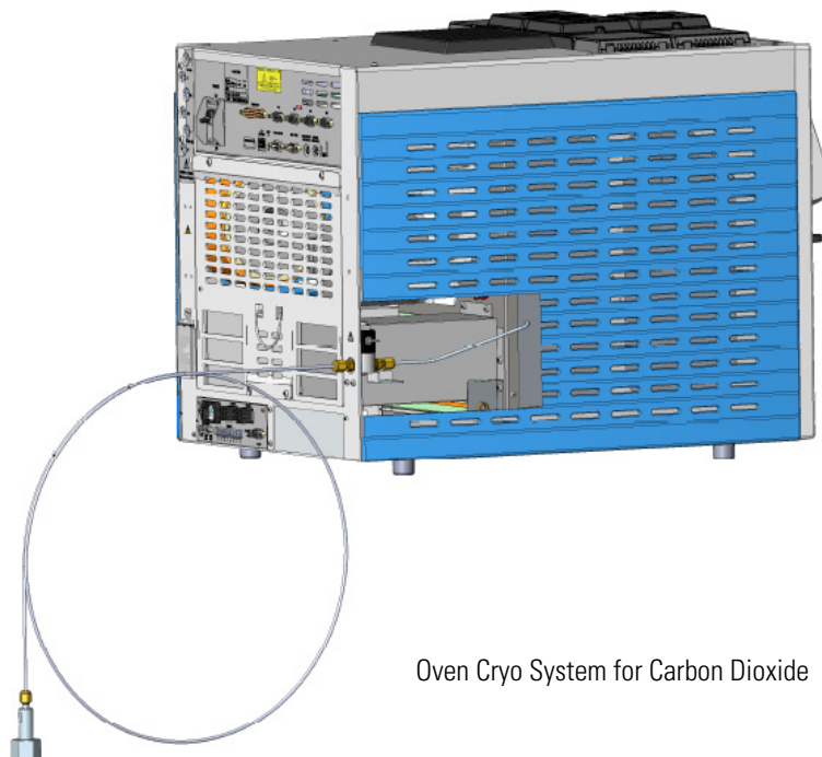
Figure 545. Oven Cryo System for Carbon Dioxide and Liquid Nitrogen
