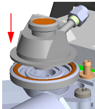
Figure 353. HS Adapter (3)
