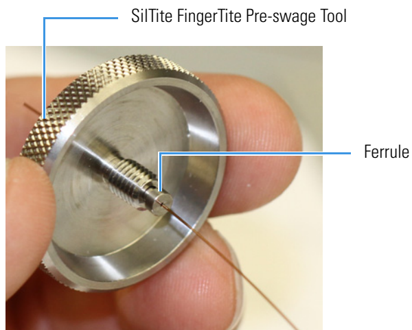
Figure 382. Pre-swaging the Ferrule to the 30 cm Fused Silica Tubing
