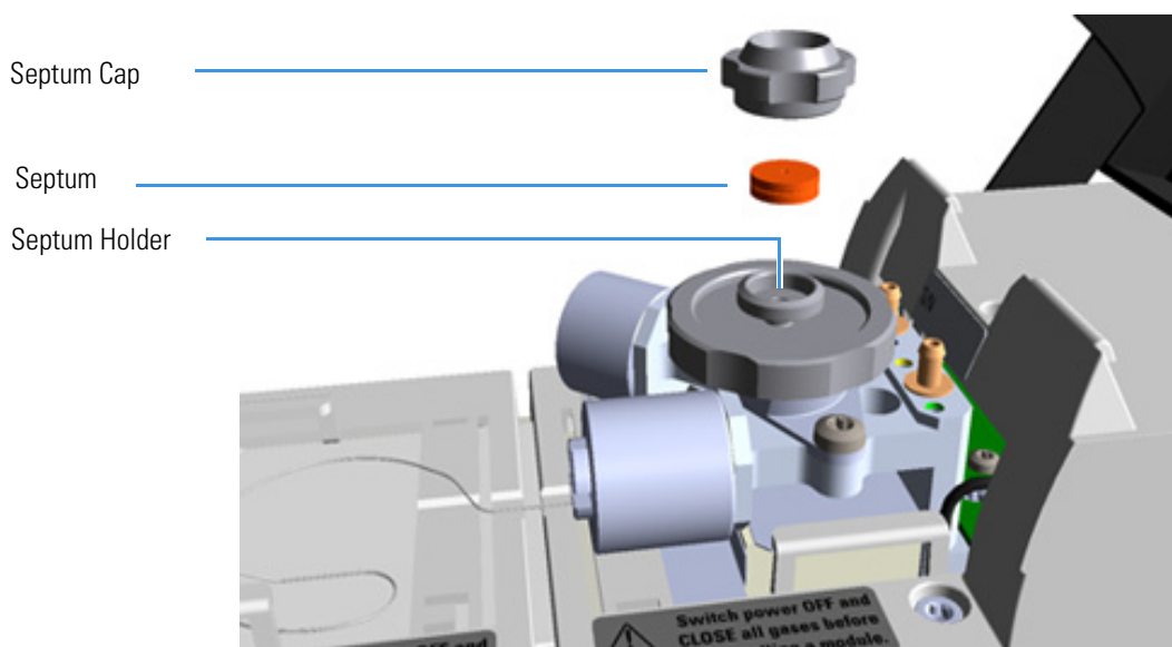
Figure 101. HeS-S/SL Injector: Septum Replacement
