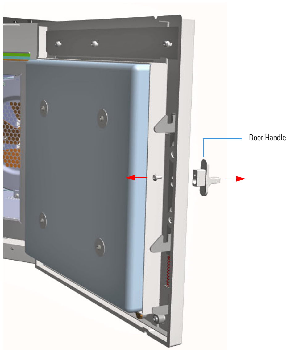
Figure 618. Door Handle Removal
