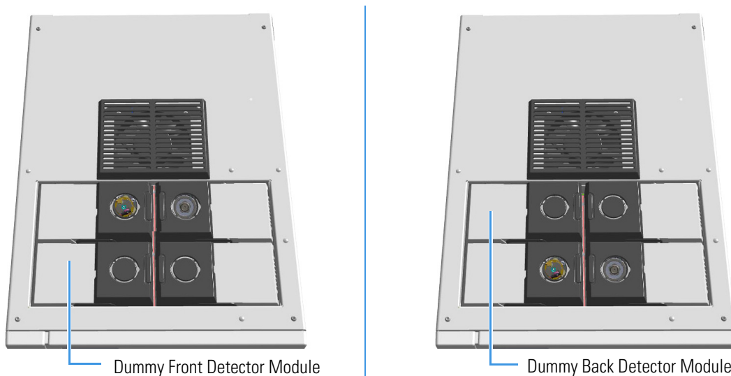
Figure 375. Location of Detector Modules on your TRACE 1300/TRACE 1310 GC
