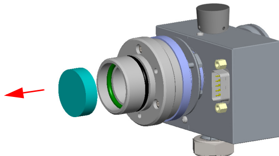
Figure 292. Filter Removal
