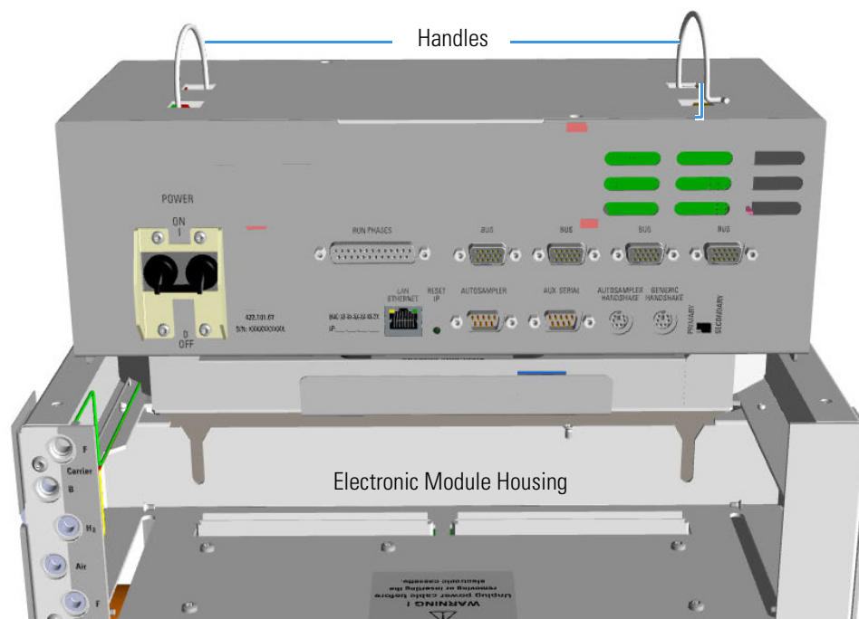
Figure 201. Electronic Module Extraction
