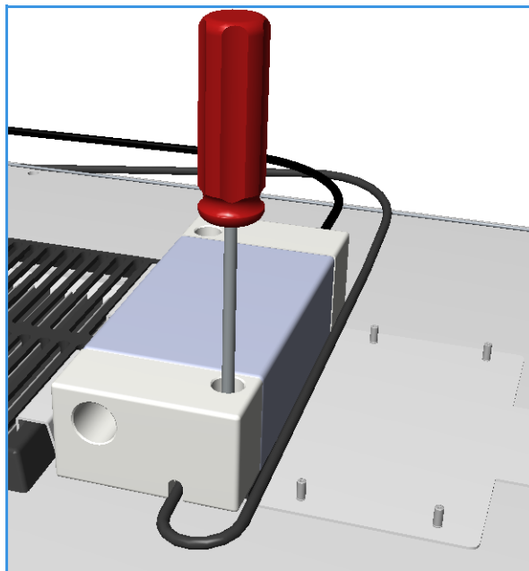
Figure 510. Pulses Cable Connection (3)
