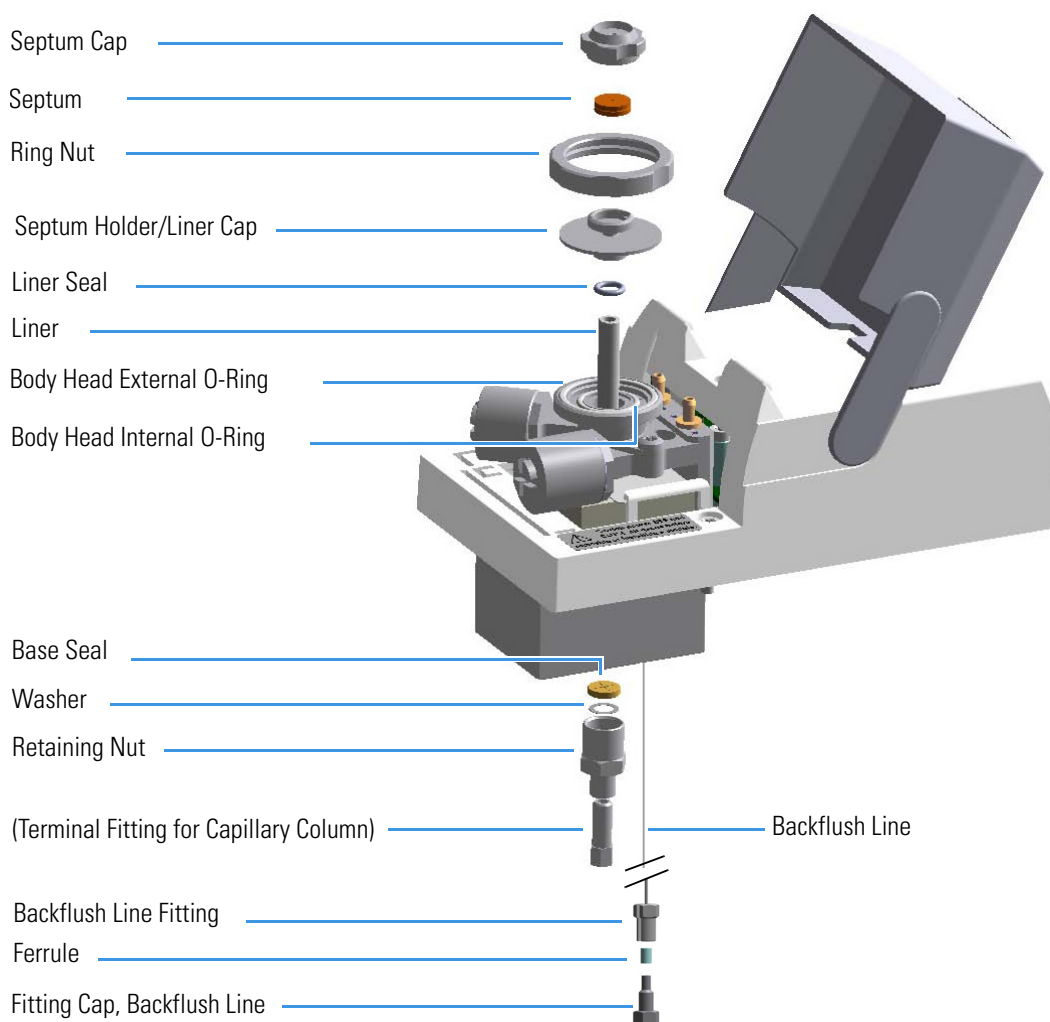
Figure 86. SSLBKF Injector Components
