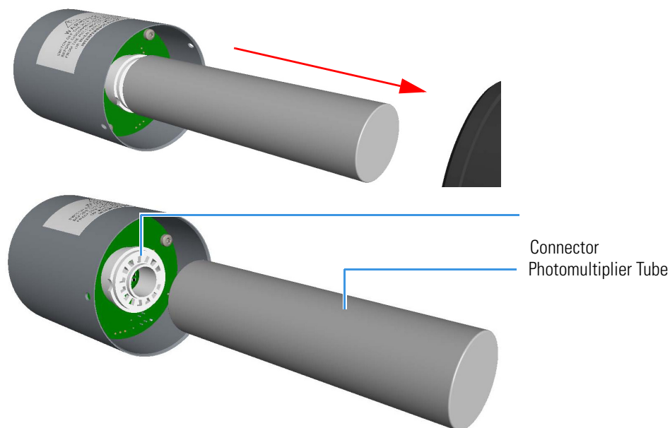
Figure 321. Photomultiplier Tube Replacement (1)
