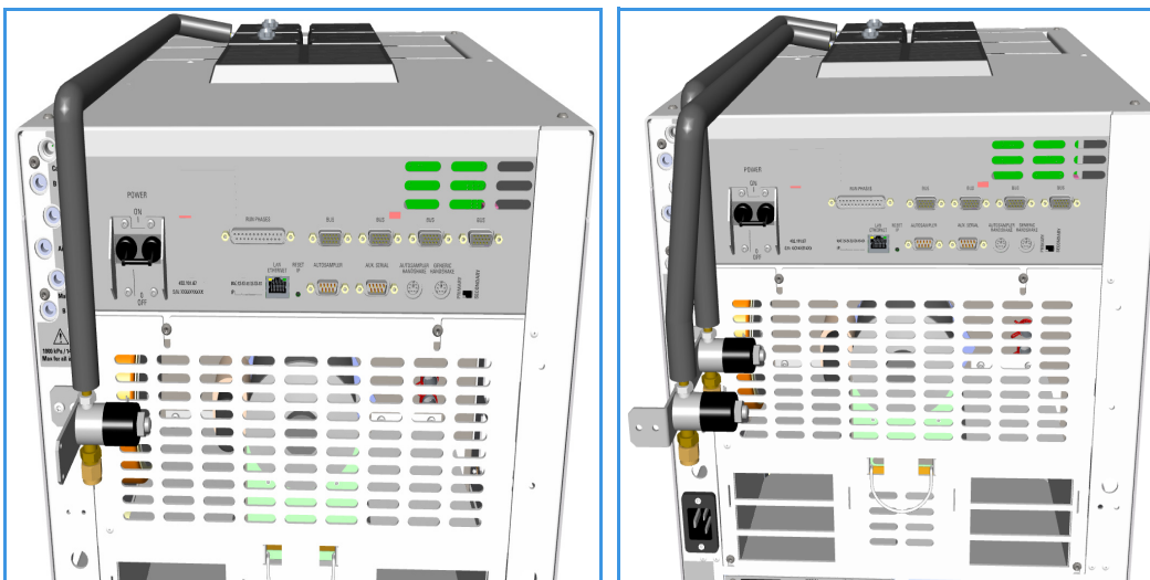
Figure 565. PTV and PTVBKF Single and Double Cryo System for Liquid Nitrogen
