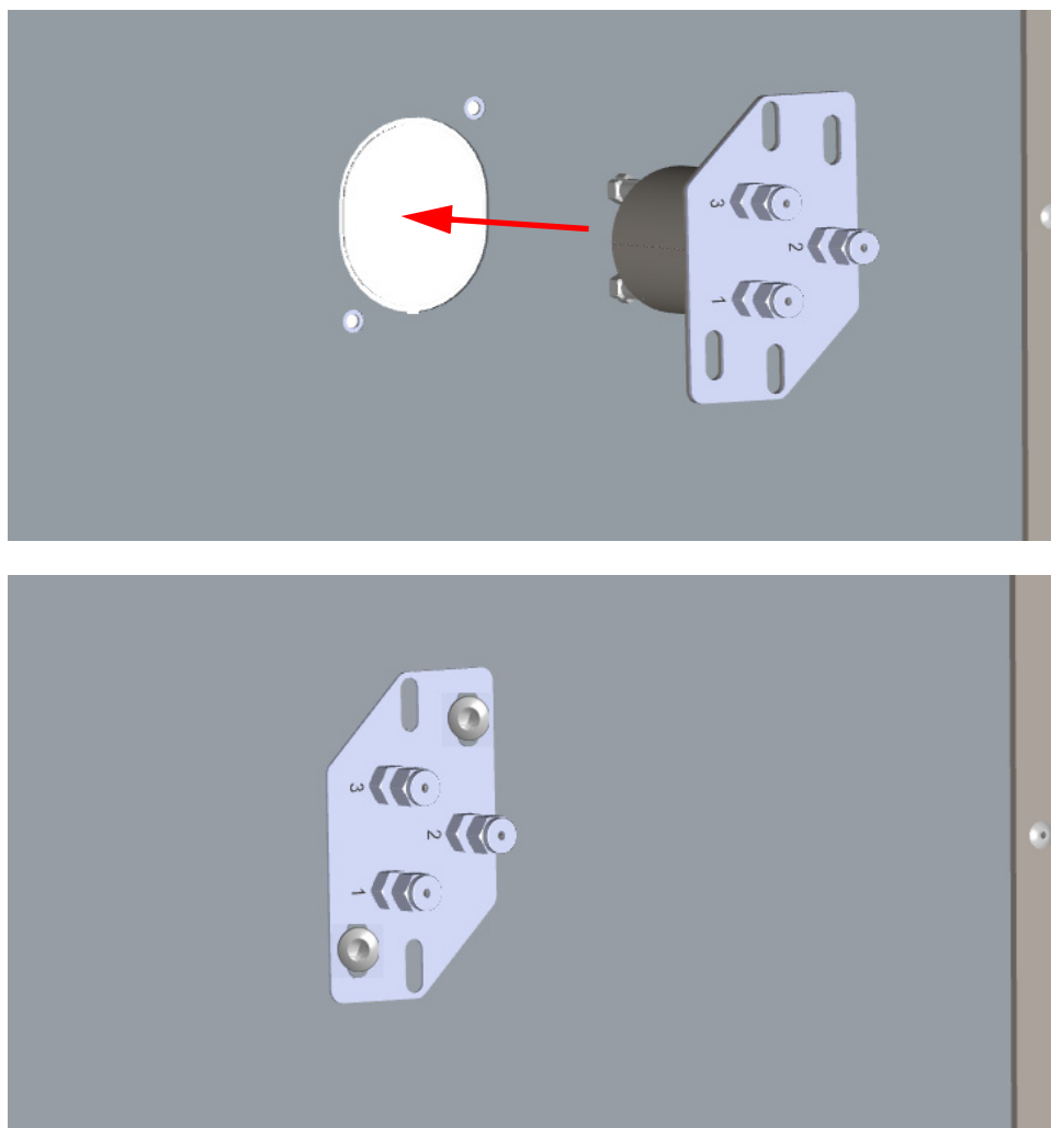
Figure 595. Perform the Duct for the Auxiliary Gas Interface (4)
