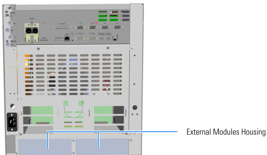
Figure 568. External Modules Housing
