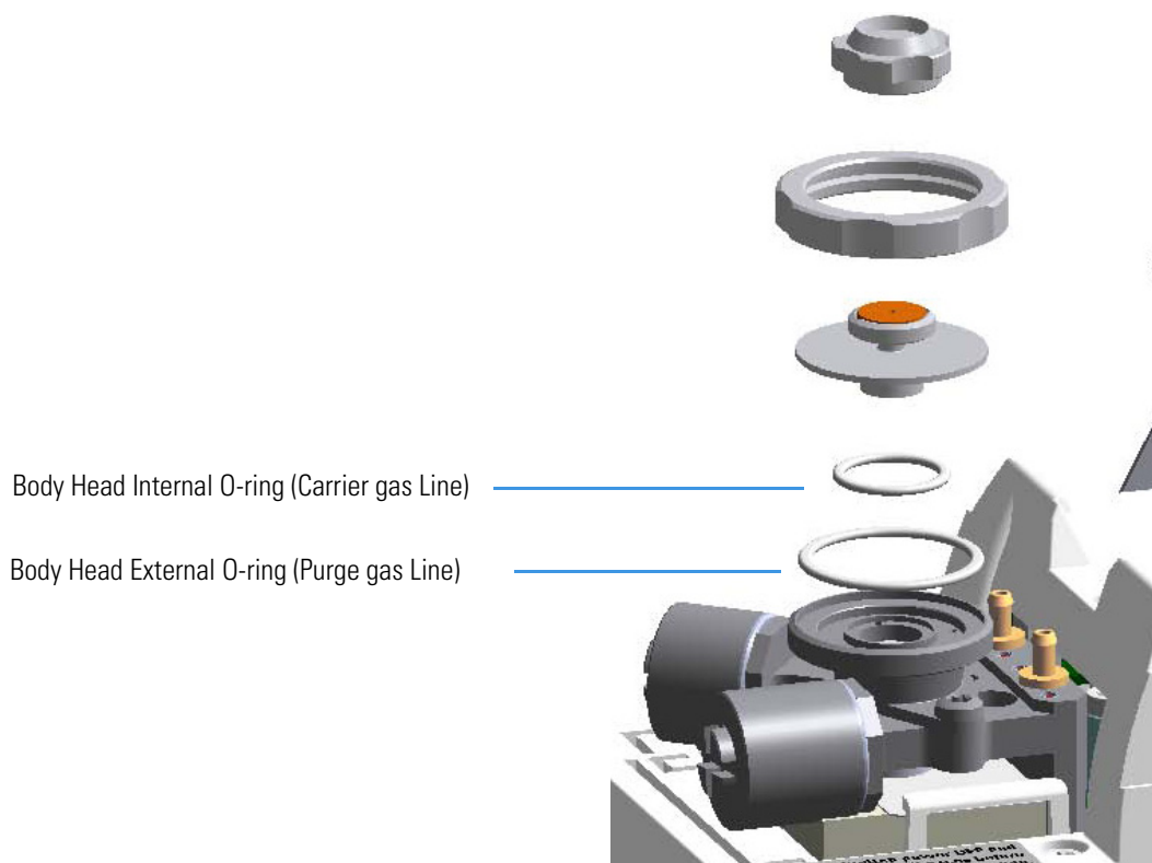
Figure 84. SSL Injector: Body Head O-Rings Replacement
