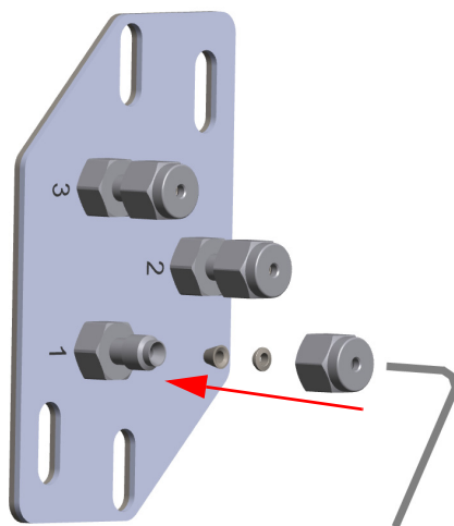
Figure 606. Gas Tubes Connection to the Auxiliary Gas Interface - External View(
