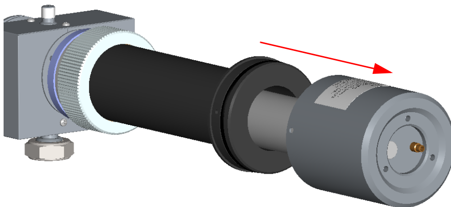
Figure 320. Photomultiplier Tube Housing Removal (2)
