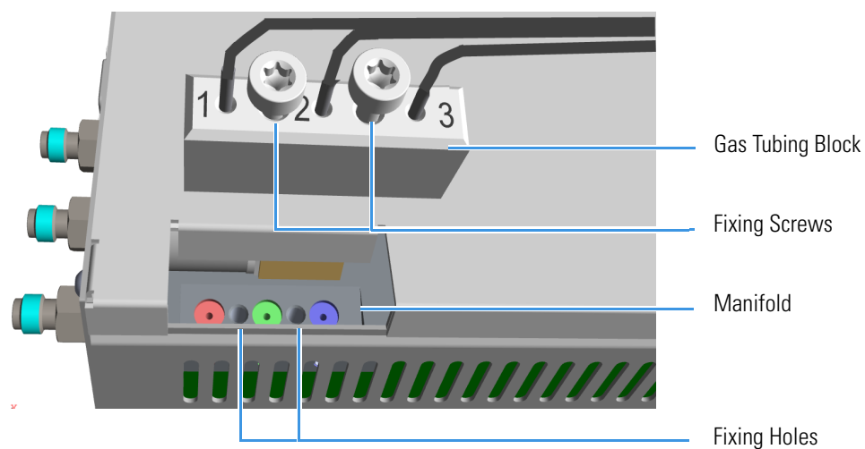
Figure 603. Gas Tubing Block and Manifold
