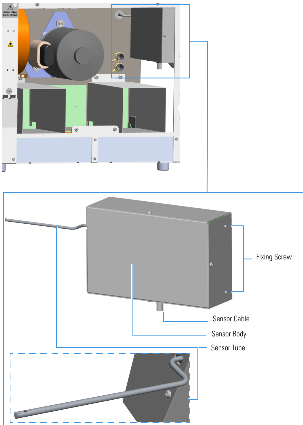
Figure 609. Hydrogen Sensor
