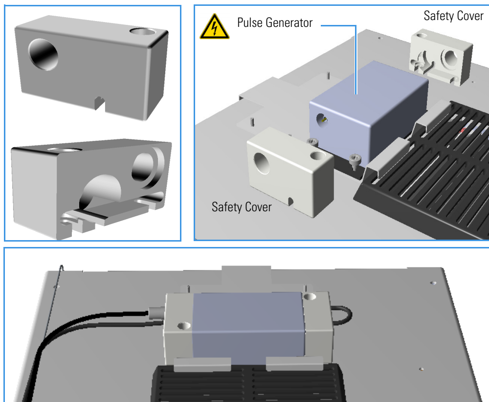
Figure 504. Pulse Generator Safety Covers
