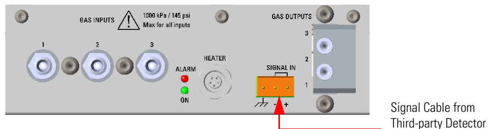
Figure 539. Signal Connection
