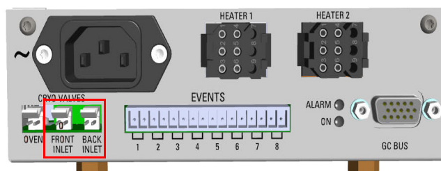
Figure 579. Cryo Valves: Oven
