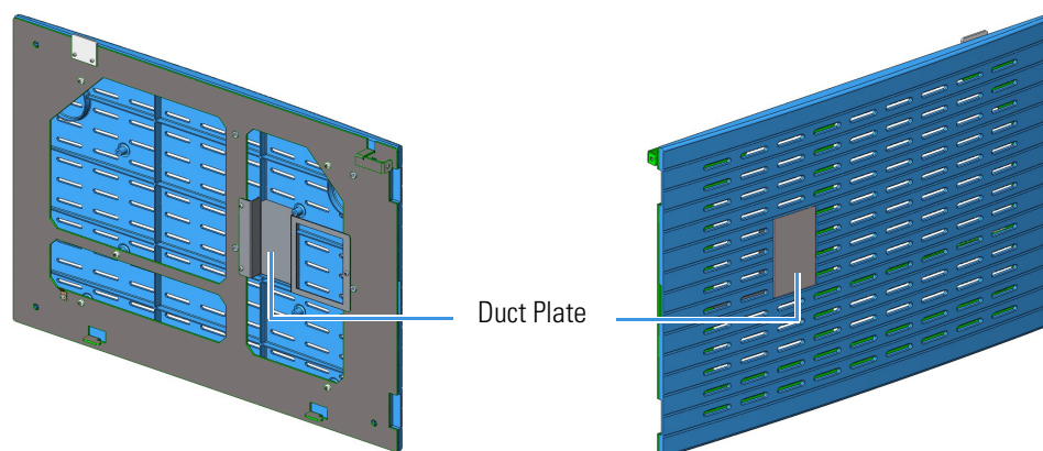
Figure 653. Right Panel for MS
