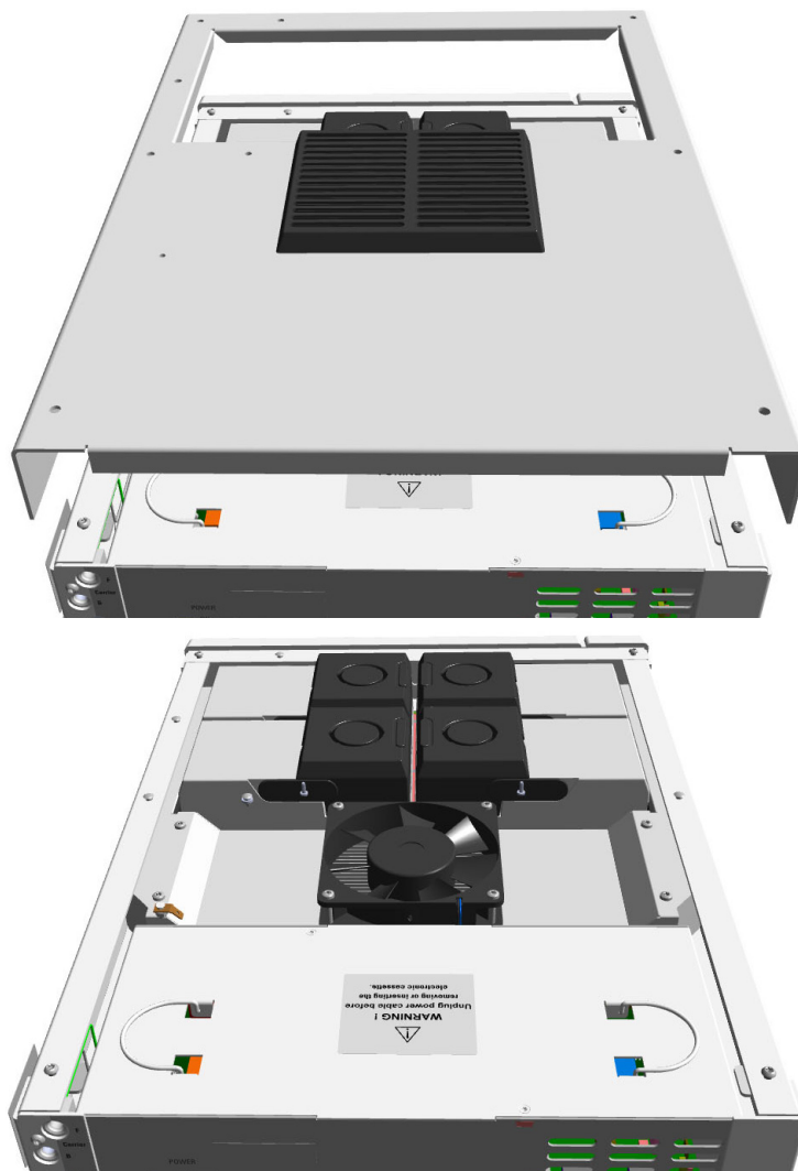
Figure 186. Top Cover Removal (2)
