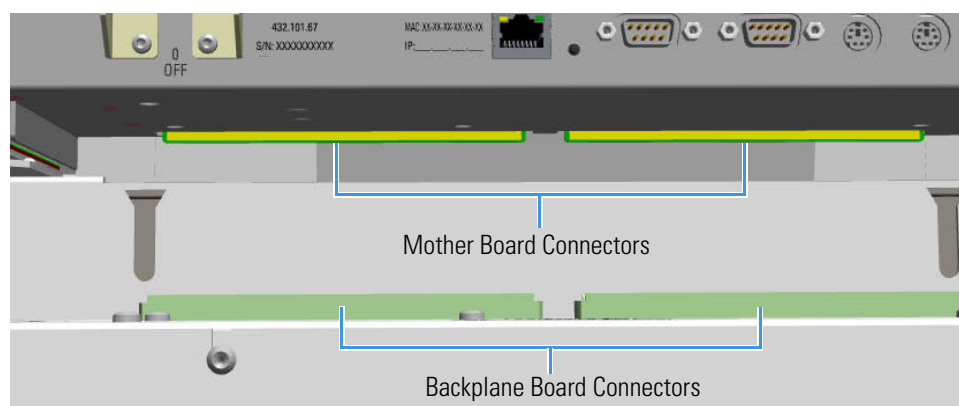
Figure 202. Electronic Module Replacement (1)
