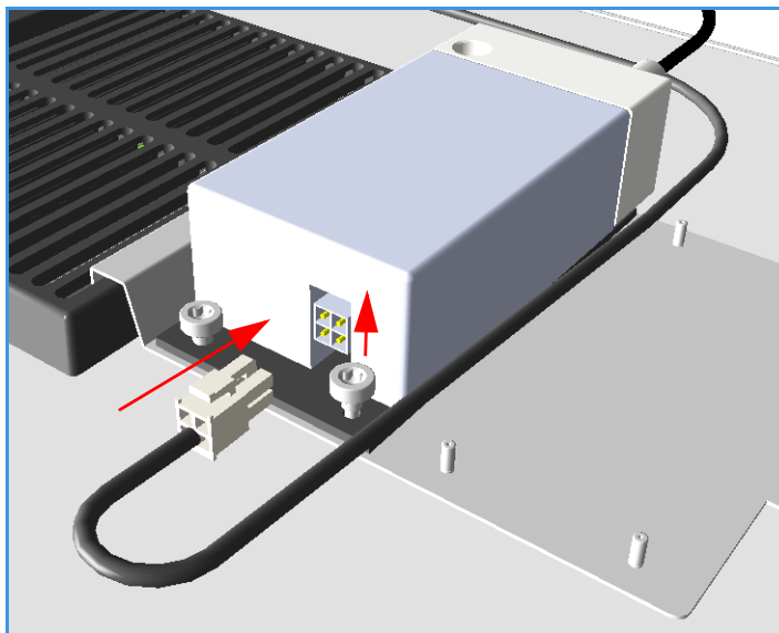
Figure 508. Pulses Cable Connection (1)
