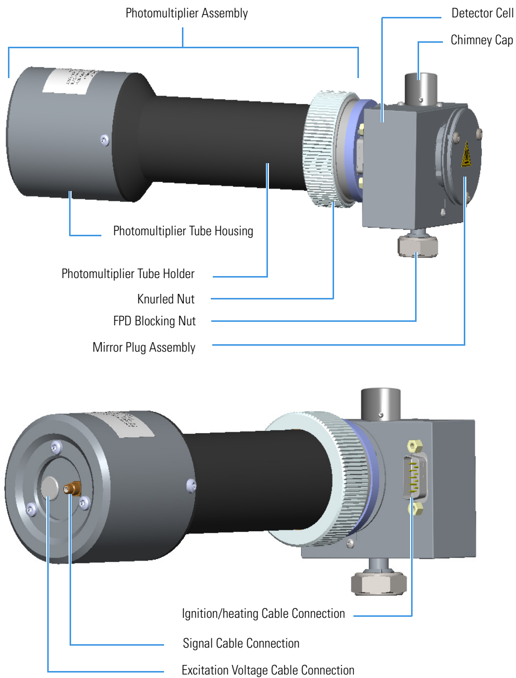
Figure 159. FPD Detector Assembly Components
