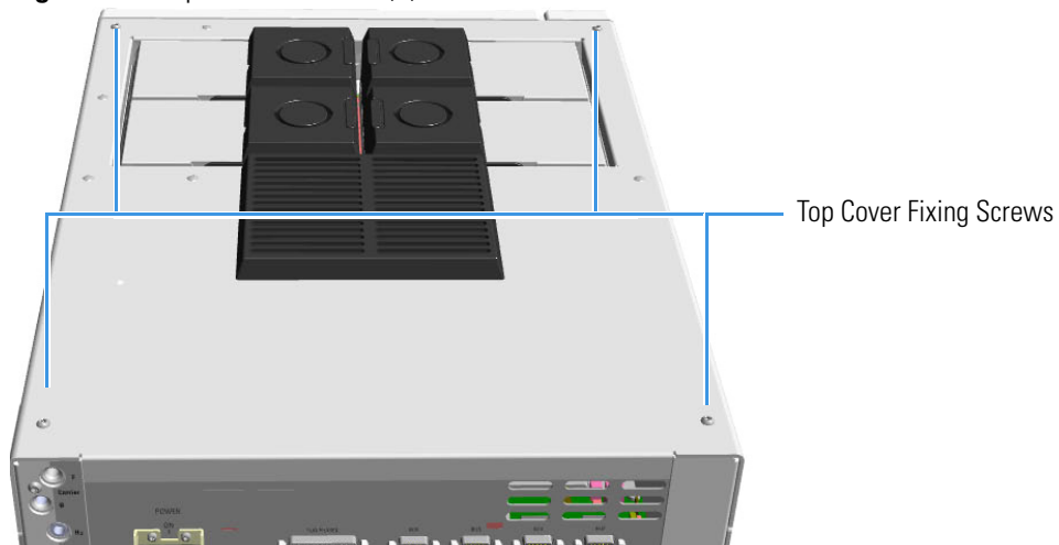
Figure 199. Top Cover Removal (1)
