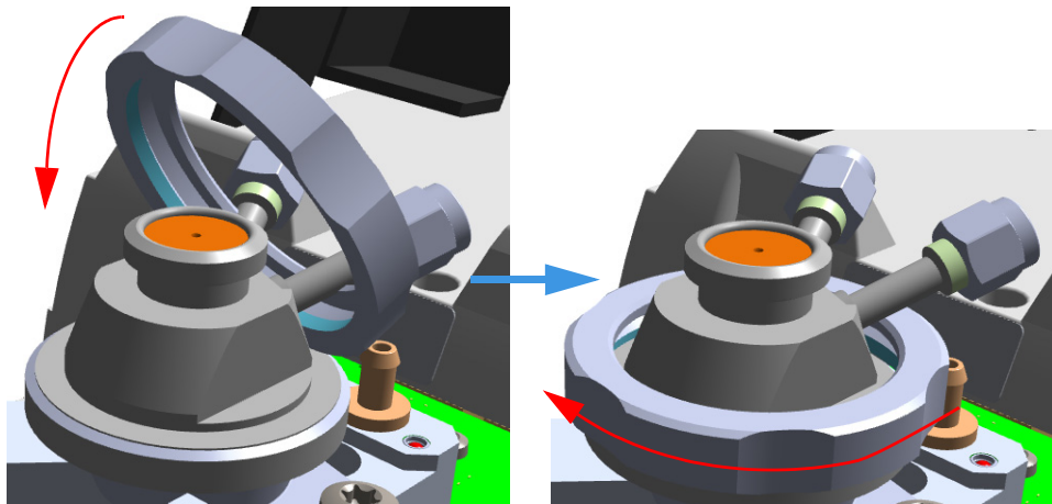
Figure 420. Hot Injection Adapter (3)
