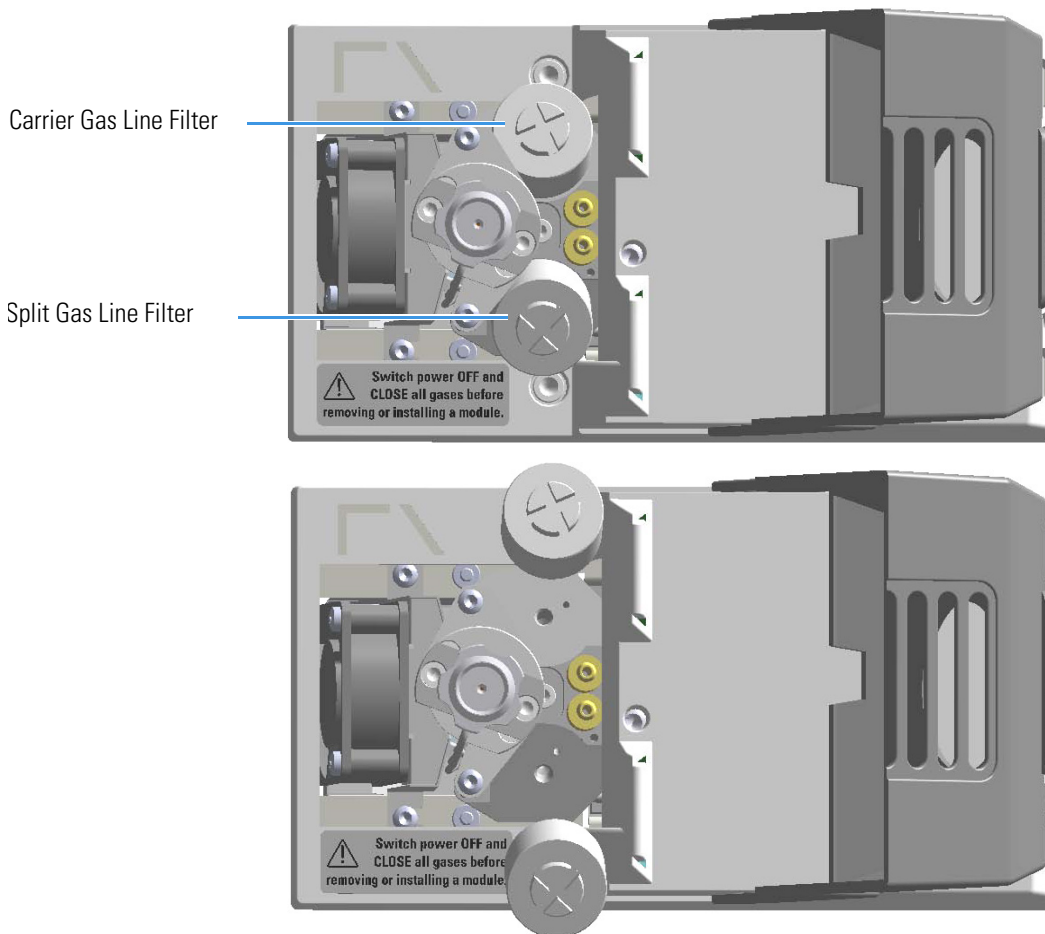
Figure 110. PTV Injector: Active Filters Replacement
