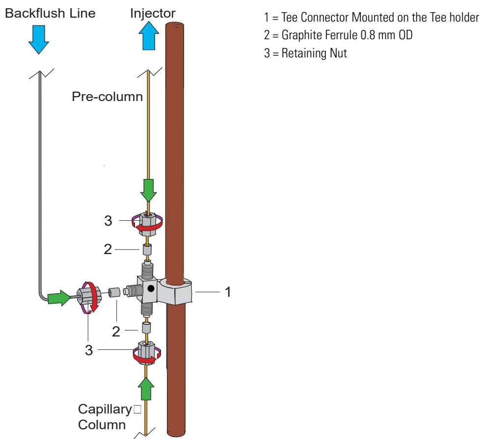
Figure 371. Connecting Backflush Line, Precolumn, and Capillary Column
