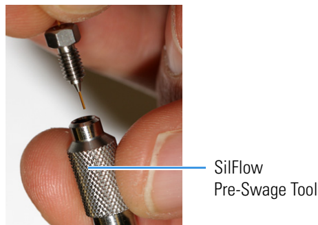
Figure 390. Inserting the Column and Ferrule into the SilFlow Pre-Swage Tool
