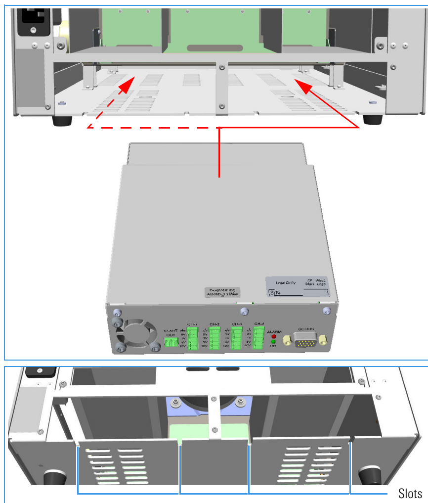
Figure 542. AOI Installation (2)
