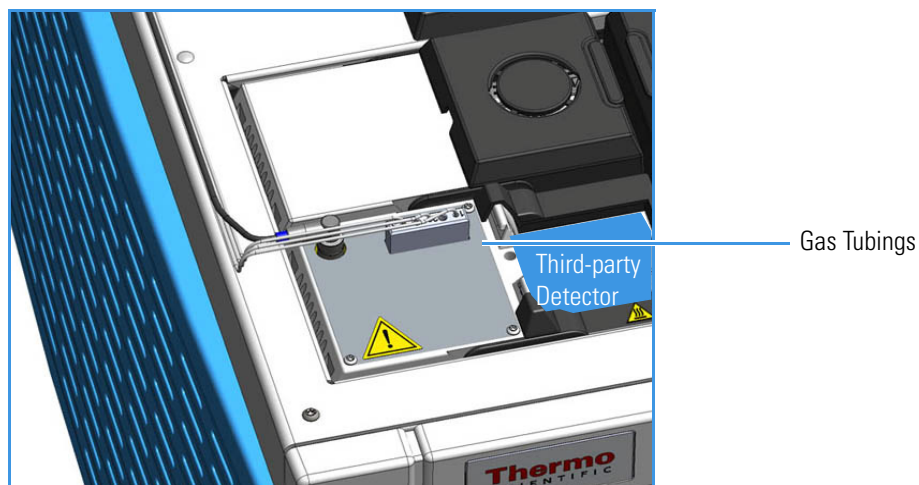
Figure 533. Bending of the Detector Gas Tubings on the TRACE 1310 Auxiliary Oven
