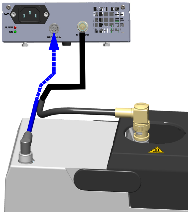
Figure 474. Signal Cable Connection
