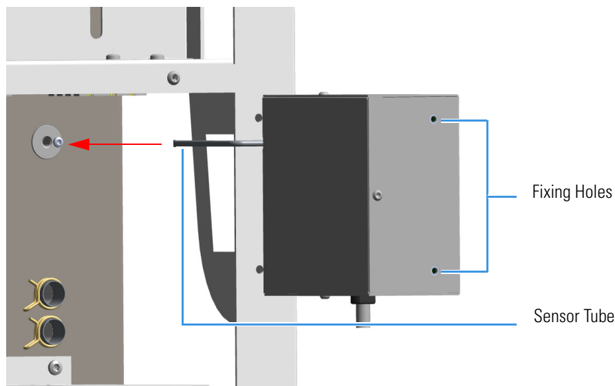
Figure 613. Hydrogen Sensor Installation (1)
