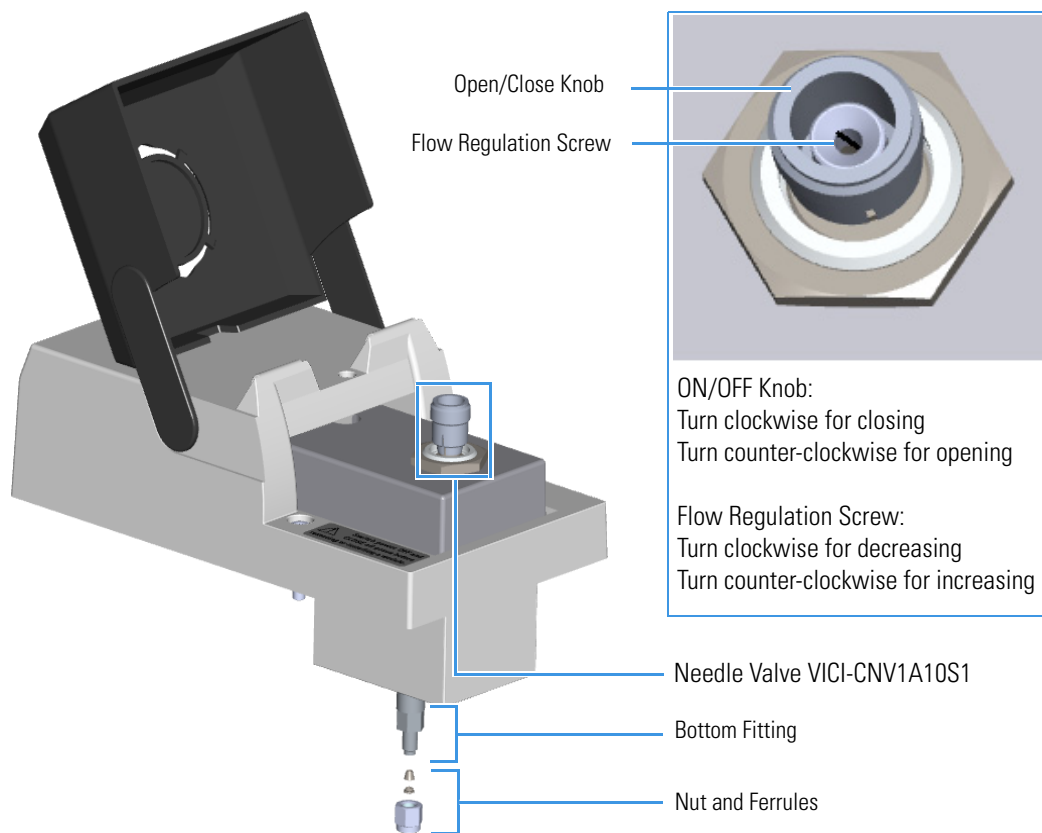
Figure 408. FTIR Make-up Module
