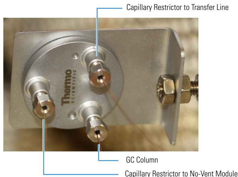
Figure 400. Correct Orientation of Columns to Microfluidics Splitter
