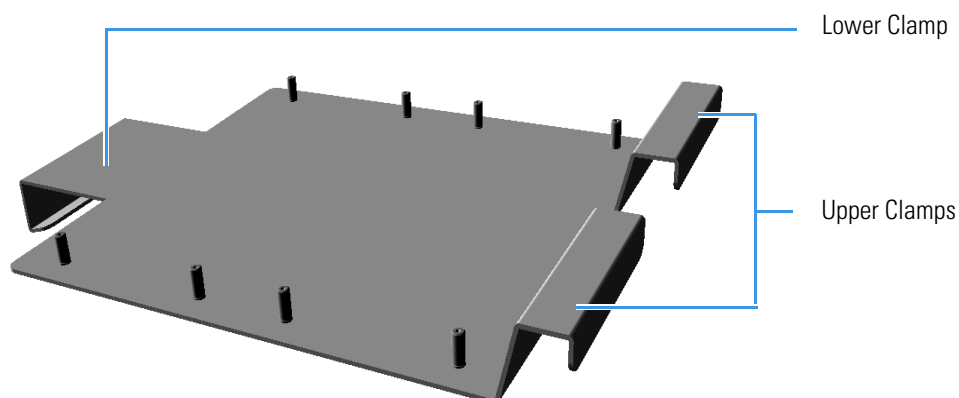
Figure 496. Support Bracket
