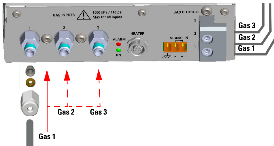
Figure 536. Gas Lines Connection to the GDI Electrical Interface
