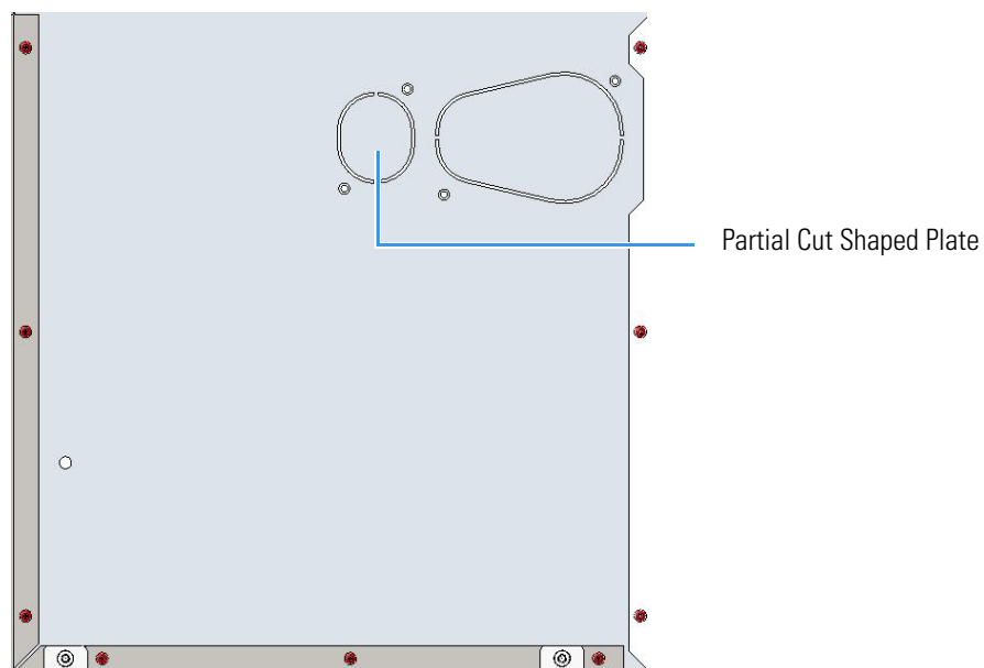
Figure 586. Perform the Duct for the Auxiliary Gas Interface (1)
