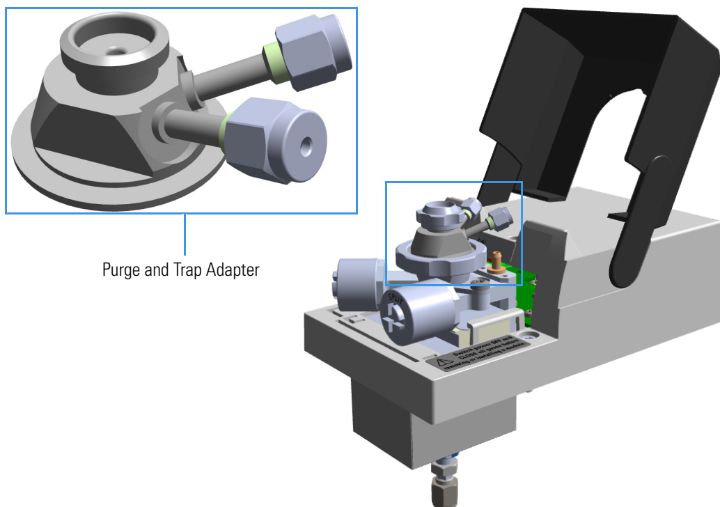
Figure 333. Purge & Trap Adapter
