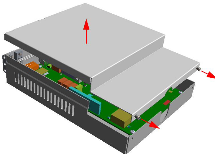
Figure 514. Assemble GDI Electrical Interface (1)
