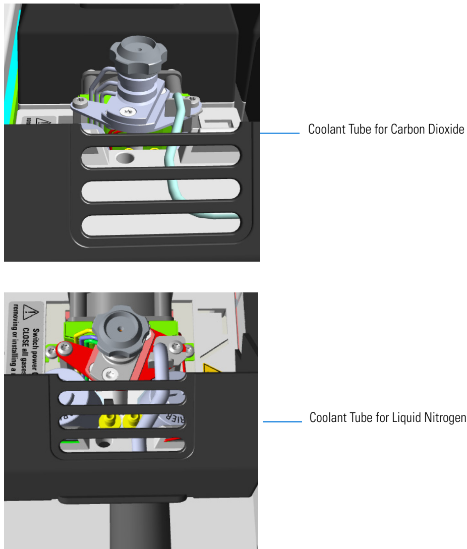
Figure 576. Installation of the Coolant Tubes for Carbon Dioxide and Liquid Nitrogen
