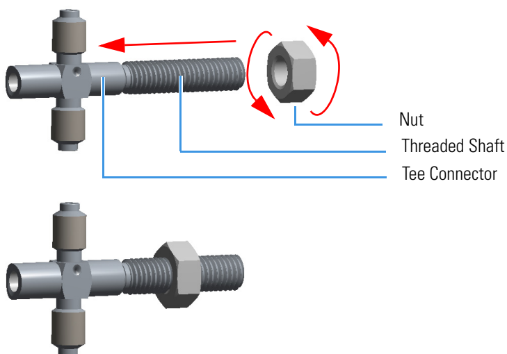
Figure 363. Assembling Tee Connector and Mounting Bracket (3)
