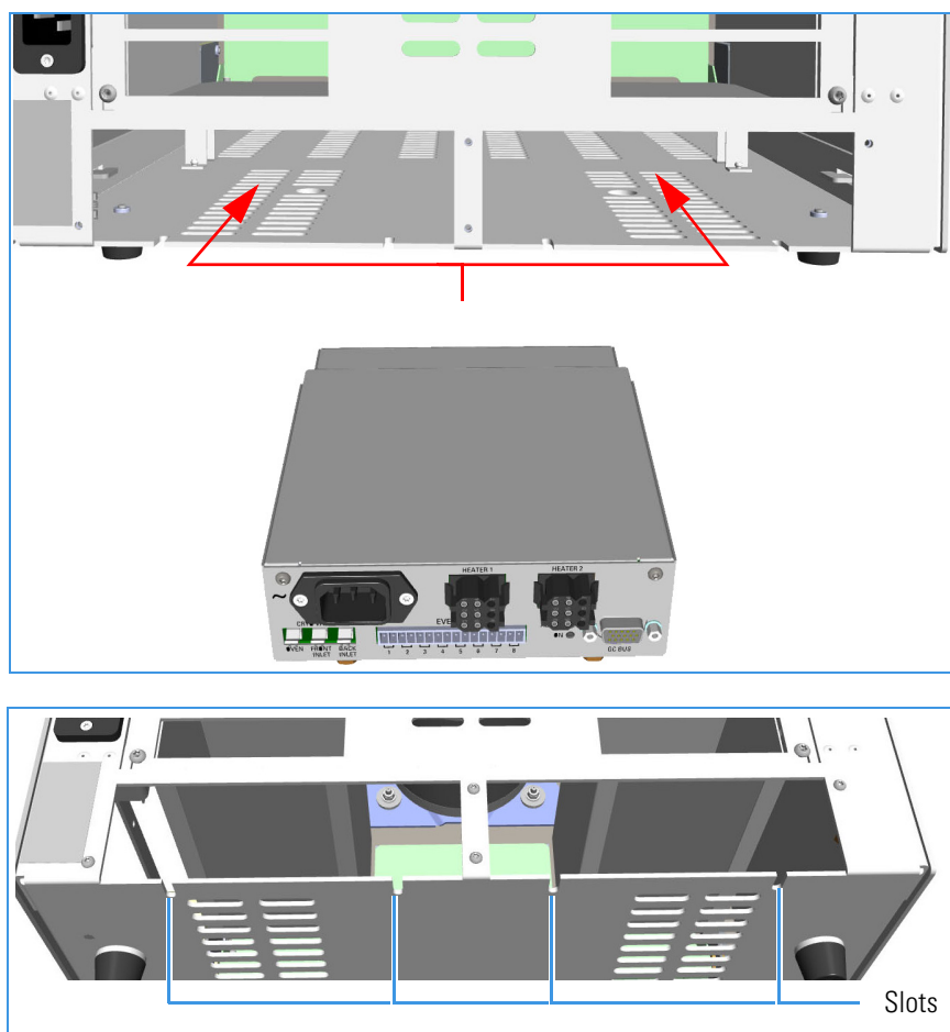
Figure 553. Module Installation (2)
