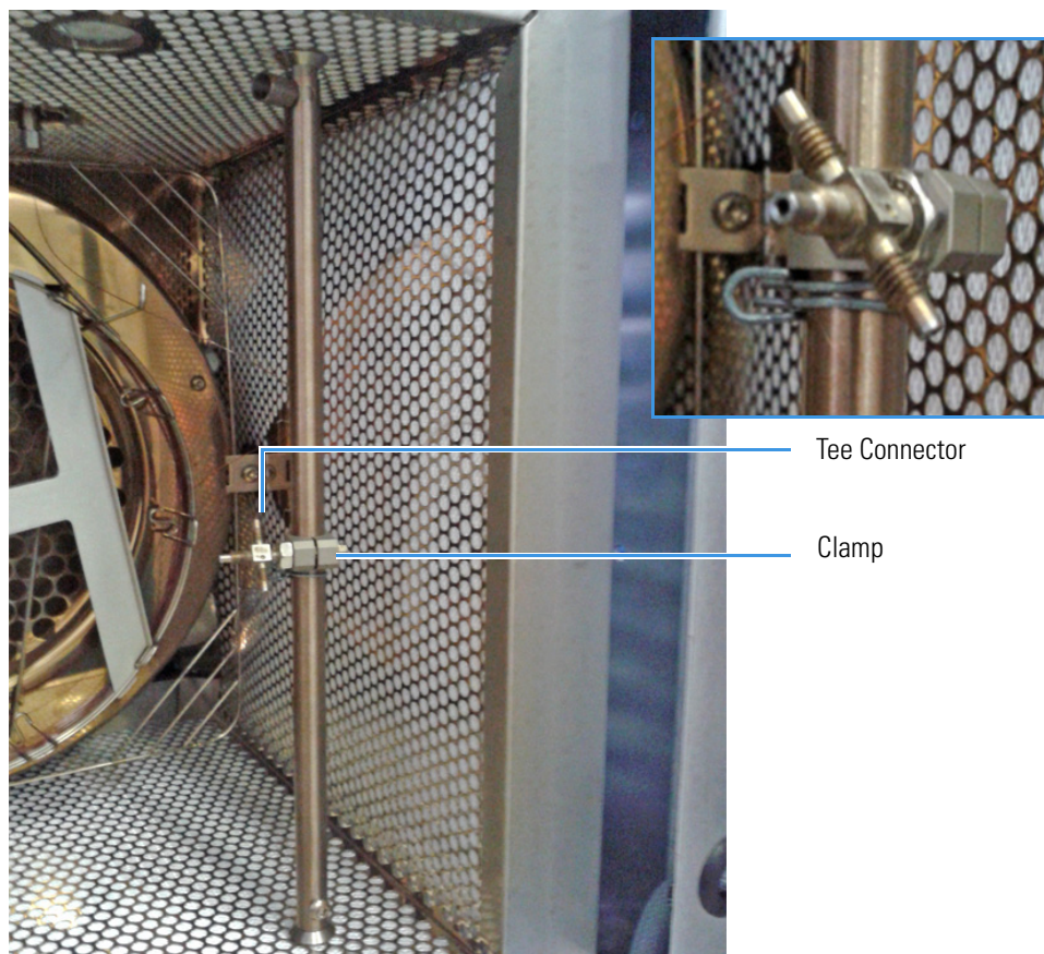
Figure 370. Mounting Bracket Installed in the GC
