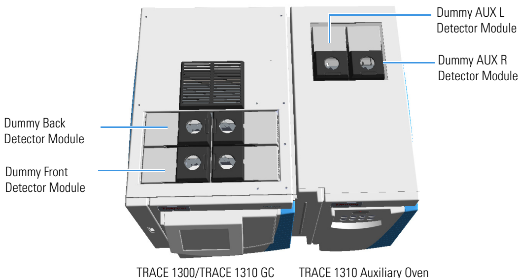
Figure 527. Add a Front/Back/Aux L/Aux R Detector Module
