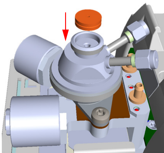
Figure 419. Hot Injection Adapter (2)
