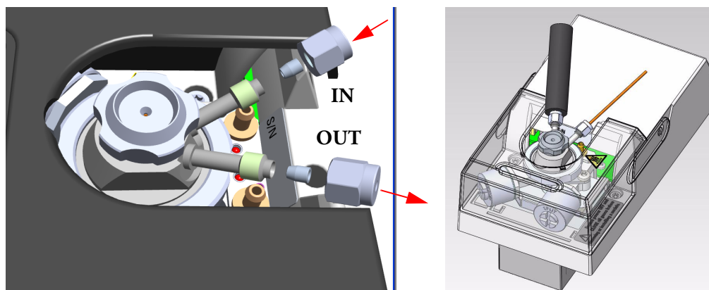
Figure 341. Purge & Trap Adapter (6)
