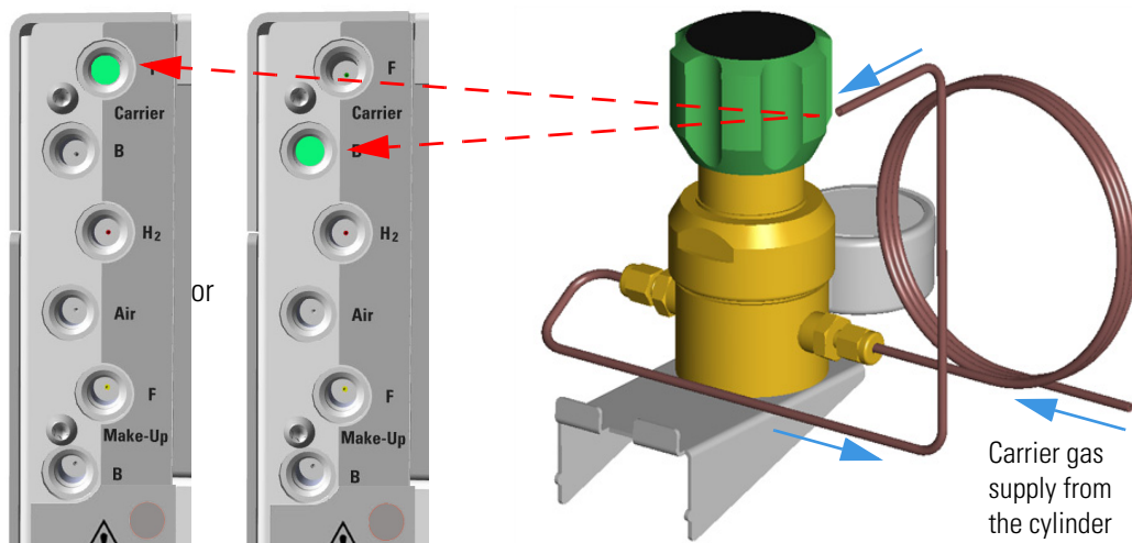
Figure 442. Front or Back Gas Carrier Inlet Connection
