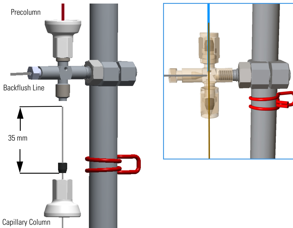
Figure 367. Precolumn and Capillary Column Connection
