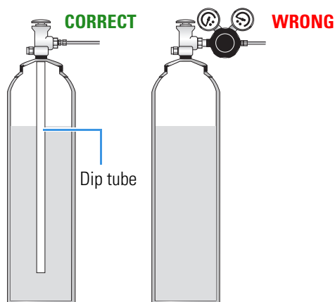
Figure 20. Carbon Dioxide Container
