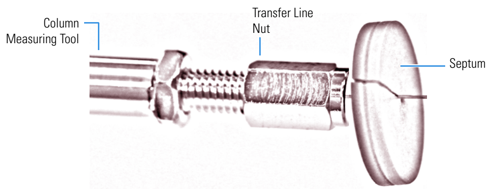
Figure 395. Positioning the Septum
