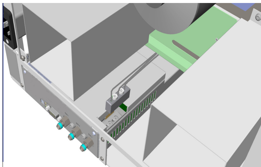
Figure 605. Installation on the Left Side
