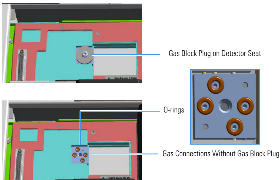
Figure 463. Detector Gas Block Plug
