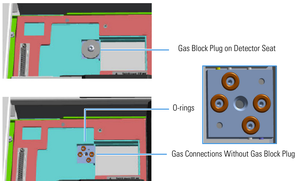
Figure 467. Detector Gas Block Plug
