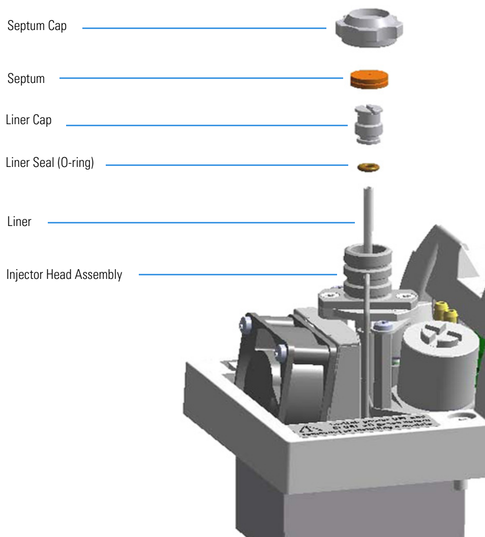
Figure 236. PTVBKF Top Parts and Liner Removal
