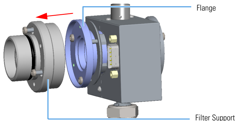
Figure 293. Filter-side Heat Shield Removal (1)
