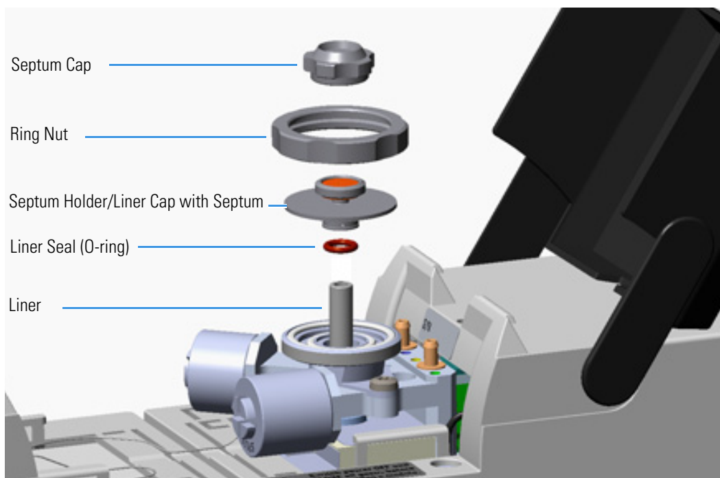
Figure 102. HeS-S/SL Injector: Glass Liner Replacement
