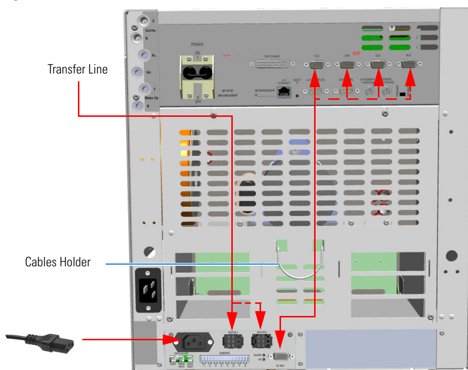
Figure 646. Electrical Connections
