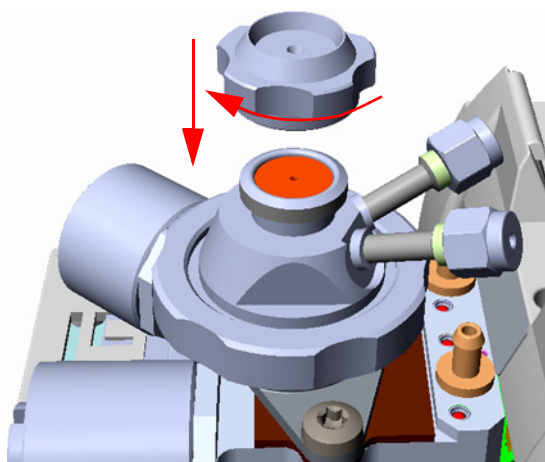
Figure 421. Hot Injection Adapter (4)
