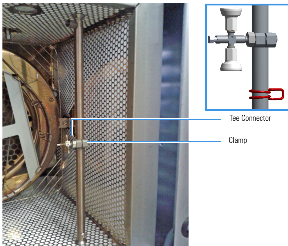
Figure 365. Mounting Bracket Installed in the GC
