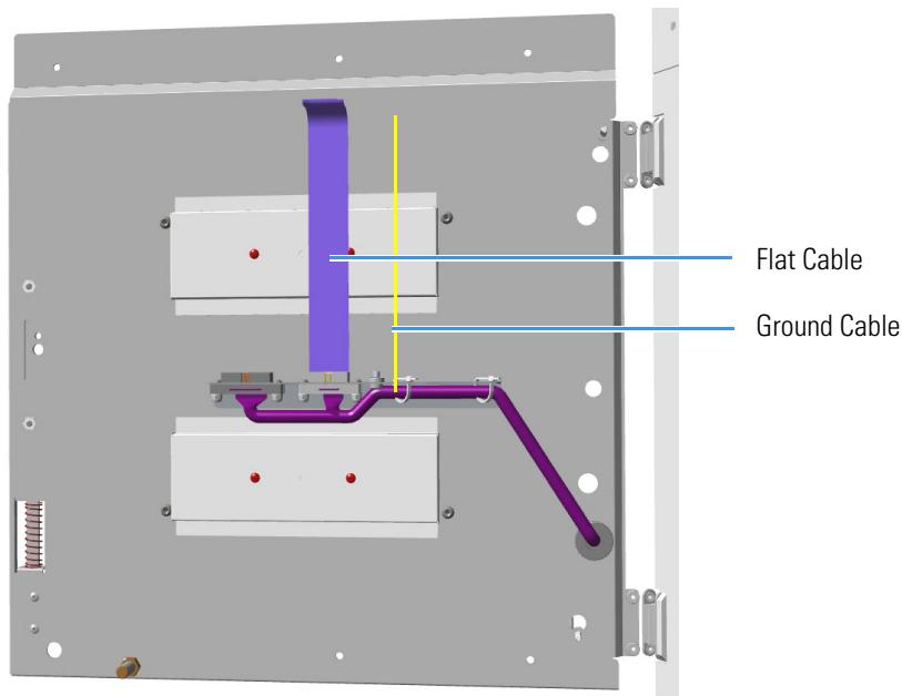
Figure 198. TRACE 1310 Front Door Cables Removal
