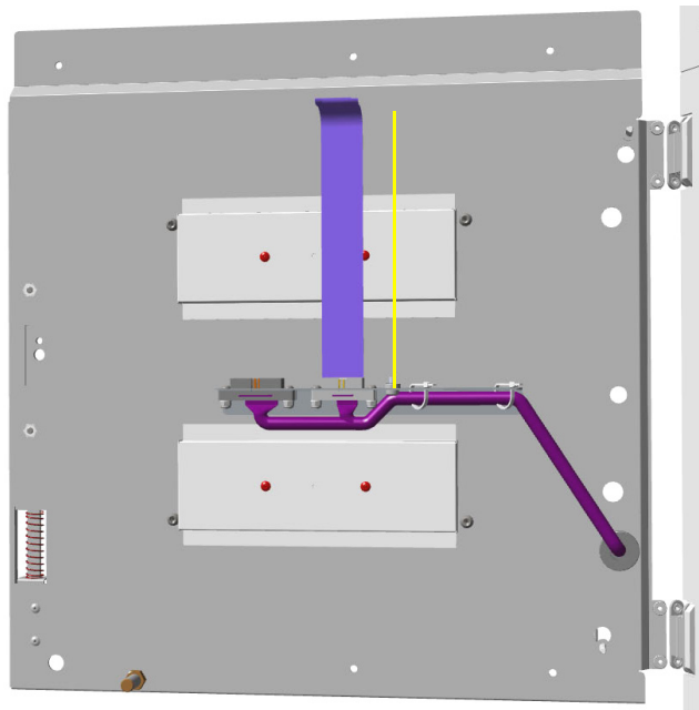
Figure 623. Cables Connections
