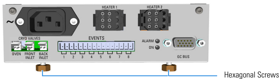
Figure 479. Module Installation (1)
