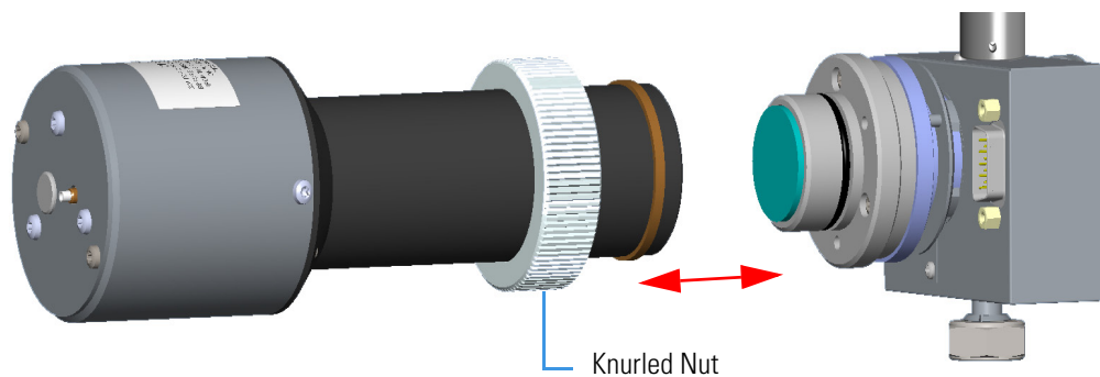
Figure 426. Photomultiplier Assembly Removal
