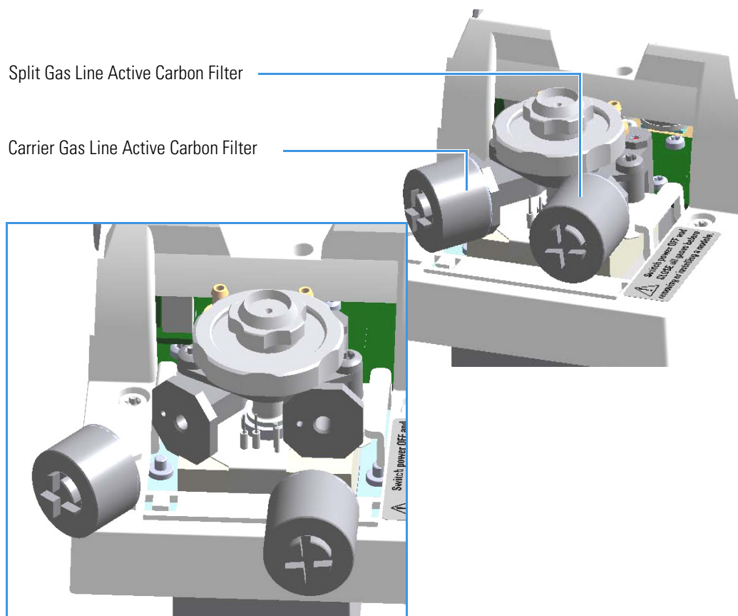
Figure 90. SSLBKF Injector: Active Filters Replacement
