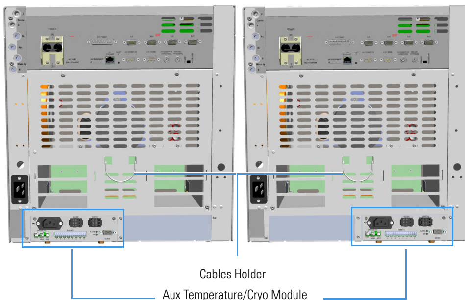
Figure 554. Aux Temperature/Cryo Module Installed into the GC
