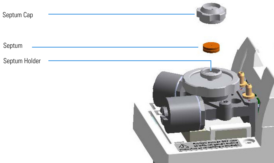
Figure 87. SSLBKF Injector: Septum Replacement
