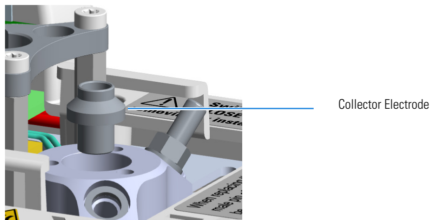
Figure 276. NPD Collecting Electrode Removal
