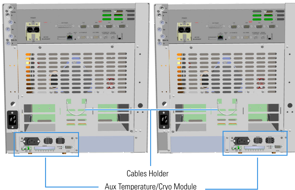
Figure 481. Aux Temperature/Cryo Module Installed into the GC
