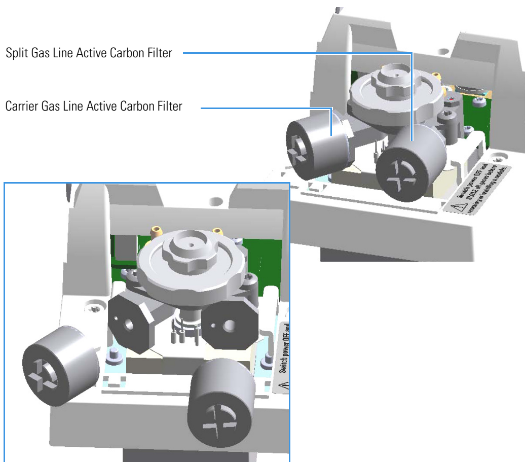
Figure 83. SSL Injector: Active Filters Replacement
