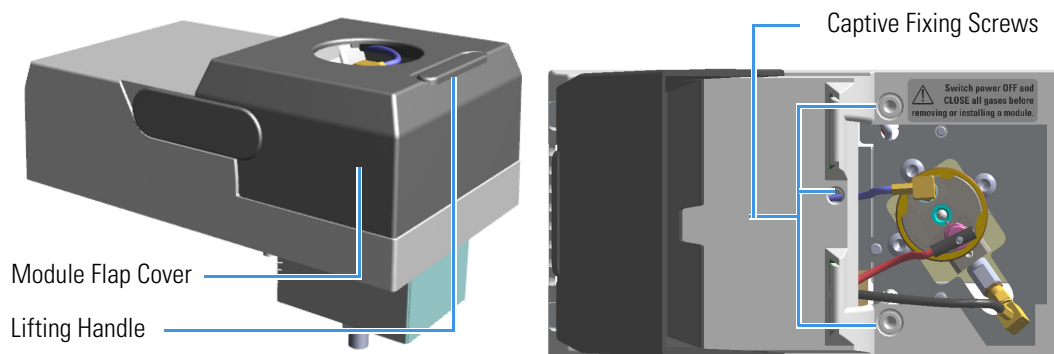
Figure 244. Replacing a Front Detector Module
