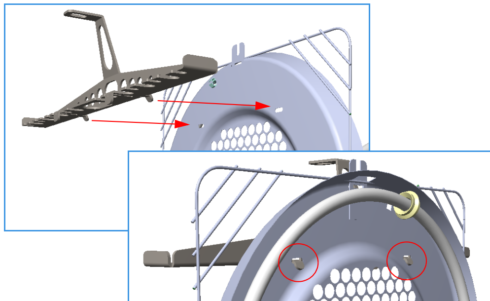
Figure 446. Kit Installation (2)
