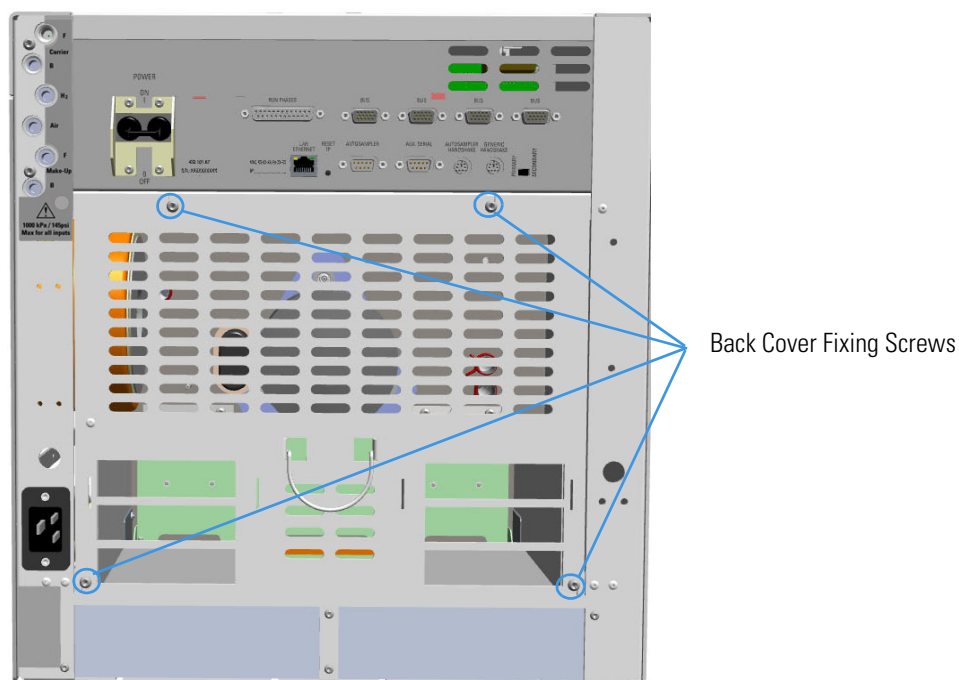
Figure 512. Back Cover Removal
