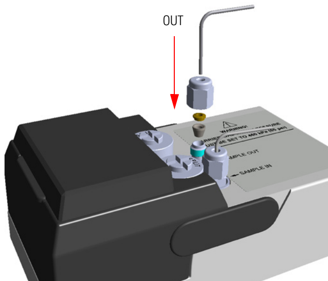
Figure 95. GSV Sample Out Line Connection
