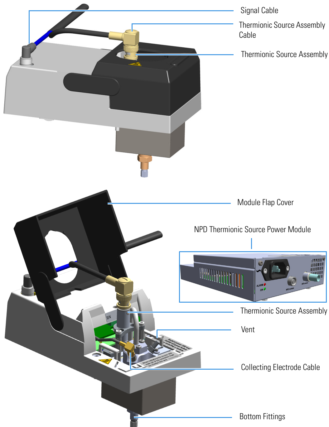
Figure 126. NPD Module Components
