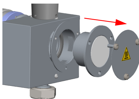
Figure 307. Mirror Plug Removal
