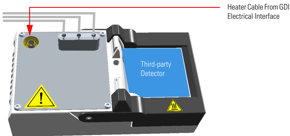
Figure 538. Heater Cable Connection
