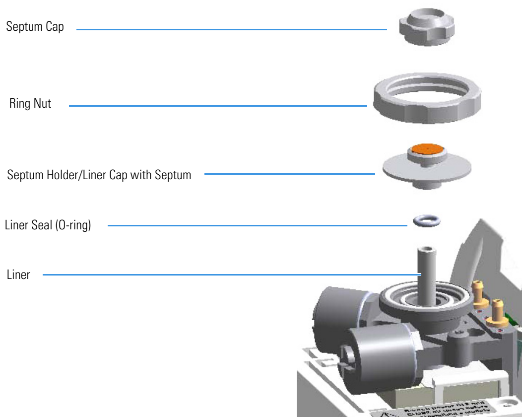
Figure 81. SSL Injector: Glass Liner Replacement
