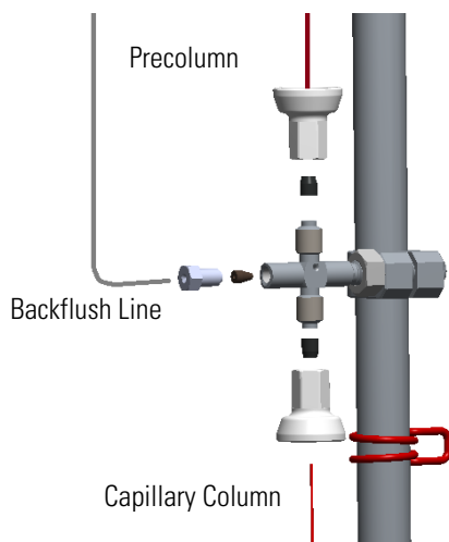
Figure 366. Connecting Backflush Line, Precolumn, and Capillary Column
