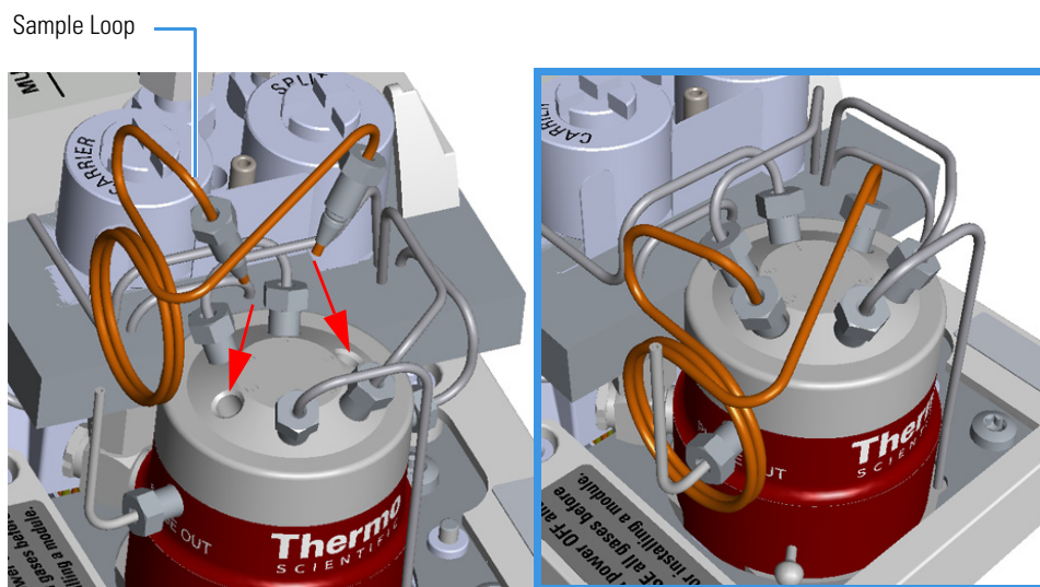
Figure 98. Example of Sample Loop Replacement
