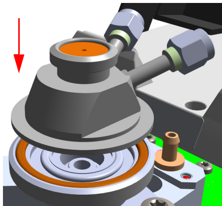
Figure 338. Purge & Trap Adapter (3)
