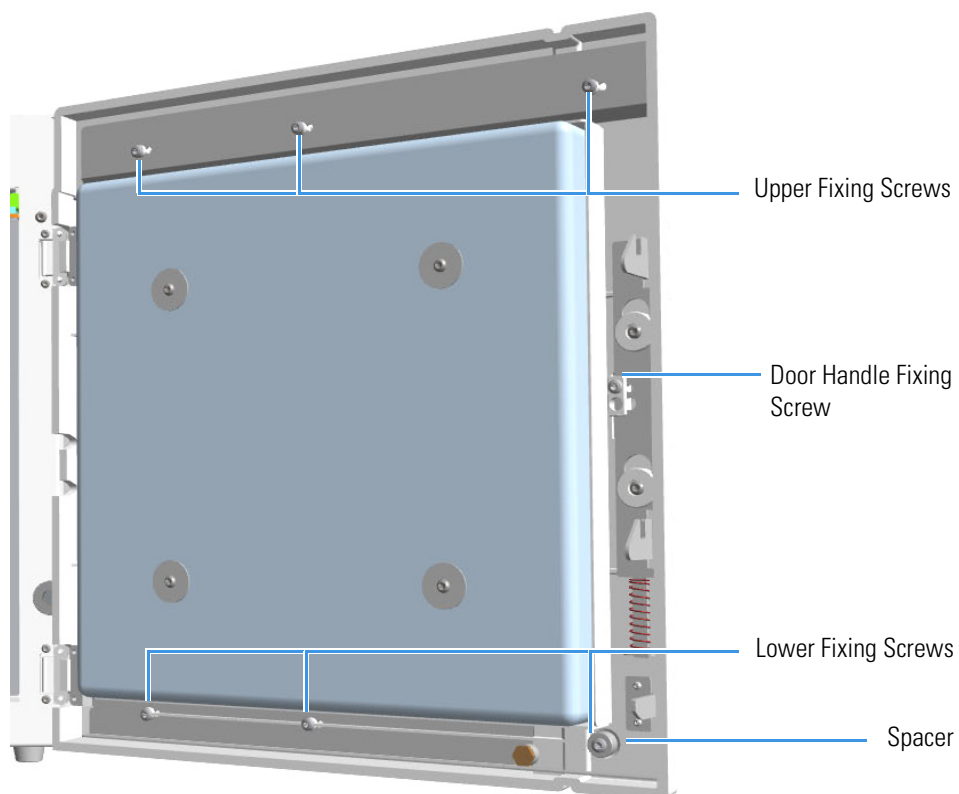
Figure 617. Front Door Back View
