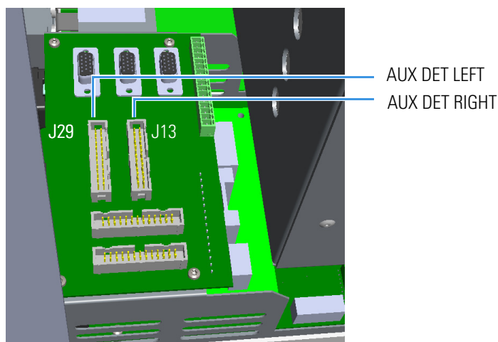
Figure 526. VOBO-HRM Board Layout
