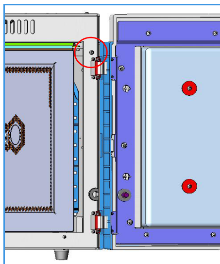
Figure 32. Right Side Panel Fixing Screw
