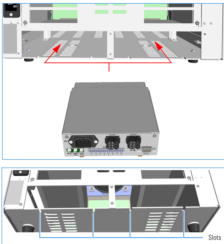
Figure 480. Module Installation (2)
