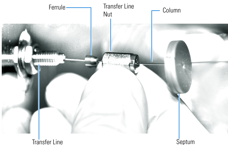
Figure 397. Inserting the Column into the Transfer Line
