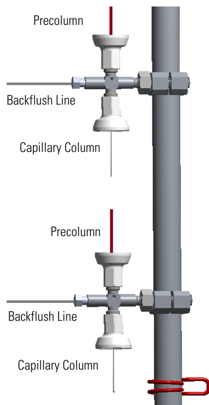
Figure 368. Schematically Connection of a Second Backflush System
