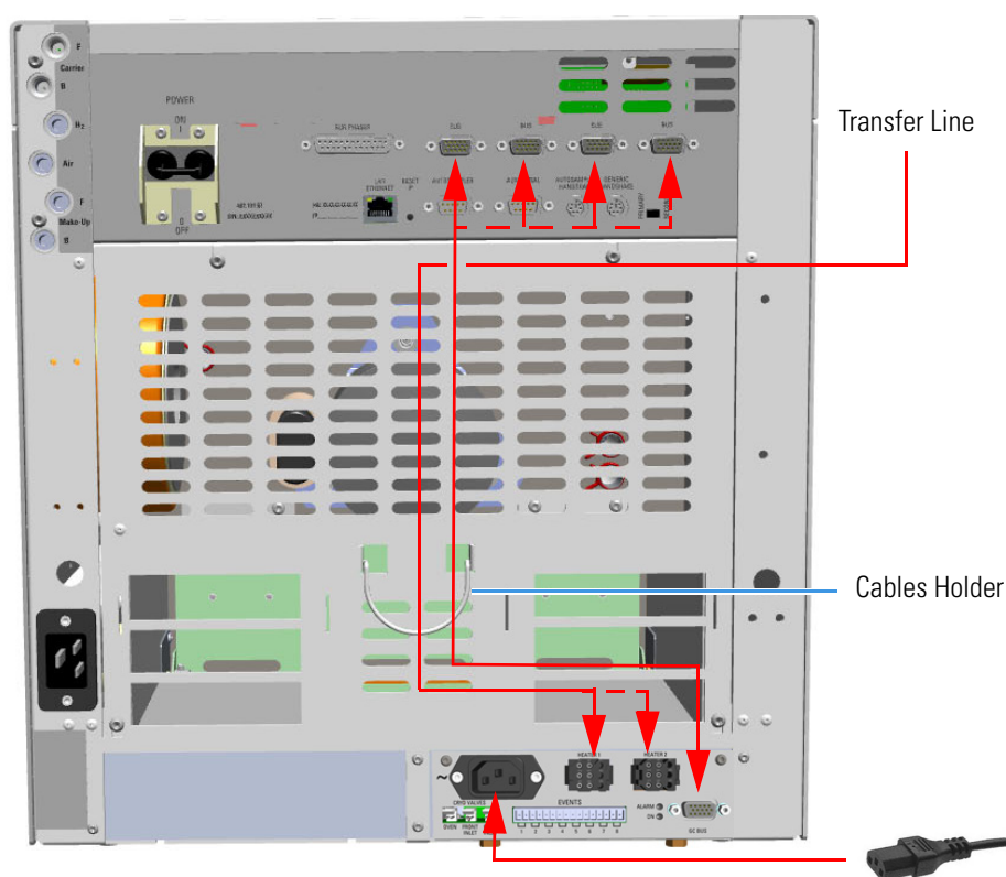
Figure 654. Electrical Connections
