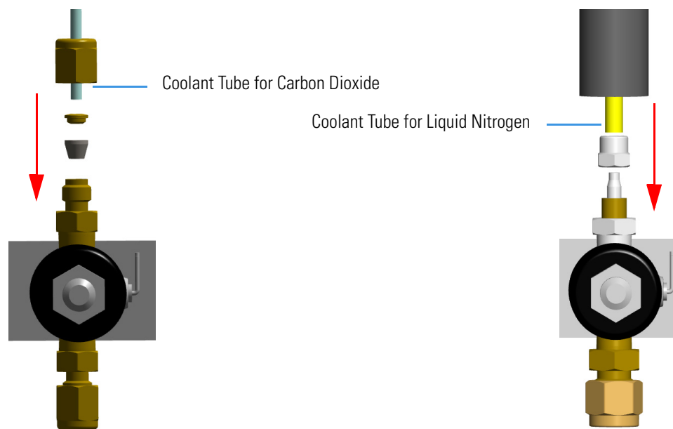
Figure 577. Coolant Tube Connection to the Solenoid Valve
