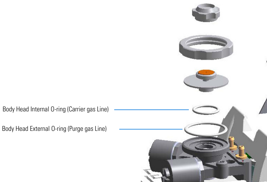
Figure 91. SSLBKF Injector: Body Head O-Rings Replacement
