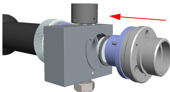
Figure 432. Filter Support and Flange Assembly Installation
