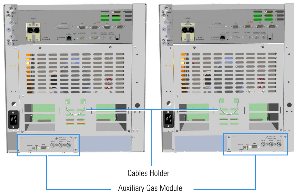
Figure 602. Auxiliary Gas Module Installed into the GC
