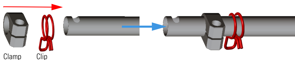
Figure 362. Assembling Tee Connector and Mounting Bracket (2)
