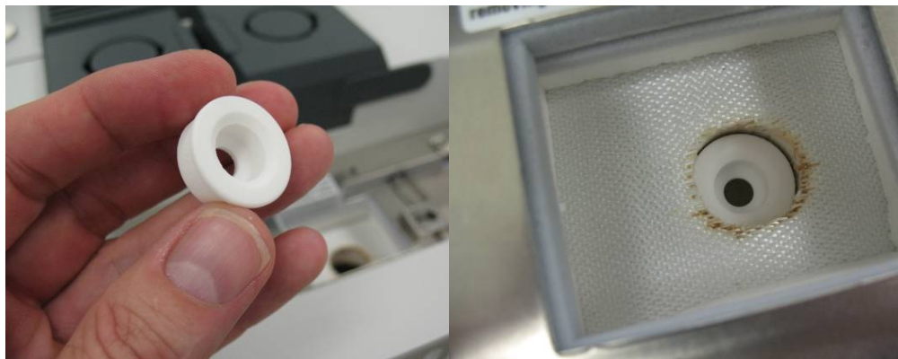
Figure 486. Positioning the Instant Connect Helium Saver Injector Module
