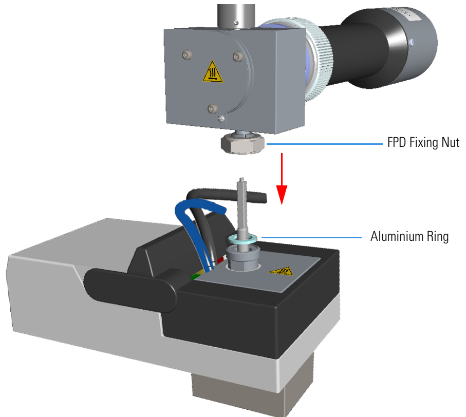
Figure 287. FPD Detector Reinstallation
