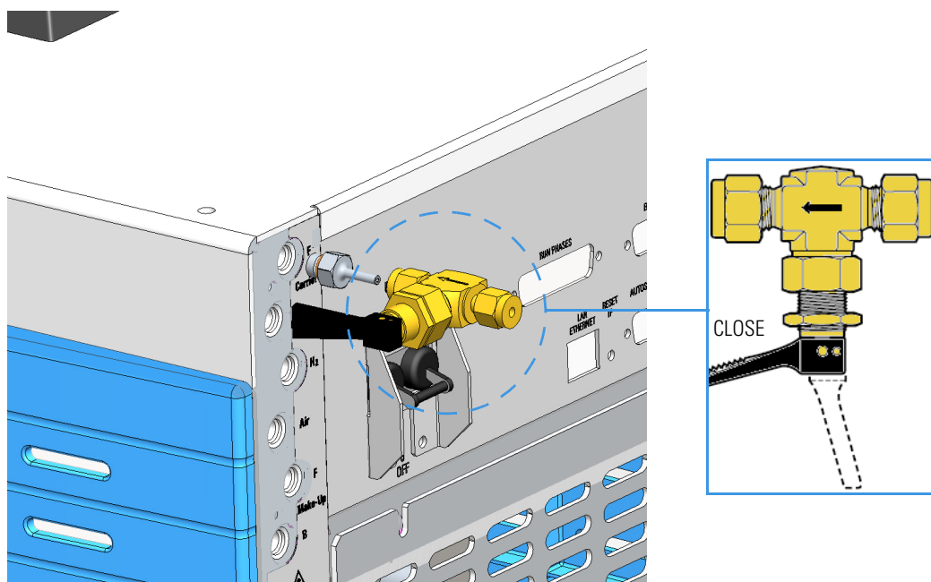
Figure 360. Manual Toggle Valve Installation
