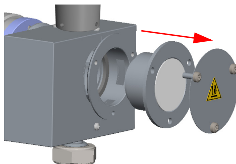
Figure 431. Mirror Plug Removal
