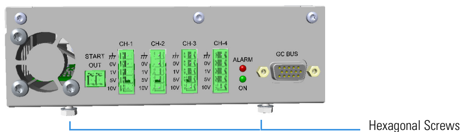
Figure 541. AOI Installation (1)
