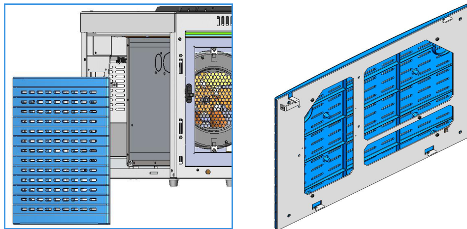
Figure 550. Left Panel Removal
