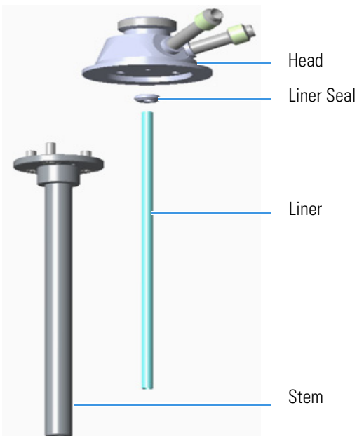
Figure 411. Hot Injector Adapter Assembly
