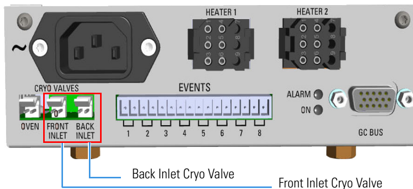
Figure 22. Cryo Valves: Front/Back Inlet
