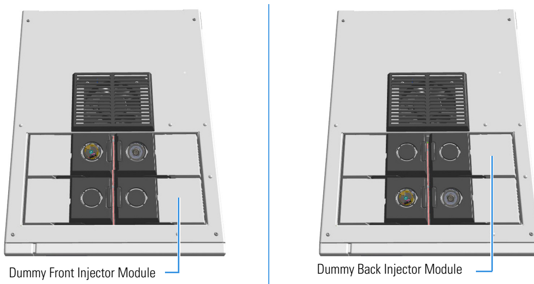
Figure 456. Add a New Front/Back GSV Injector Module
