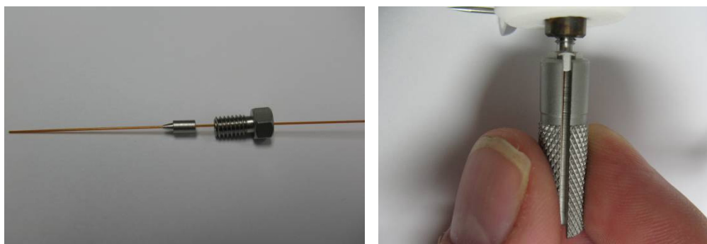
Figure 489. Installing the Column Nut and Ferrule
