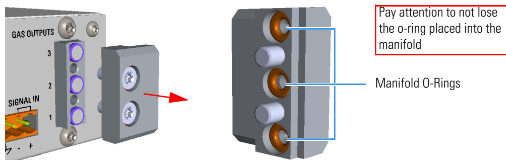
Figure 518. Gas Outputs Manifold
