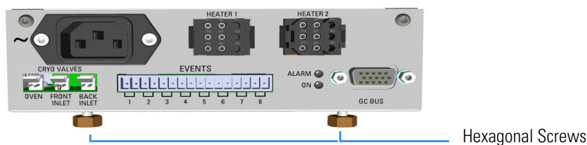
Figure 570. Module Installation (1)
