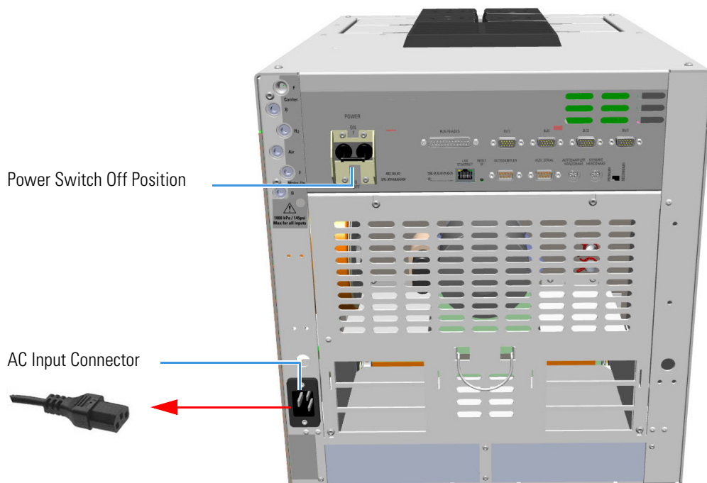
Figure 76. GC Power Off
