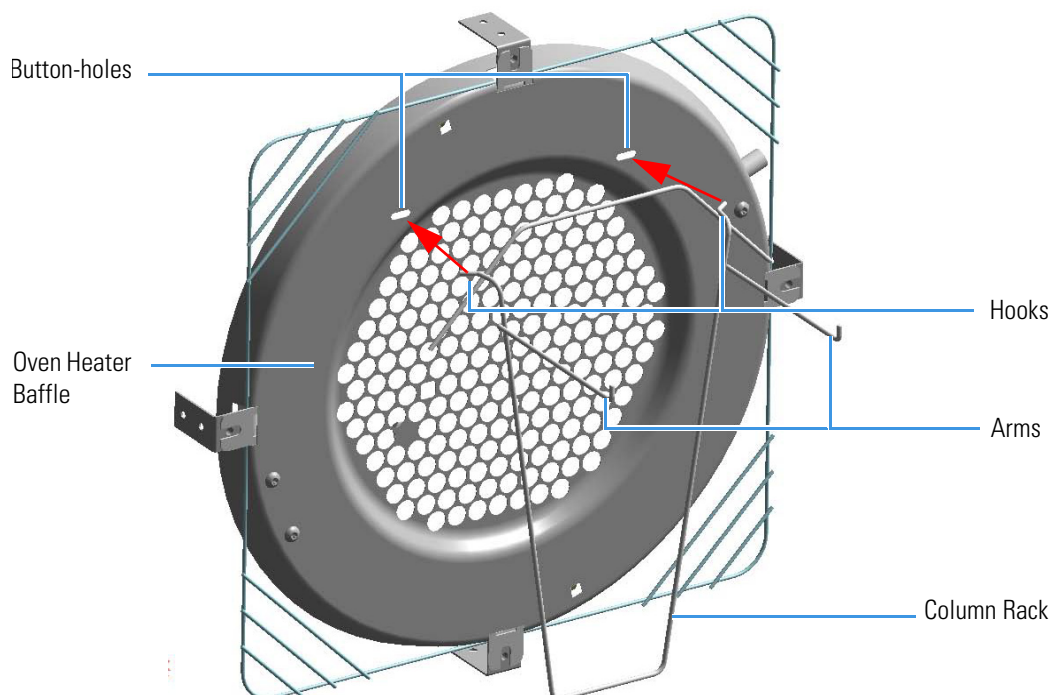
Figure 66. Column Rack
