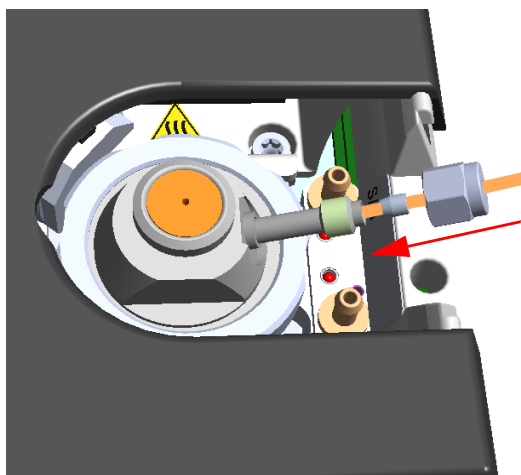
Figure 355. HS Adapter (5)
