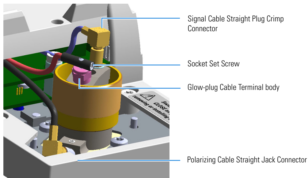
Figure 124. FID Cables Disconnection
