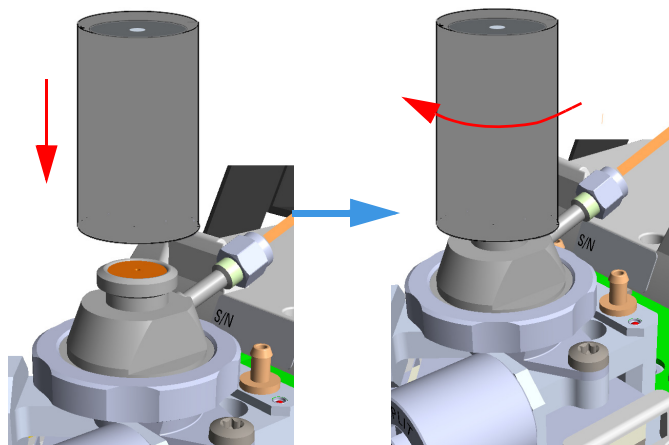
Figure 356. HS Adapter (6)
