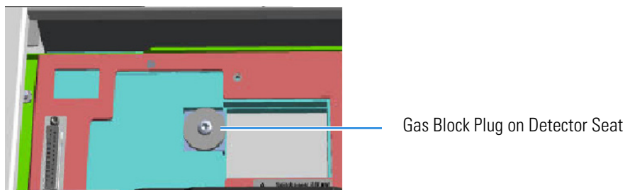
Figure 528. Detector Gas Block Plug (1)
