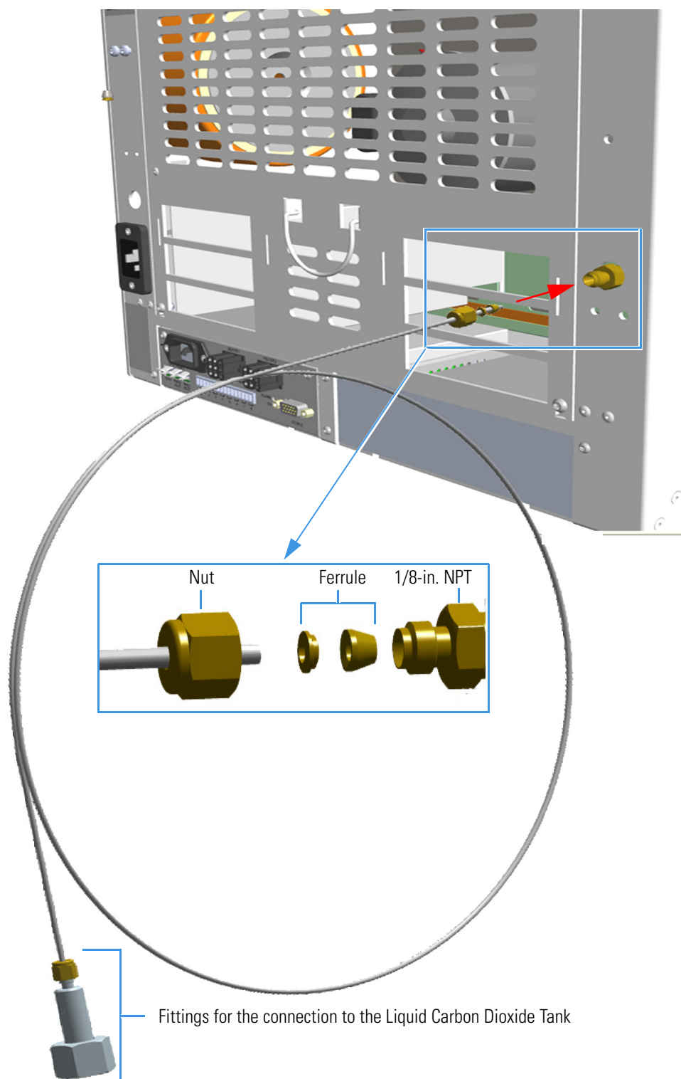
Figure 560. Oven Cryo Supply Tube for Carbon Dioxide Connection
