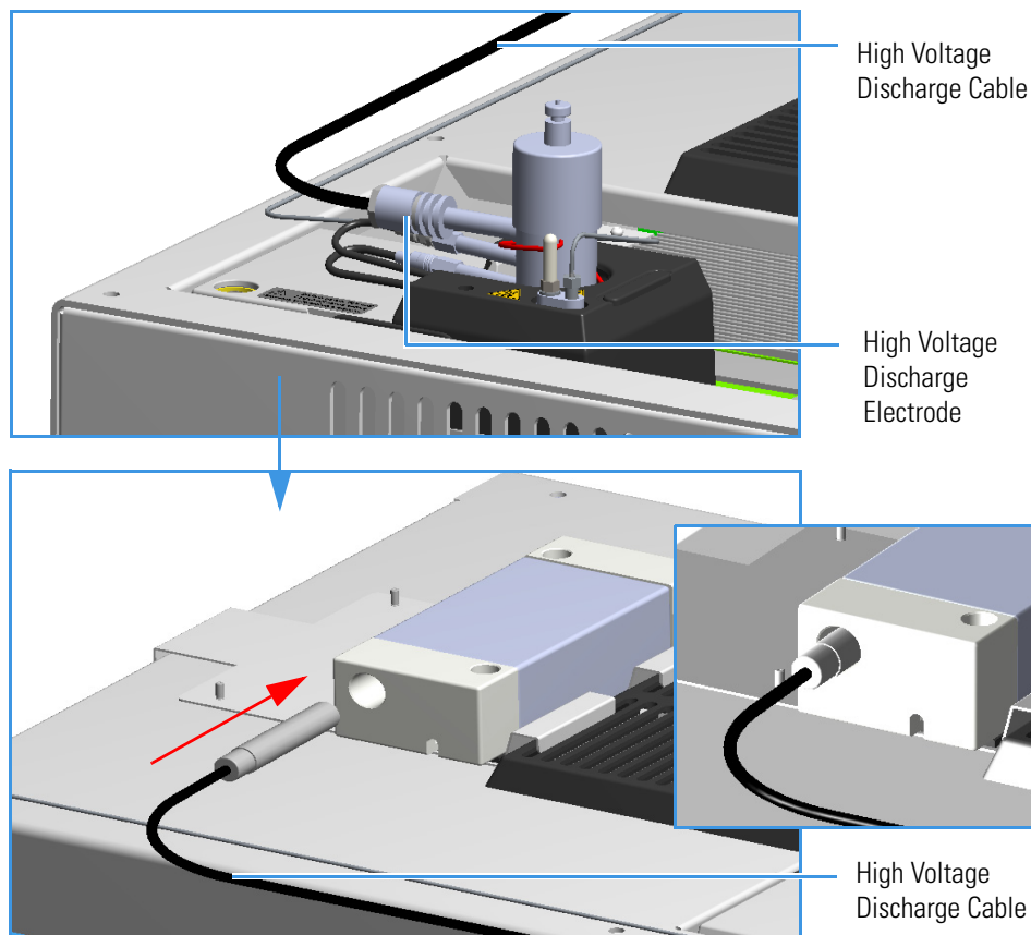
Figure 507. High Voltage Discharge Cable Connection (3)
