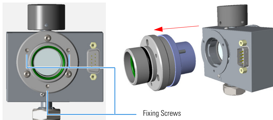
Figure 428. Filter Support and Flange Assembly Removal
