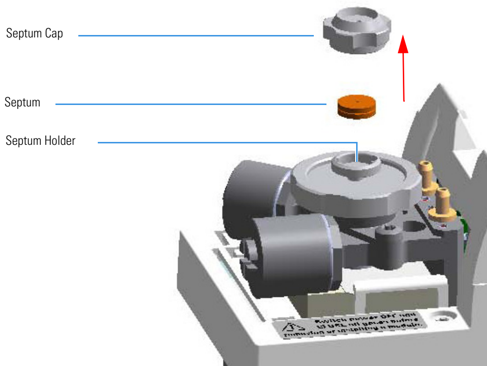
Figure 329. SSL/SSLBKF and HeS-S/SL Injector: Septum Replacement
