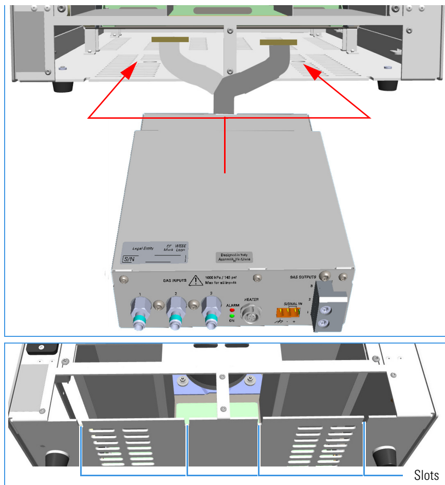
Figure 522. GDI Module Installation (2)
