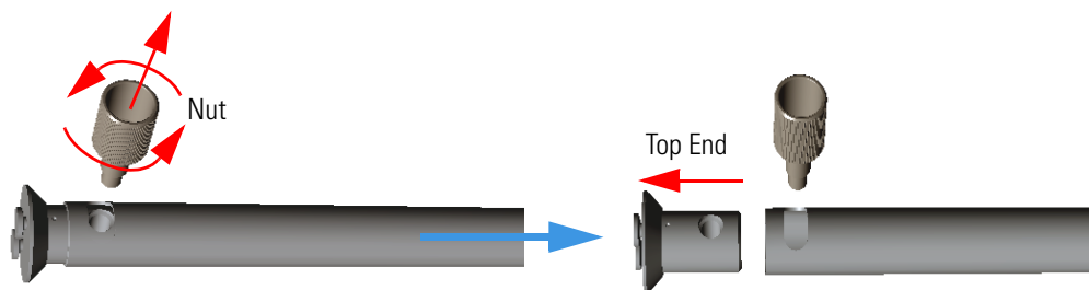
Figure 361. Assembling Tee Connector and Mounting Bracket (1)
