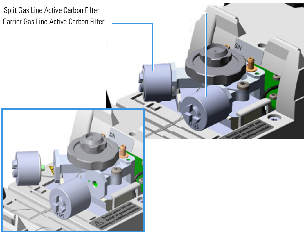
Figure 103. HeS-S/SL Injector: Active Filters Replacement
