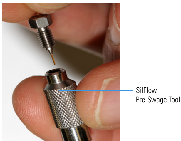
Figure 386. Inserting the Column and Ferrule into the SilFlow Pre-Swage Tool
