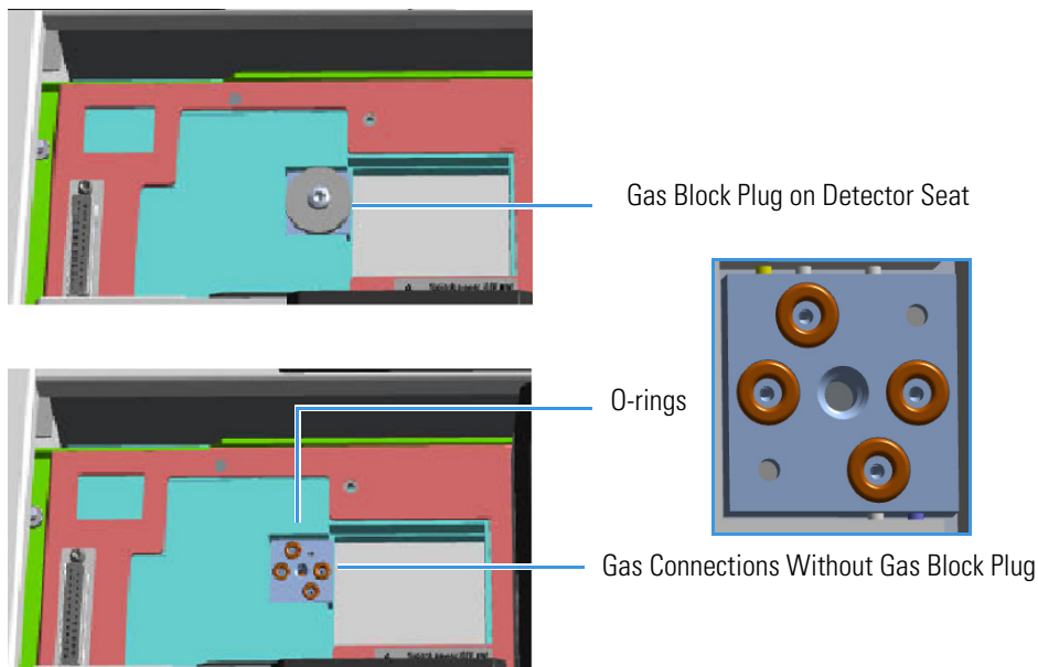
Figure 409. Detector Gas Block Plug
