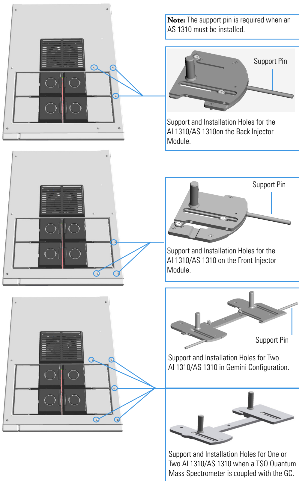
Figure 42. Installation Holes and Sampler Supports for AI/AS 1310 - AI/AS 3000 II Autosampler
