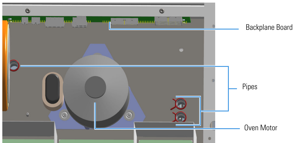
Figure 213. Pipes
