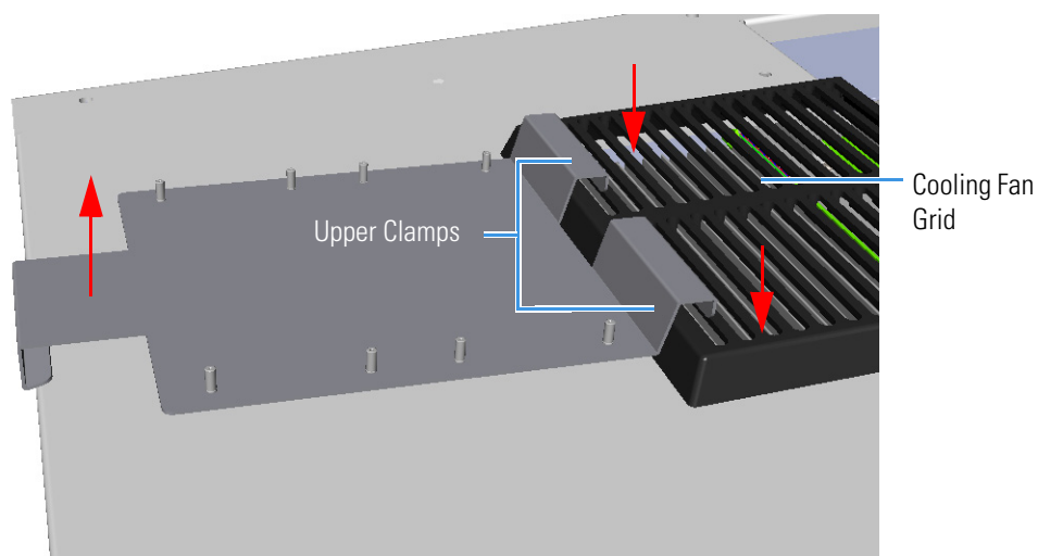
Figure 497. Support Bracket Installation (1)
