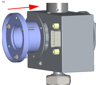
Figure 310. Filter-side Heat Shield Replacement
