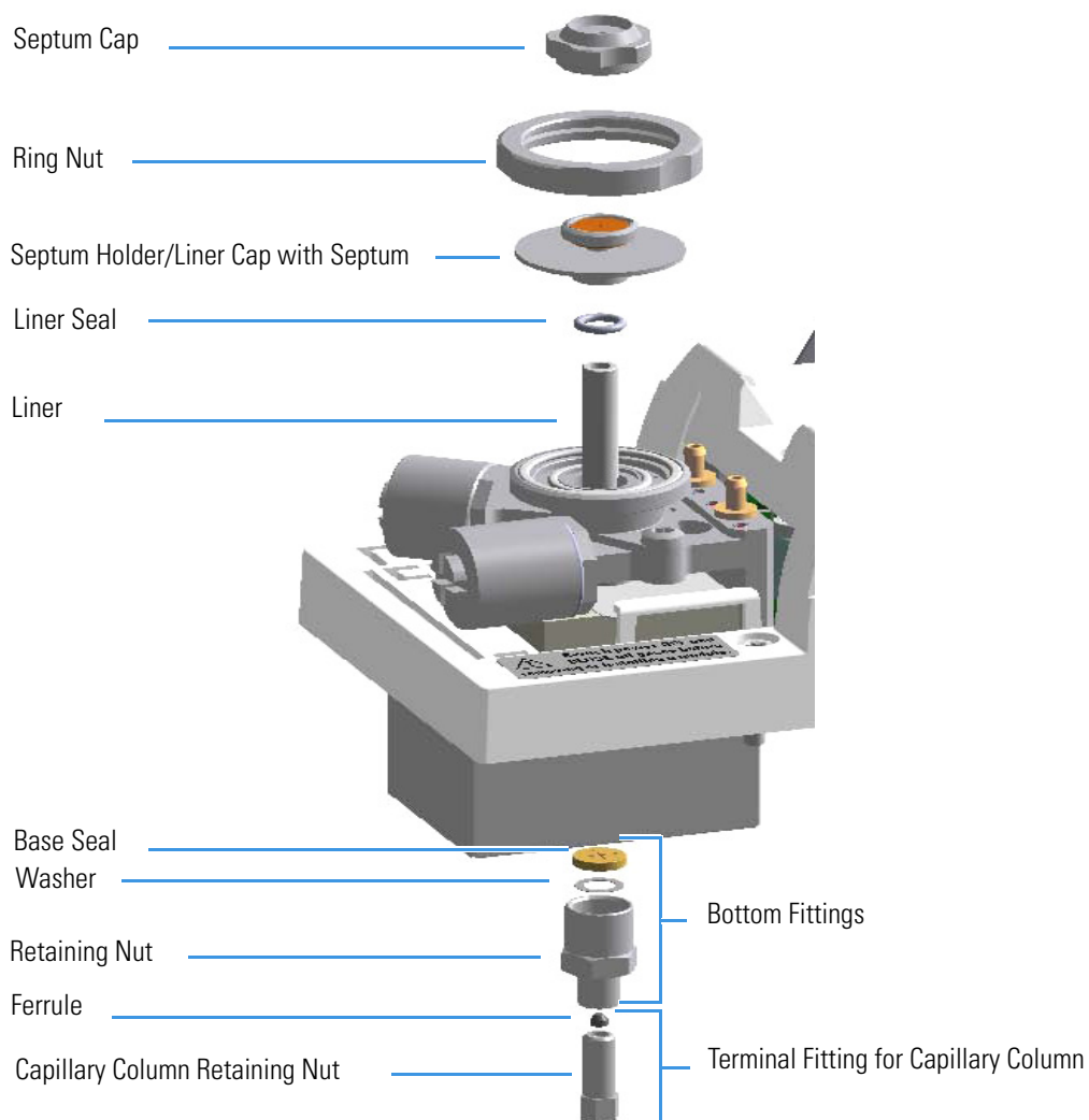
Figure 82. SSL Injector: Broken Liner Replacement
