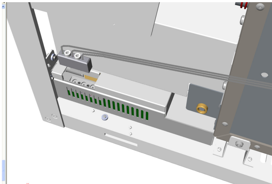
Figure 605. Installation on the Left Side
