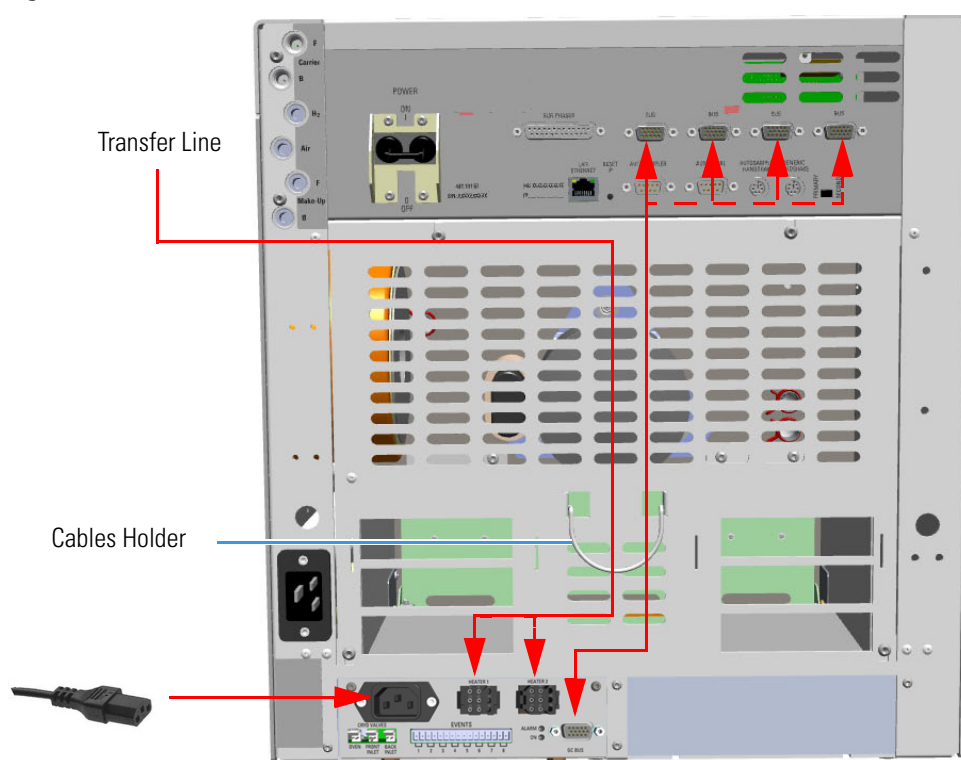
Figure 638. Electrical Connections
