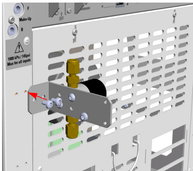
Figure 573. Single Solenoid Valve Assemble Installation
