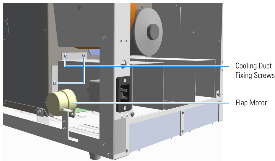
Figure 217. Cooling Duct Removal
