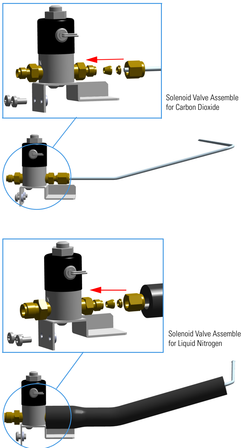
Figure 556. Solenoid Valve Assembly
