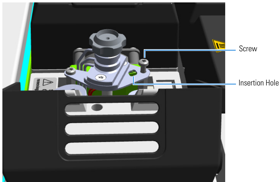
Figure 575. Coolant Tube Insertion Hole
