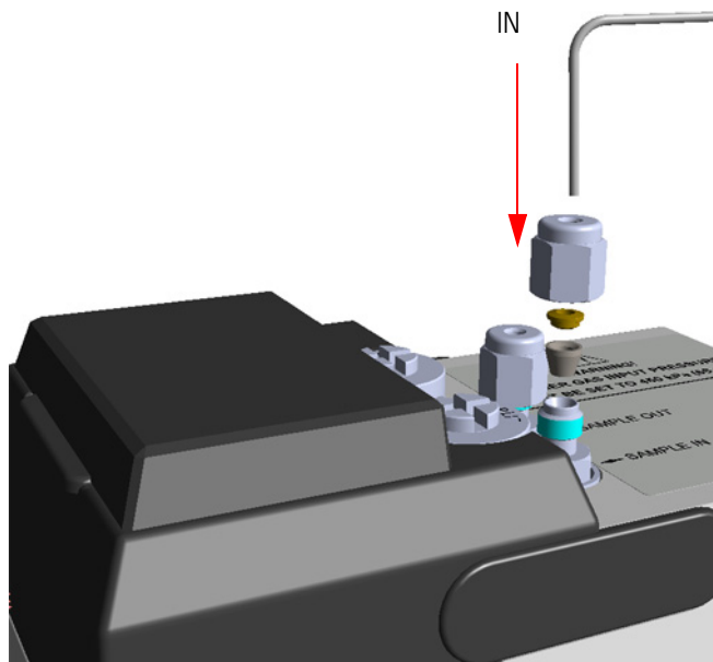
Figure 94. GSV Sample In Line Connection
