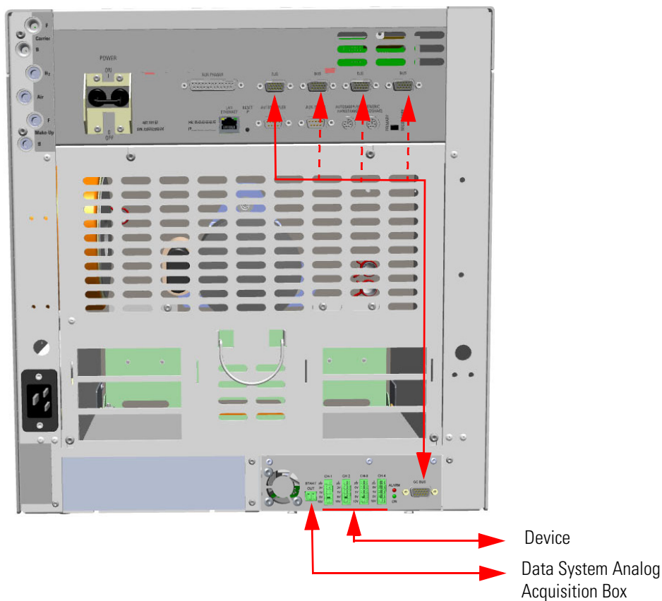
Figure 544. AOI Connections
