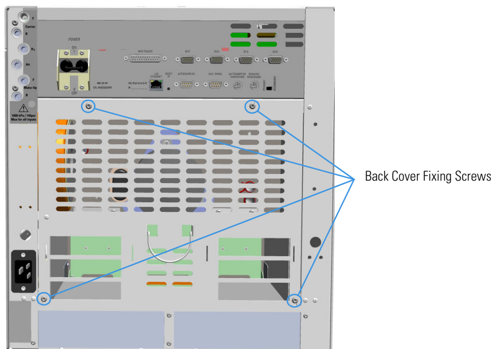
Figure 216. Back Cover Removal
