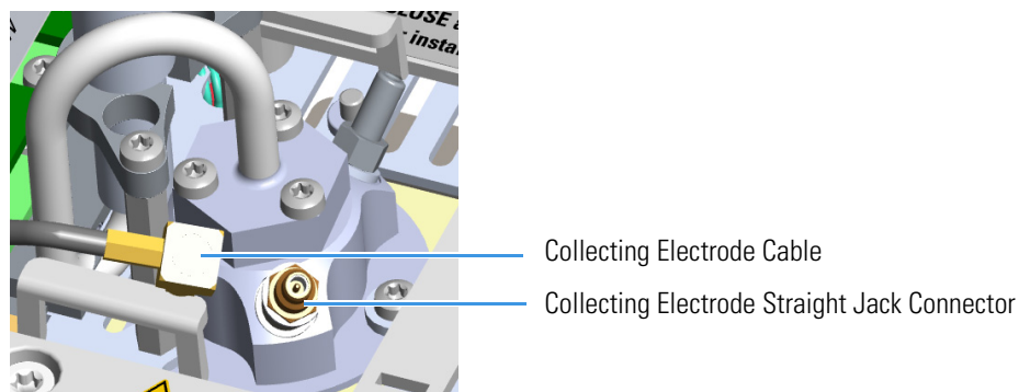
Figure 279. Reinstall Thermionic Source (2)
