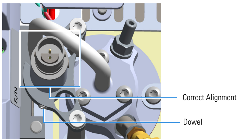
Figure 135. Replace NPD Thermionic Source (1)
