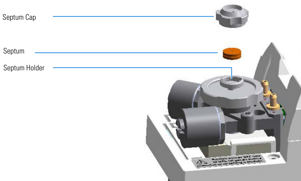
Figure 80. SSL Injector: Septum Replacement
