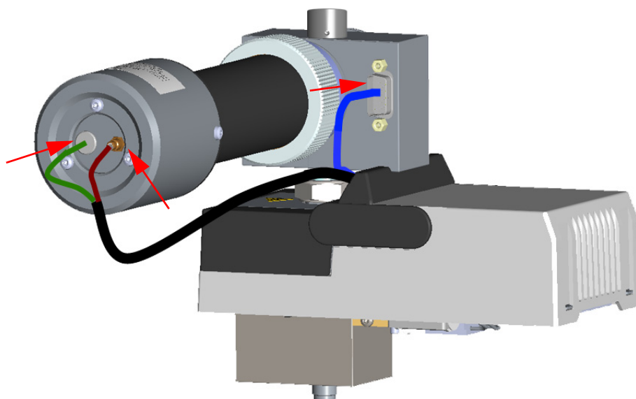
Figure 327. FPD Cables Connection
