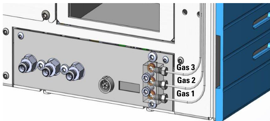
Figure 535. Detector Gas Tubings Connection to the GDI Electrical Interface - External View (2)
