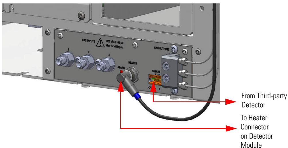
Figure 537. Heater and Signal Connectors
