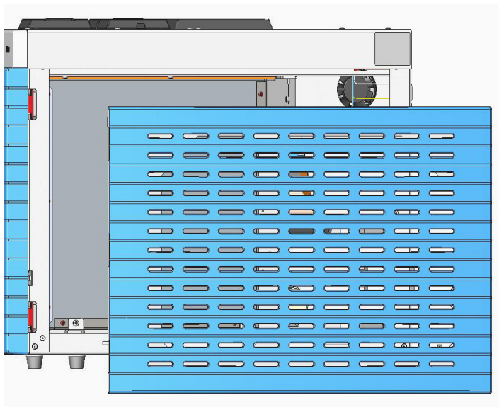
Figure 648. Right Side Panel Removal
