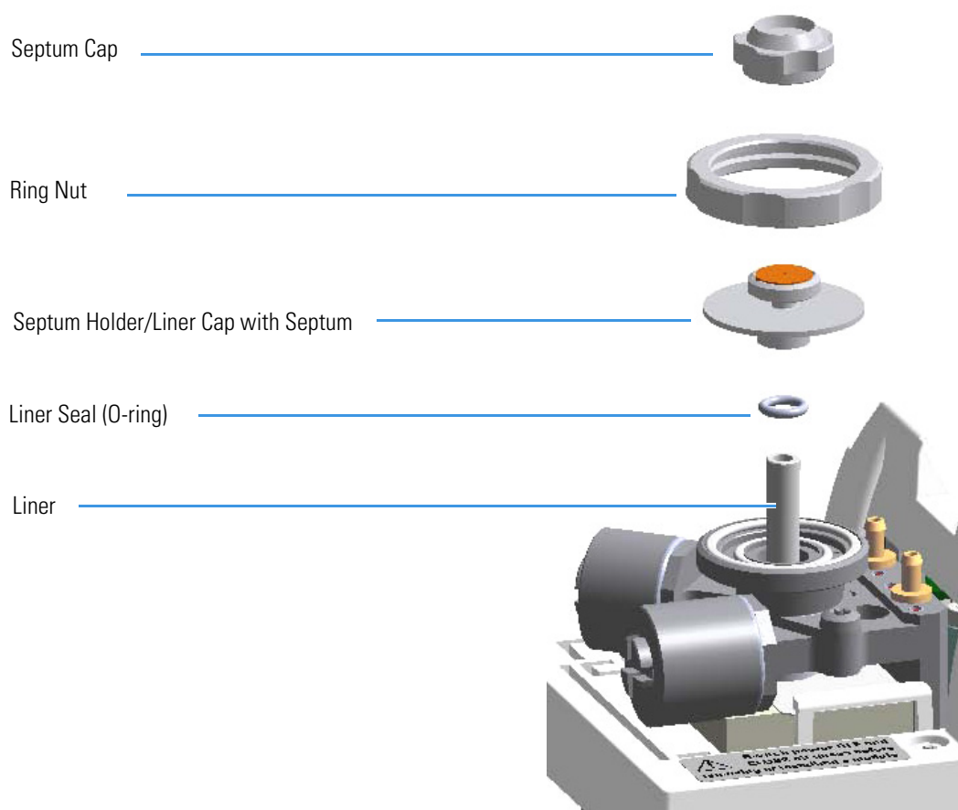
Figure 88. SSLBKF Injector: Glass Liner Replacement
