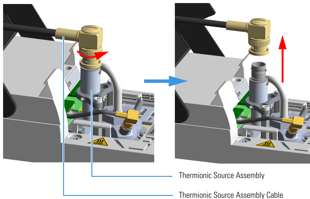
Figure 258. NPD Thermionic Source Cable Removal
