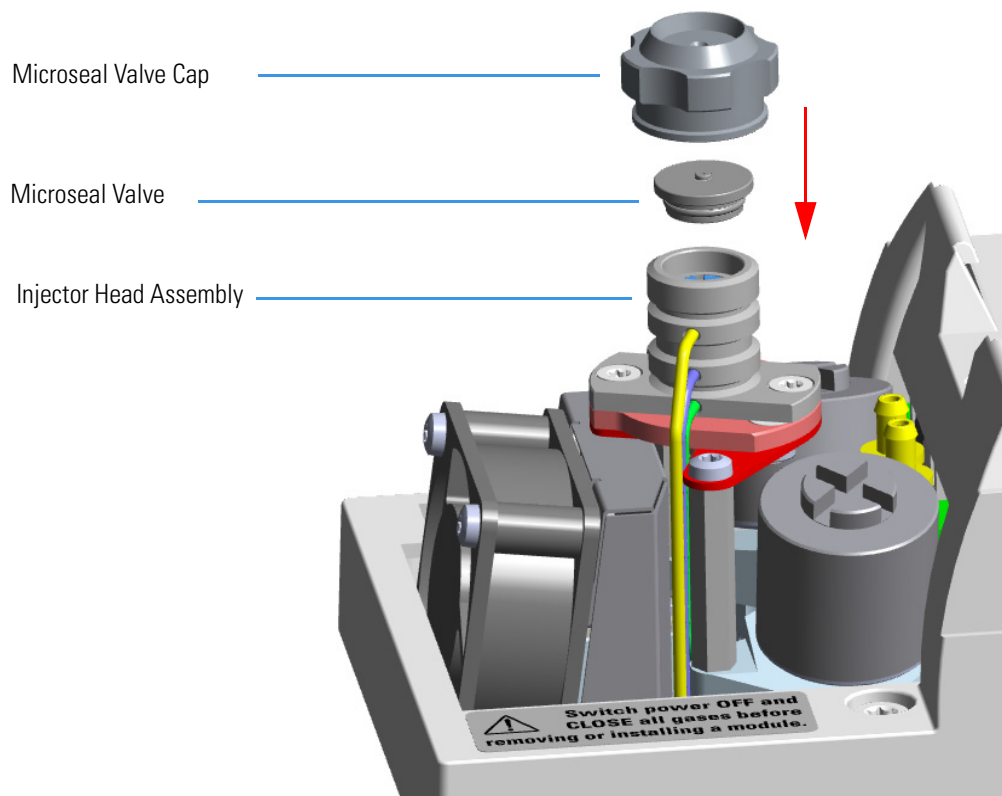
Figure 332. PTV/PTVBKF Injector: Microseal Valve Installation
