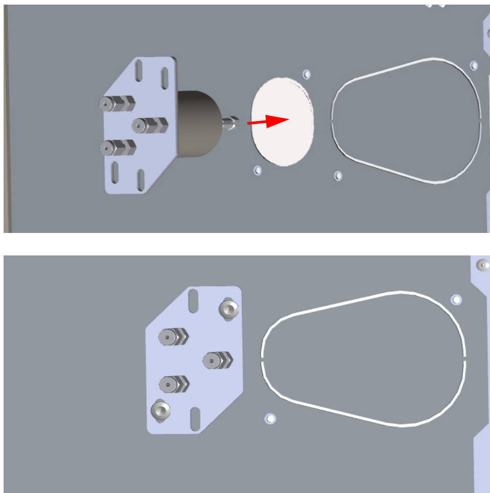
Figure 589. Perform the Duct for the Auxiliary Gas Interface (4)
