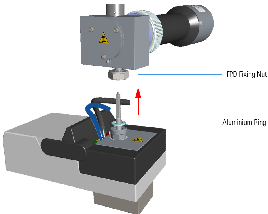
Figure 425. FPD Detector Removal
