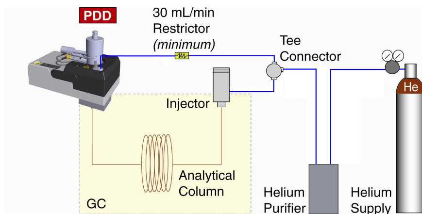
Figure 502. Gas Line Connections
