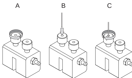
Figure 68. Using a Flowmeter for Leak Check
