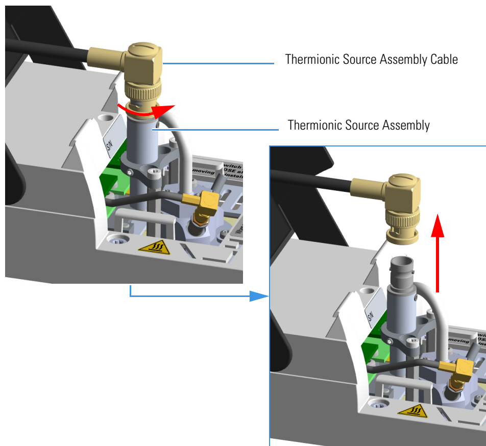
Figure 140. NPD Thermionic Source Cable Removal
