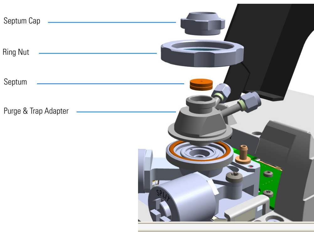
Figure 336. Purge & Trap Adapter (1)
