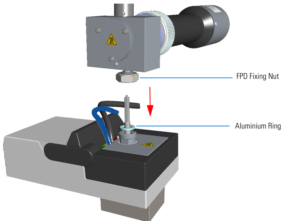
Figure 169. FPD Detector Reinstallation
