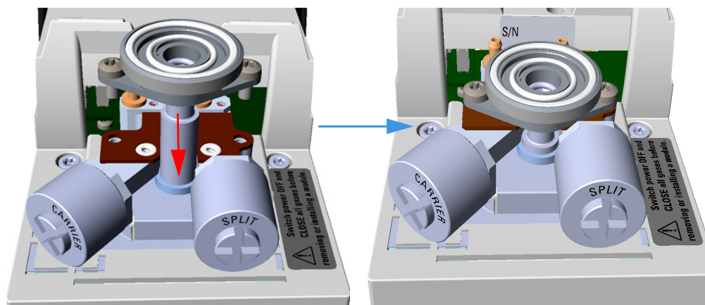
Figure 417. Injector Body Reinstallation
