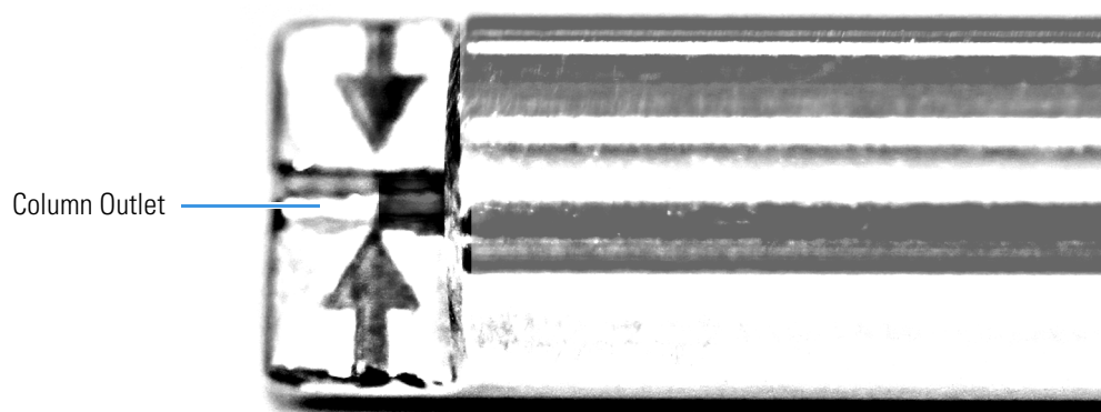
Figure 394. Lining Up the Column in the Column Measuring Tool
