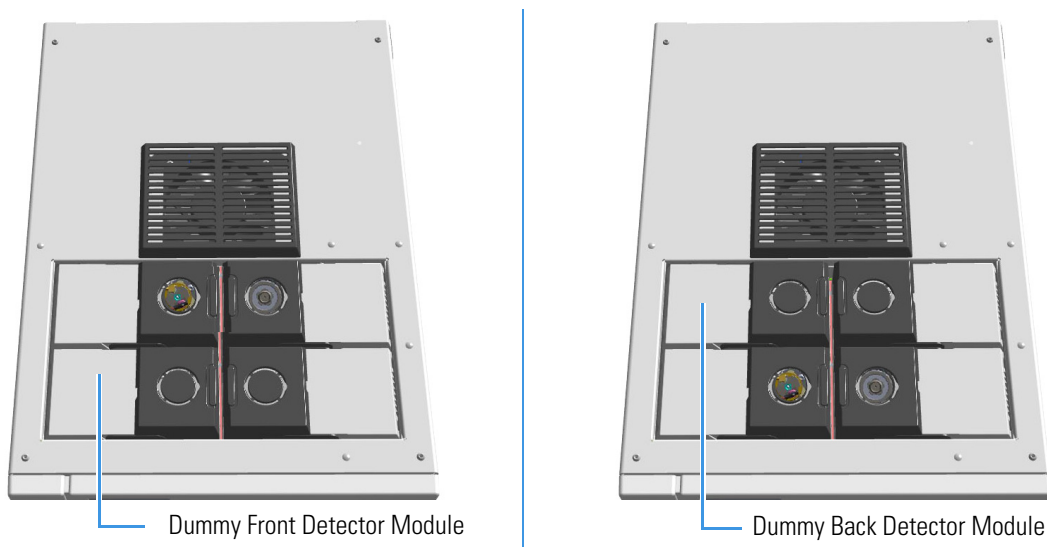
Figure 492. Add a Front/Back Detector Module
