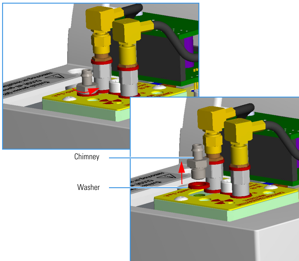
Figure 451. ECD Exhaust Vent Kit Installation (1)
