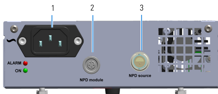
Figure 466. NPD Thermionic Source Power Module Connections
