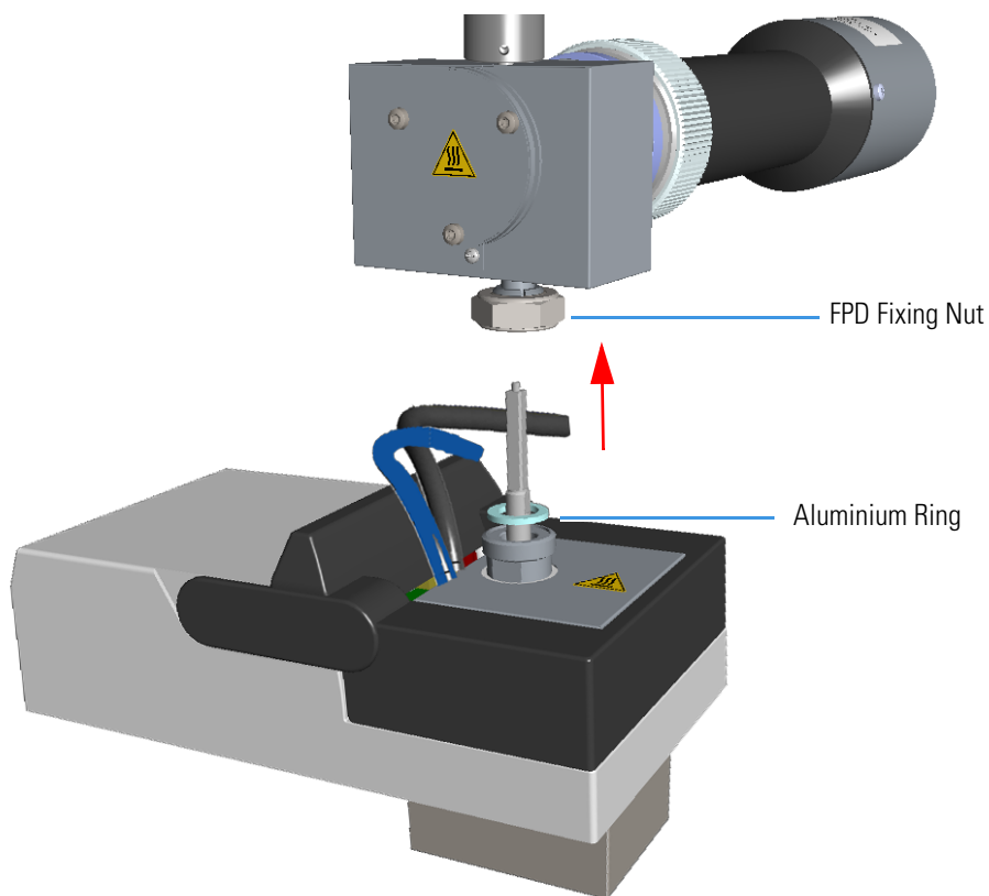
Figure 318. FPD Detector Removal
