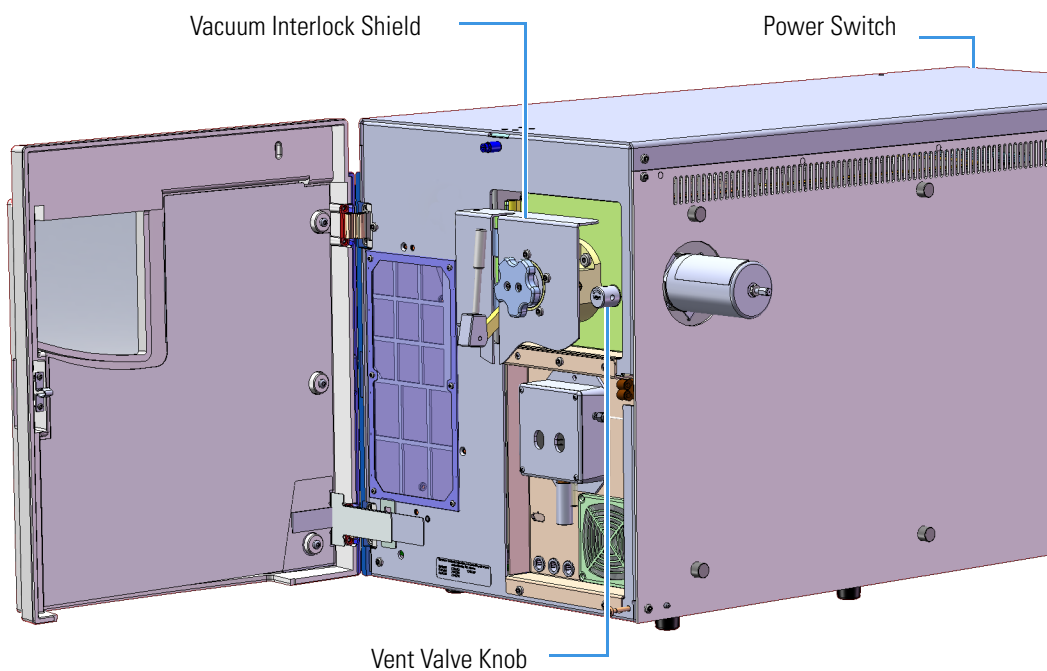
Figure 376. Finding the Vent Valve on the Mass Spectrometer
