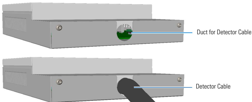
Figure 513. GDI Electrical Interface Back View
