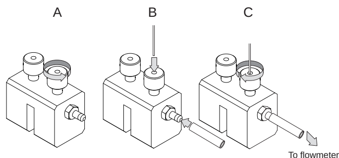
Figure 77. Column Flowmeter Connector
