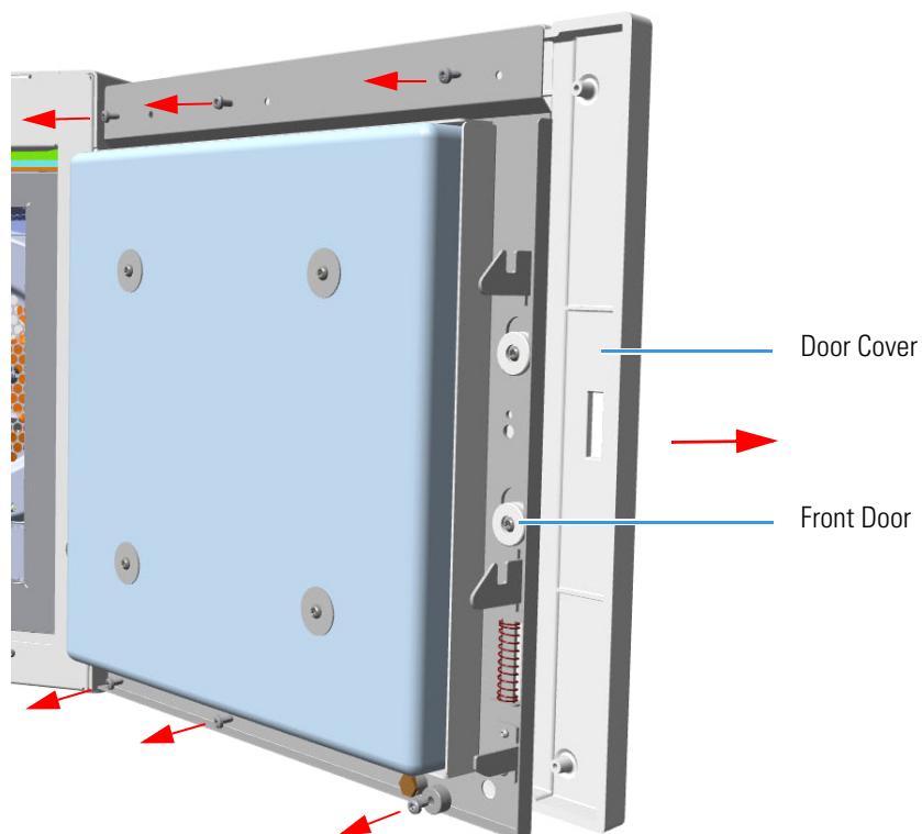
Figure 620. Front Door Removal
