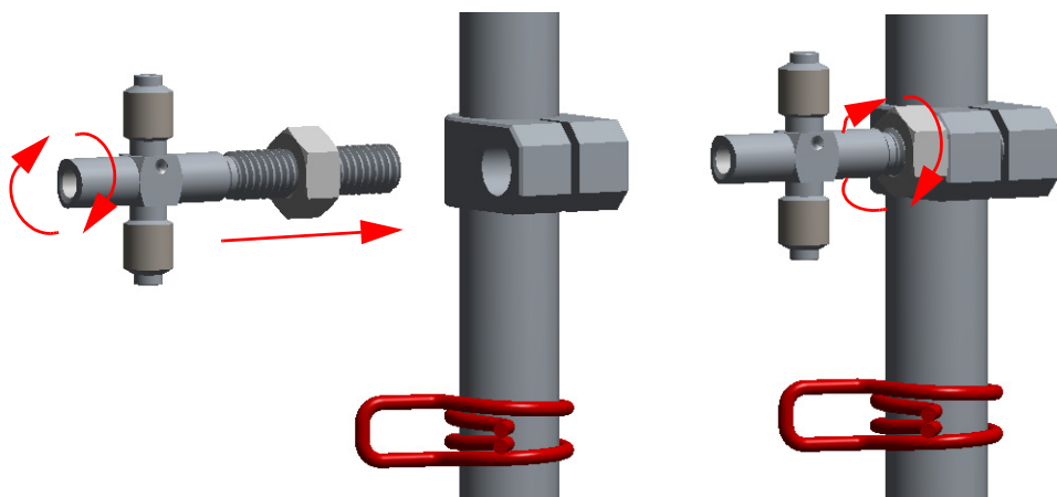
Figure 364. Assembling Tee Connector and Mounting Bracket (4)
