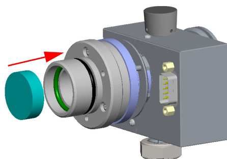
Figure 297. Filter Remounting
