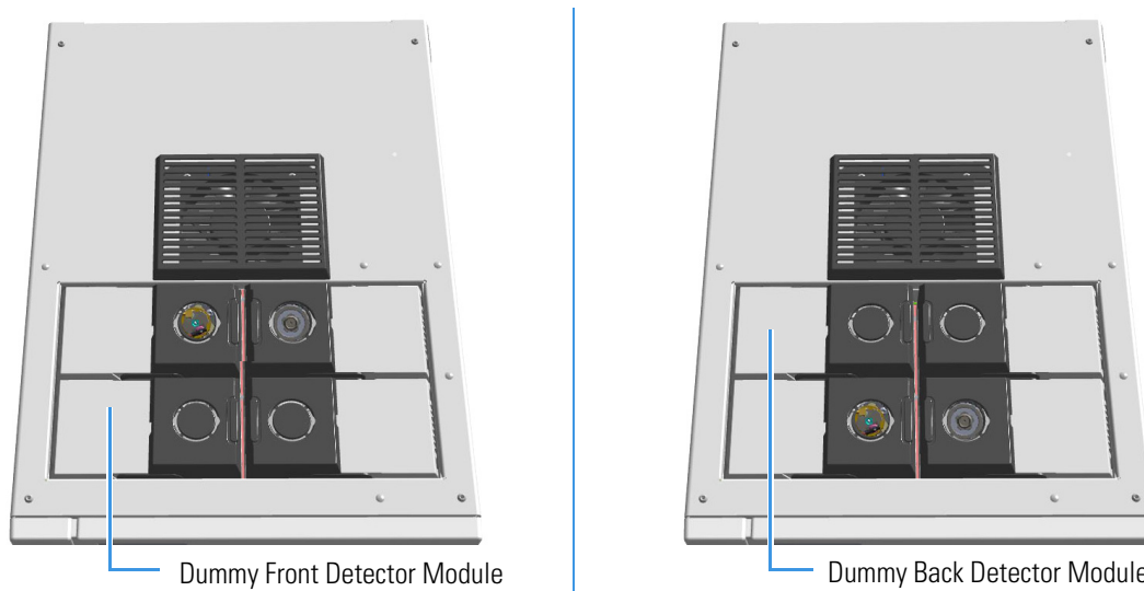
Figure 407. Add a Front/Back Detector Module
