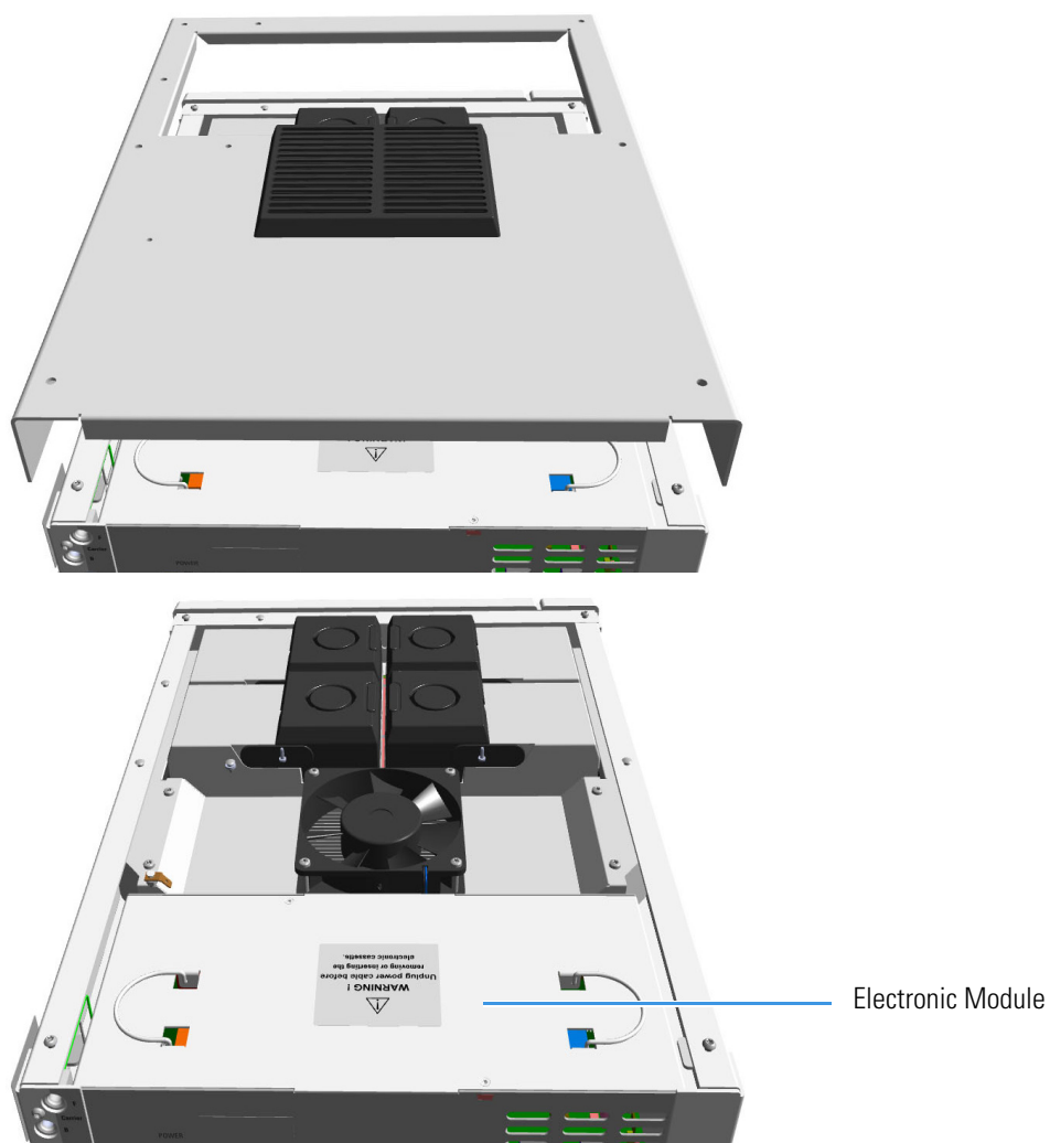
Figure 200. Top Cover Removal (2)
