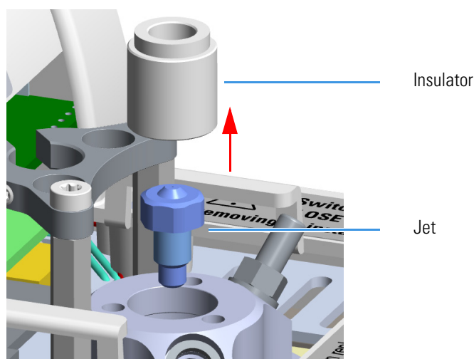
Figure 277. Jet Removal
