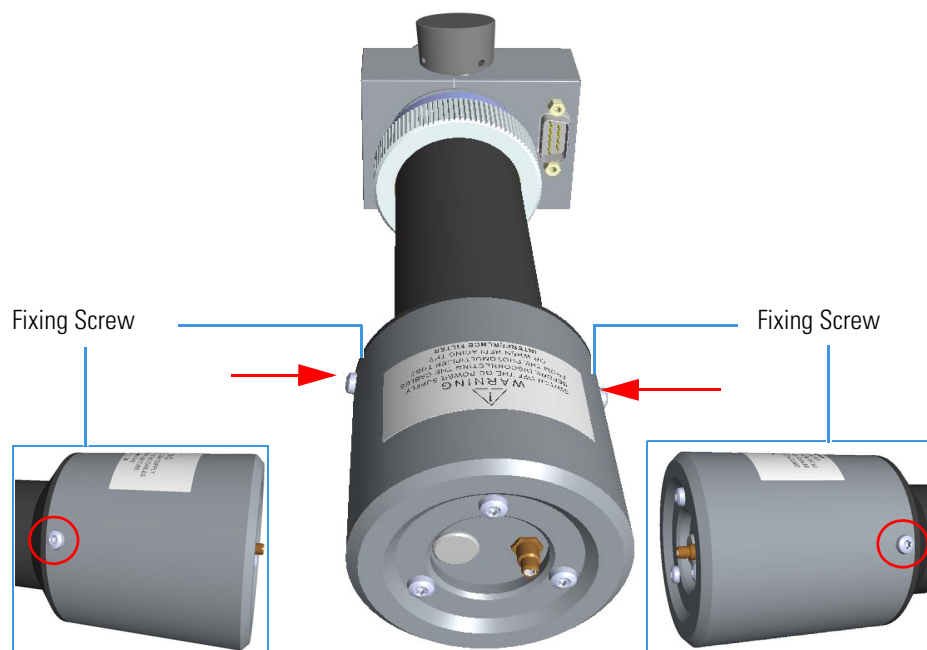
Figure 325. Photomultiplier Tube Housing Reinstallation (3)
