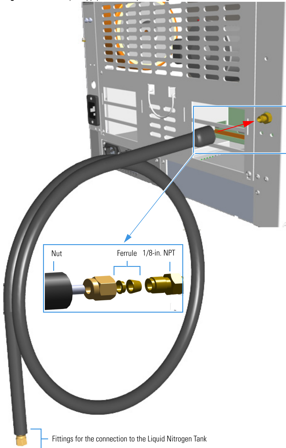
Figure 561. Oven Cryo Supply Tube for Liquid Nitrogen Connection
