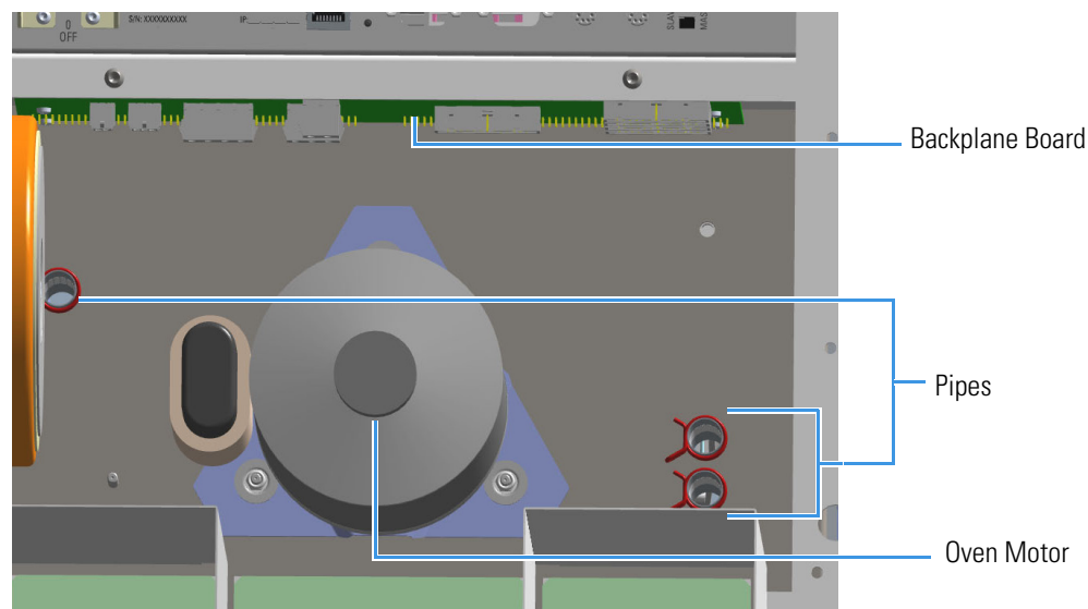
Figure 206. Pipes
