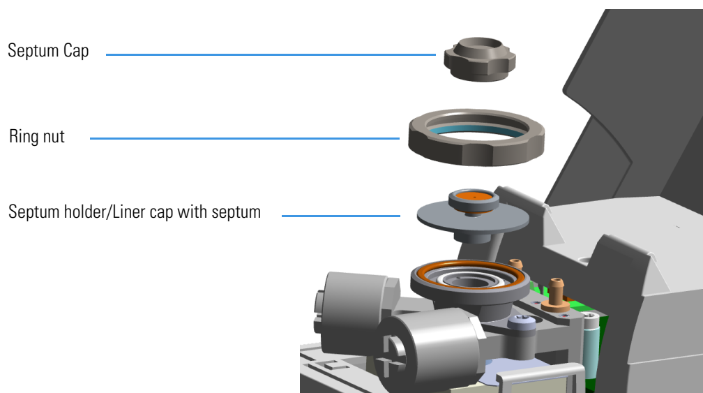
Figure 350. Injector Top Parts Removal
