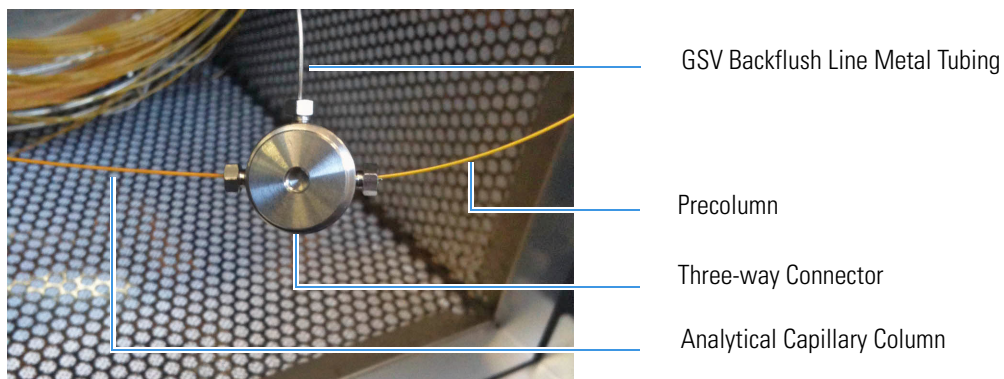
Figure 374. Connecting GSV Backflush Line, Precolumn, and Analytical Capillary Column
