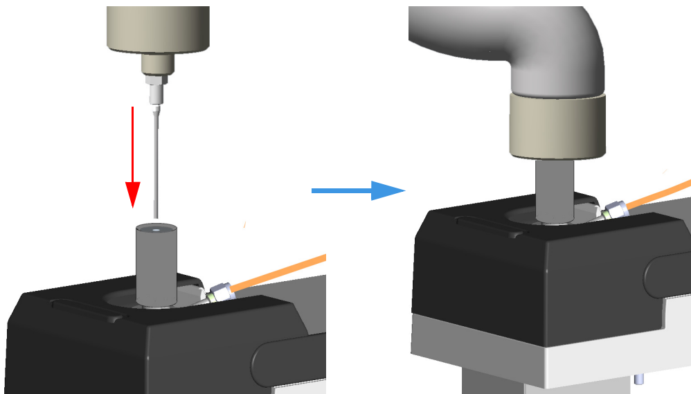
Figure 357. Transfer Line Connection
