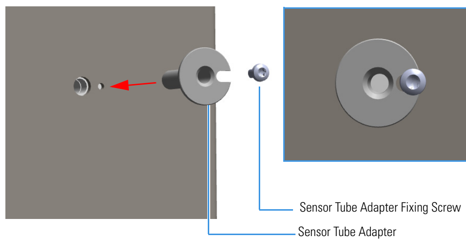
Figure 611. Sensor Tube Adapter Installation (1)
