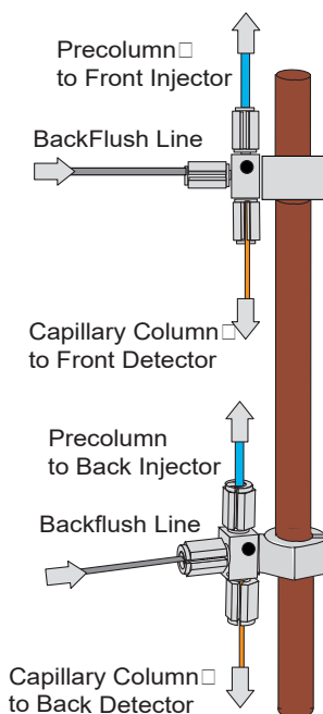
Figure 373. Schematically Connection of a Second Backflush System
