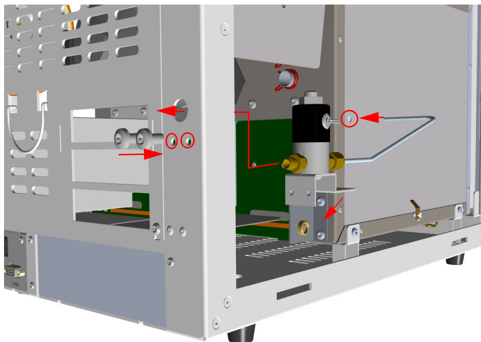
Figure 557. Installation of the Solenoid Valve Assembly for Carbon Dioxide
