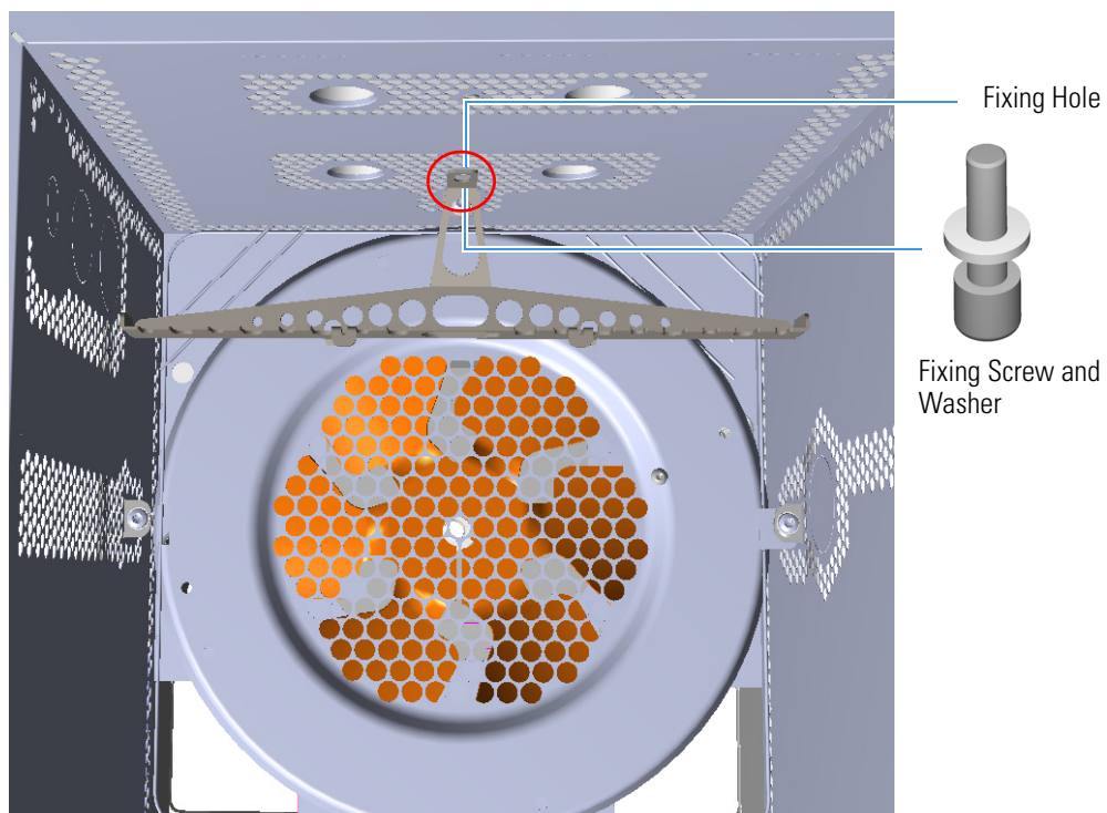
Figure 447. Kit Installation (3)
