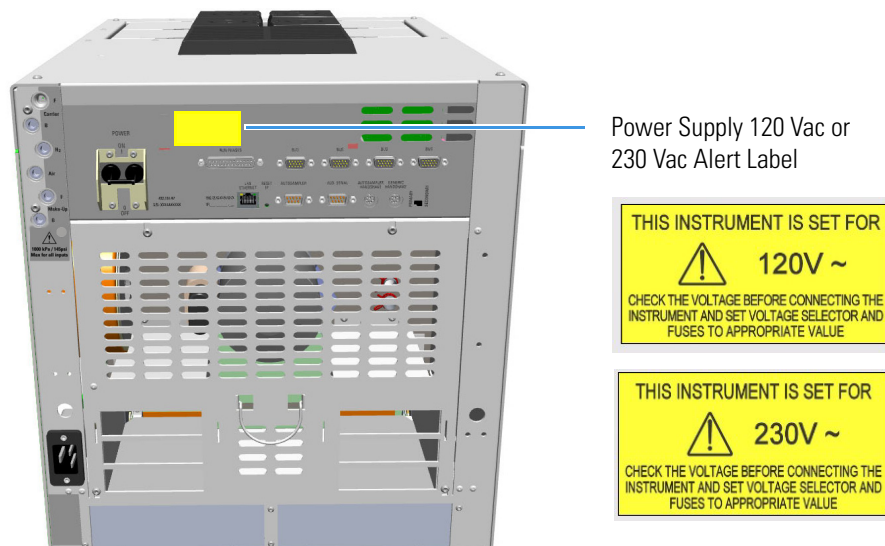
Figure 660. Identify Your Instrument: Power Supply Data
