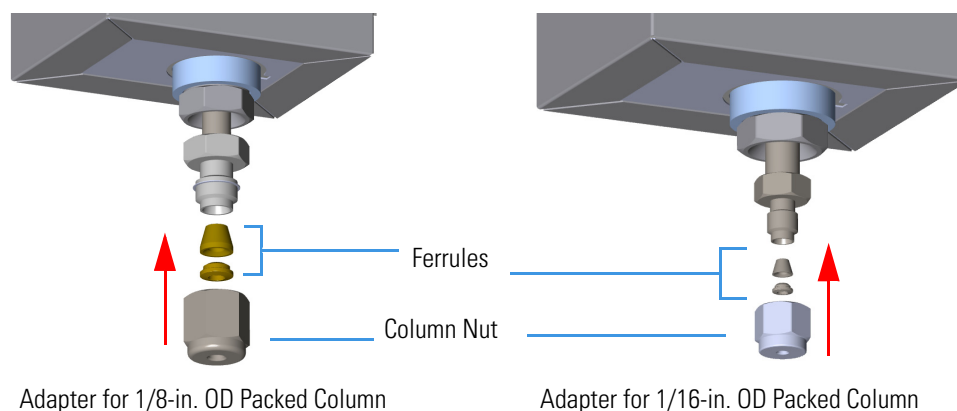
Figure 346. Column Nut and Ferrules (1)
