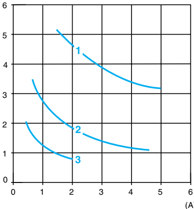
DC-12 : control of resistive loads and isolated solid state loads via optocoupler L/R \leq 1 \text{ ms}
