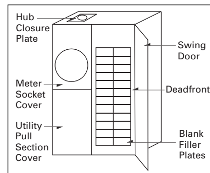
Figure 6. House Panel Line Diagram
