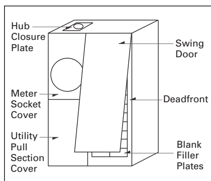
Figure 2. CGBT Style Line Diagram
