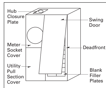
Figure 4. MBE Style Line Diagram
