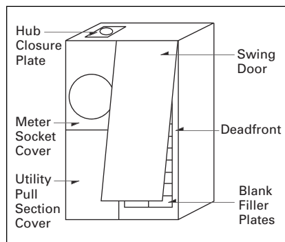
Figure 1. WMB Style Line Diagram
