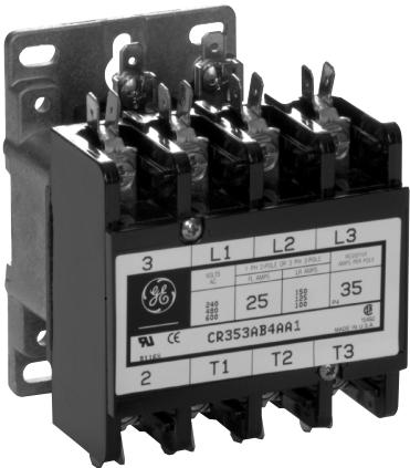
CR353A Contactor
