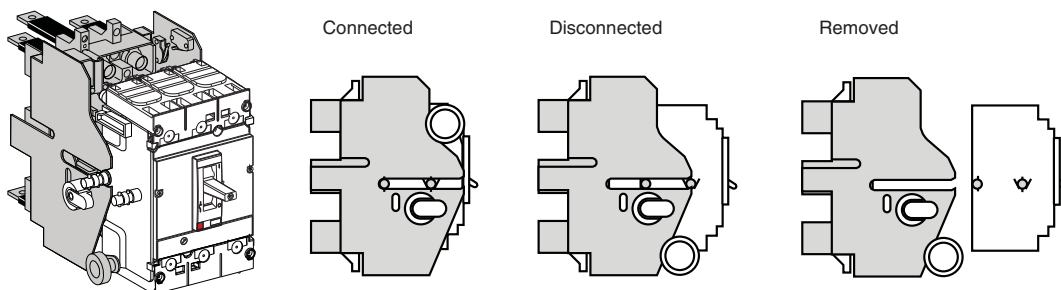
Figure 7: Drawout Mounting Positions
