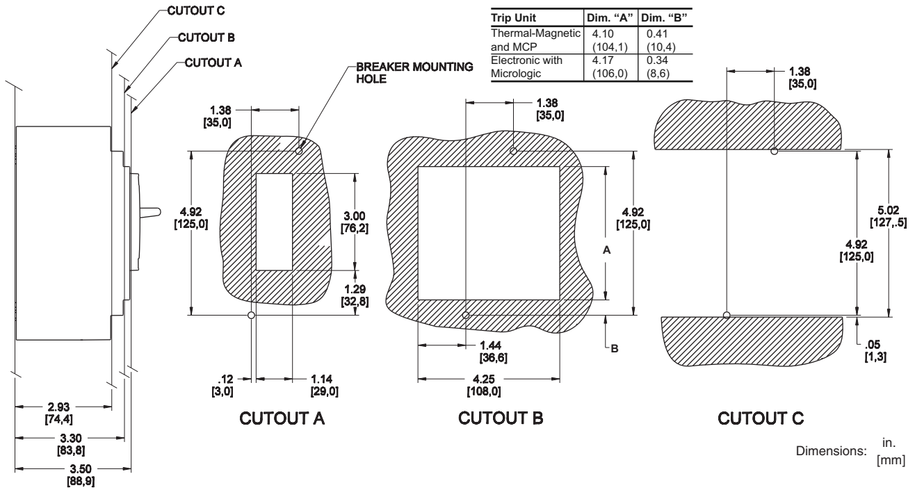
Figure 27: PowerPact H- and J-Frame Circuit Breaker Toggle Handle With Escutcheon Door Cutout
