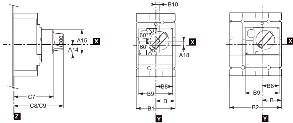
Figure 43: PowerPact L-Frame Circuit Breaker Rotary-Operating Handles
