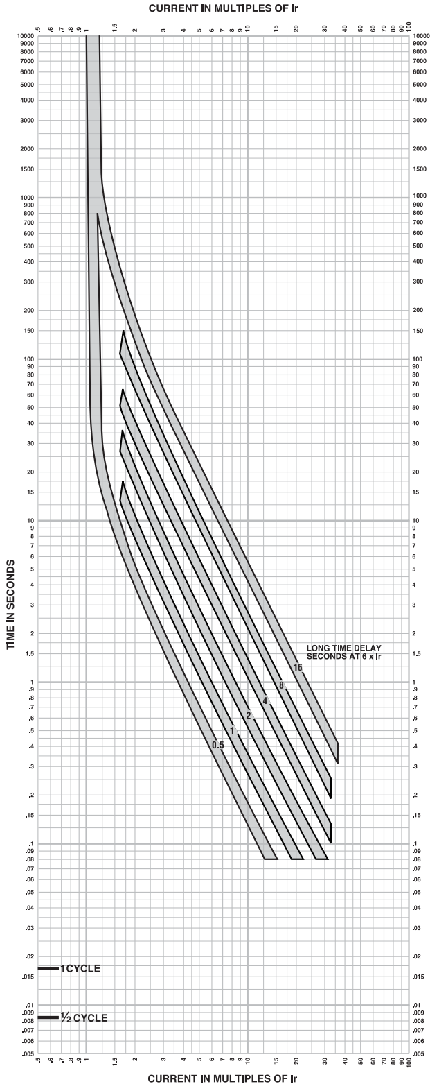
Figure 95: Micrologic 3.3 and 3.3-W Electronic Trip Unit Long Time Trip Curve
