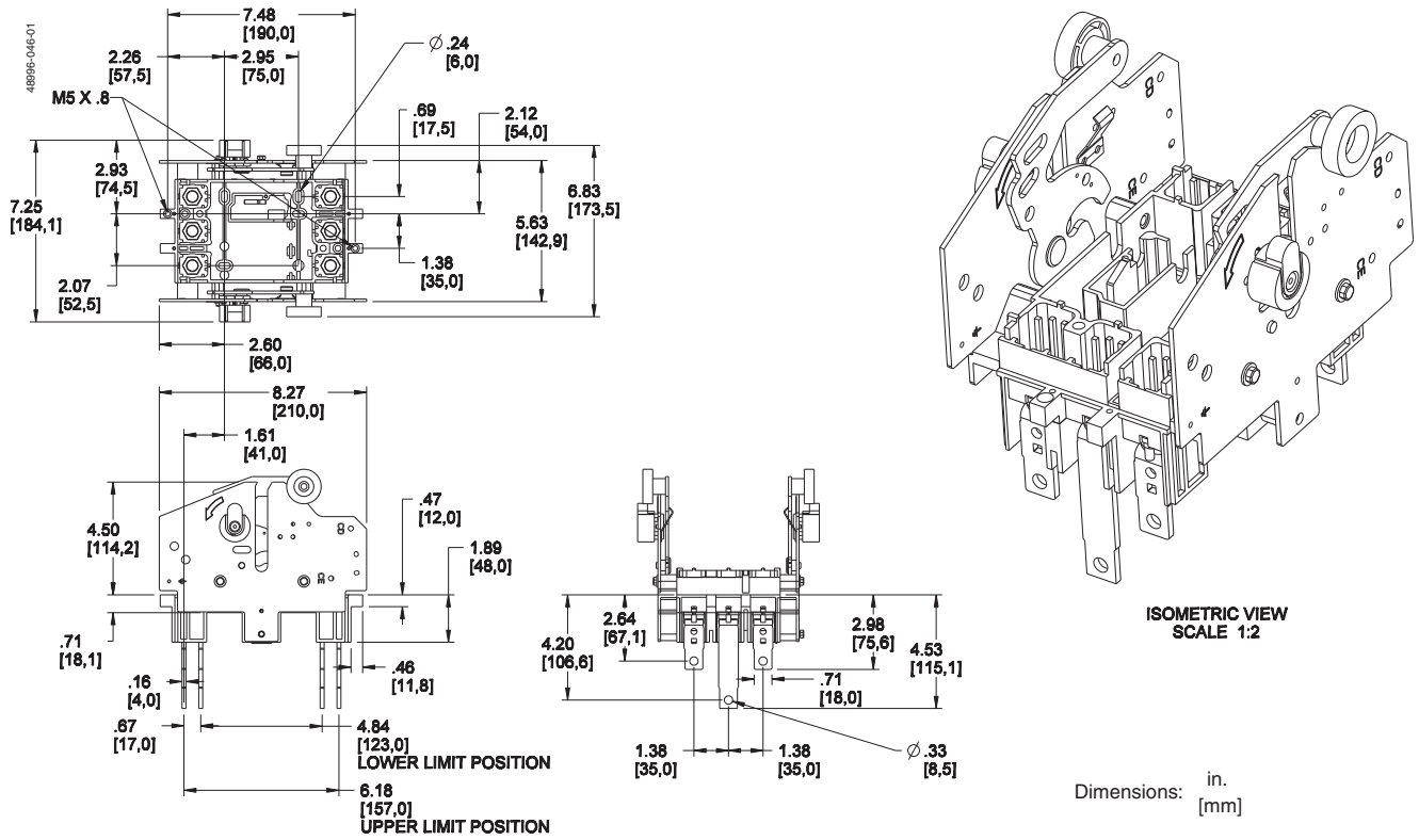
Figure 23: 15–250 A PowerPact H- and J-Frame Drawout 3P Circuit Breaker
