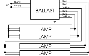
For three lamp operation, cap any blue lead, insulate to 600V DIAGRAM 7a
