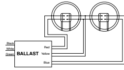
DIAGRAM 23 Series lamp operation
