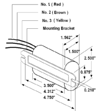
Ref. Drawing 33
