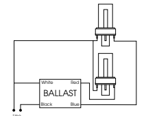
DIAGRAM 10 Parallel lamp operation
