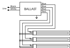
DIAGRAM 14 Parallel lamp operation + Cap unused blue lead; insulate to 600
