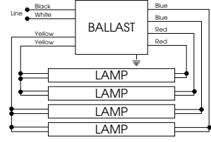
For Three Lamp Operation, Insulate one blue lead to 600V DIAGRAM 7
