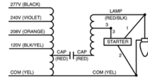
Wiring Diagram 11
