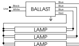
For Two Lamp Operation, Insulate one blue lead to 600V DIAGRAM 6
