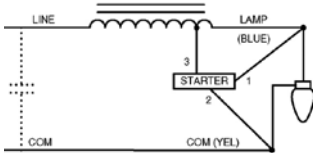
Wiring Diagram 1
