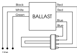
Mount lamp within 1" of grounded metal reflector. DIAGRAM 21
