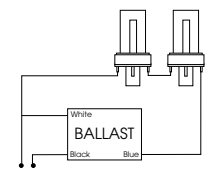
DIAGRAM 9 Series lamp opera-
