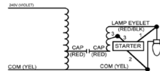
Wiring Diagram 40
