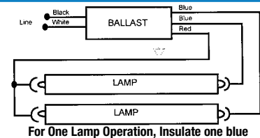
For One Lamp Operation, Insulate one blue lead to 600V
