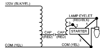
Wiring Diagram 38
