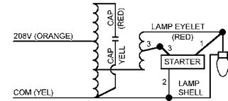
Wiring Diagram 37
