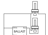
DIAGRAM 8 Parallel lamp operation
