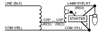
Wiring Diagram 40
