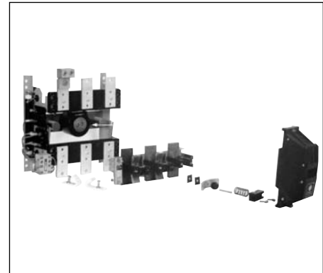
Typical NEMA Size 6 Contactor (exploded view)
