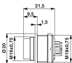
Solder connection: PV-..P1N126100
