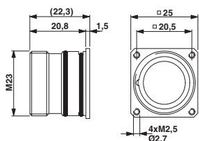
RC-00000004200, RC-00000005200 Radial O-ring
