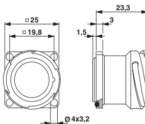
TU-0000000WB00 Axial O-ring
