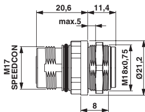
ST-17S1N8A6100S, ST-17P1N8A6100S, Separate ordering for locking nut
