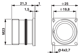
RC-00000002200 Flat gasket
