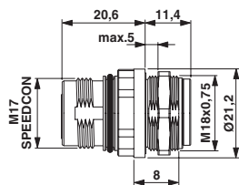
ST-ES1N8A6100S, ST-EP1N8A6100S Separate ordering for locking nut
