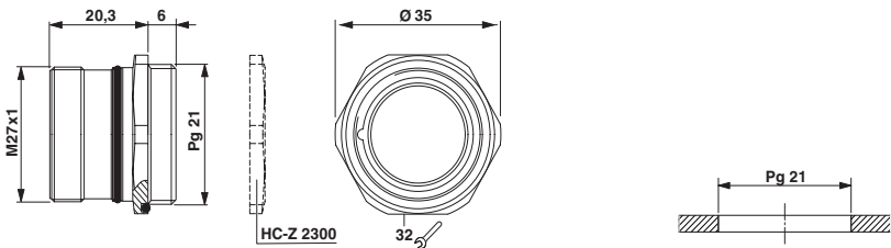
HC-..S1N1.6300 Axial O-ring
