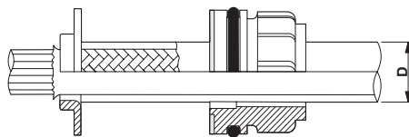
Universal cable clamp type cage with shield, D = external cable diameter
