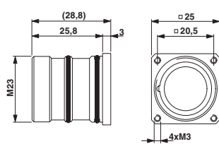
RC-0000000E000 Radial O-ring
