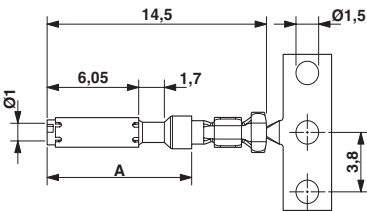
C-HC female contact Ø 1 mm A = D-SUB dimension
