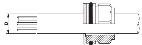
Universal cable clamp type cage, cable feed-through without shield, D=external cable diameter
