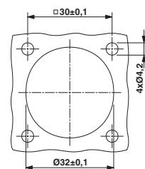
Installation dimensions: SM-EPWN8AA200
