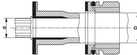
Diagram of stranded wire bundle diameter d and external cable diameter D
