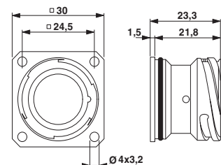
TU-00000005300 Radial O-ring
