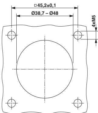
Installation dimensions (wire Ø max. 14 mm)
