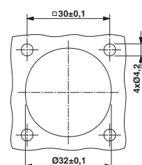
Installation dimensions: SM-EPWN8AWT00
