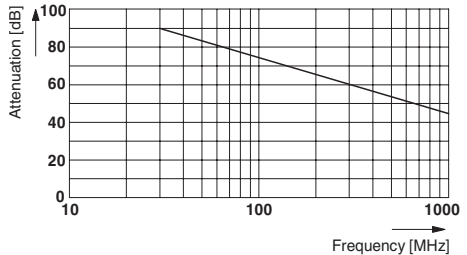
Shield attenuation curve UC / TU series based on DIN EN 50289-1-6
