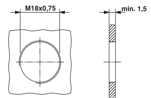
Installation dimensions: ST-E.1N8AH100S, feed-through hole with thread (recommended for installation in steel sheet panel)
