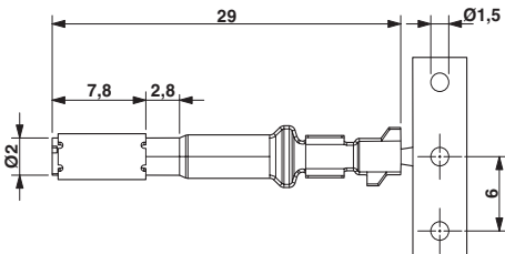
C-HC female contact Ø 2 mm
