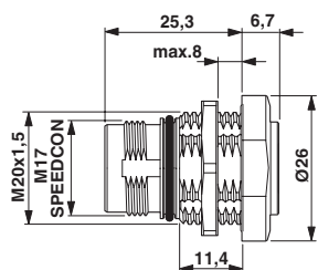
ST-17S1N8AH100S, ST-17P1N8AH100S, Separate ordering for locking nut
