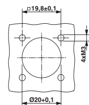
Installation dimensions: SF-ES1N8AYW00
