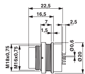
Solder-in connection: PV-..P1N22HG00
