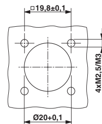
Installation dimensions
