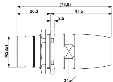
UC-0000000Q3DU, UC-0000000QNDU (Axial O-ring)
