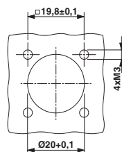
Installation dimensions: SF-EP1N8AAF00
