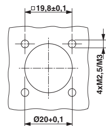
Installation dimensions
