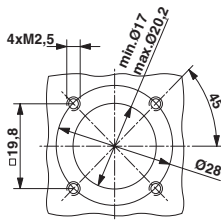
Installation dimensions: ST-17.1N8AAC00S
