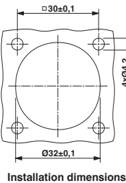
Installation dimensions
