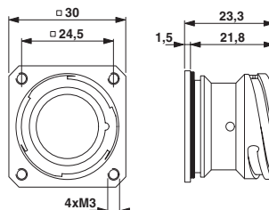
TU-00000004100 Flat gasket
