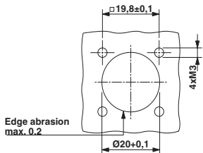
Installation dimensions: SF-EP1N8AAD00
