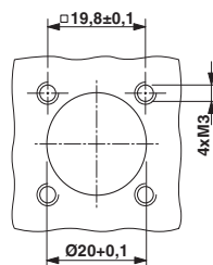
Installation dimensions: SF-EP1N8AWA00
