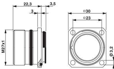
HC-...1N..WA00 Radial O-ring
