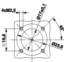
Installation dimensions: ST-17.1N8AAD00S
