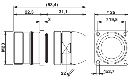
RC-0000000B2FZ Radial O-ring
