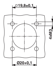
Installation dimensions: RF-1.S..8AAF00, RF-1.P..8AAF00
