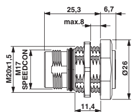
ST-ES1N8AH100S, ST-EP1N8AH100S Separate ordering for locking nut
