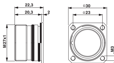
HC-...1N..4300 Radial O-ring
