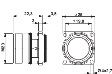
RC-0000000WQ00 Radial O-ring
