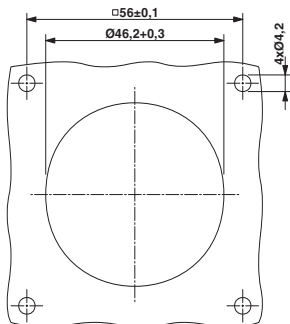
Installation dimensions
