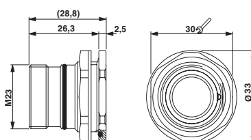
RC-0000000H000 Axial O-ring
