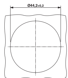
Installation dimensions
