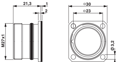
HC-...1N..2300 Flat gasket
