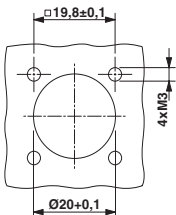
Installation dimensions
