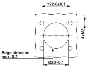
Installation dimensions: SF-EP1N8AAC00
