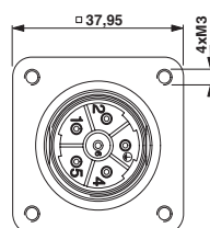
Flange dimensions: SF-EP1N8AC0.., SF-EP1N8ACL..
