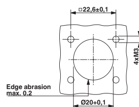
Installation dimensions: RF-1.S..8AAC00, RF-1.P..8AAC00
