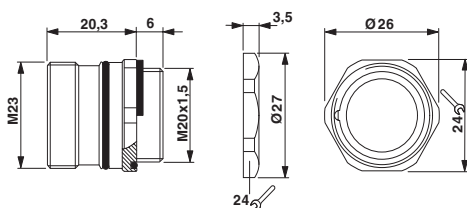
RC-00000006100 Axial O-ring
