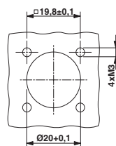
Installation dimensions: SF-ES1N8AY000
