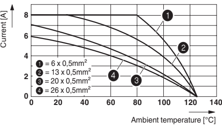
Derating curve based on DIN EN 60512-5-2 Cable plug connector (26-pos.)
