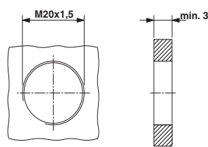
RC-00000006100 , mounting feed-through hole with thread (recommended for installation in steel sheet panel)
