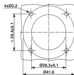
Installation dimensions: SF-EP1N8AC0.., SF-EP1N8ACL..
