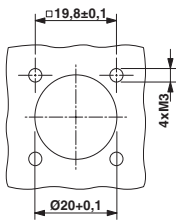
Installation dimensions: SF-EP1N8AA200
