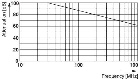
RC series shield attenuation curve based on DIN EN 50289-1-6
