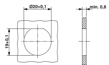
RC-00000006100 , mounting hole with polarization and locking nut (recommended for installation in steel sheet panel)
