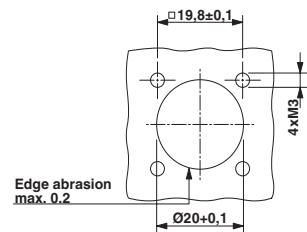
Installation dimensions: RC-0000000AD00
