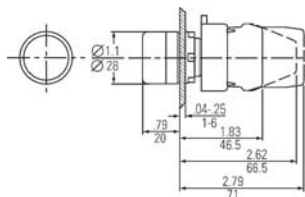
Round Illuminated Flush Push Button
