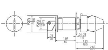
Round Plastic Emergency Stop Key-to-Release
