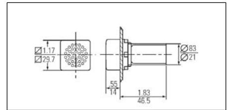
Square Buzzer
