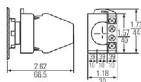
Double Contact Blocks with Screw Terminals
