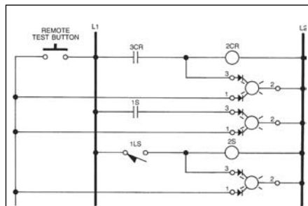
Typical wiring diagram for remote test of lights using dual input "remote test" lights.
