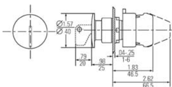
Round Metal Emergency Stop Key-to-Release
