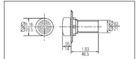
Round Buzzer
