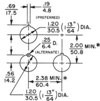
Drilling Plan Dual Dimensions
