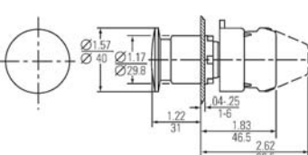
Round Push-Pull Mushroom-Head Push Button
