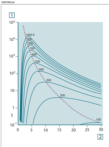
Figure 22.6 Planck curves plotted on semi-log scales from 100 K to 1000 K. The dotted line represents the locus of maximum radiant emittance at each temperature as described by Wien's displacement law. 1: Spectral radiant emittance ( \text{W}/\text{cm}^2 (\mu\text{m}) ); 2: Wavelength ( \mu\text{m} ).
