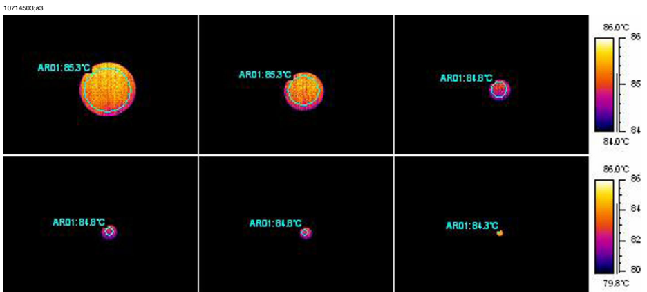
Figure 17.19 Temperature readings from a blackbody at +85^{\circ}\text{C} ( +185^{\circ}\text{F} ) at increasing distances
