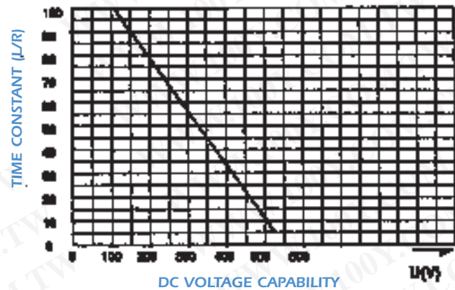
DC Voltage Capability vs. Time Constant
