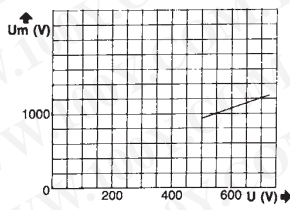
Peak arc voltage
