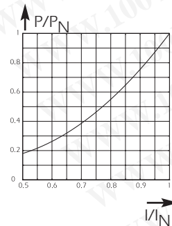
Left: Curve enables computation of power losses P for a I_N -rated fuse as a function of the R.M.S. current I (as a multiple of I_N for steady state operation)
