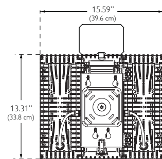
2 LED Array Top View
