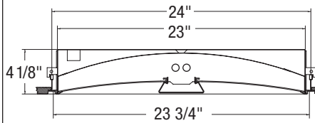
ML4U Cross-Section, (2) T5 Lamp
