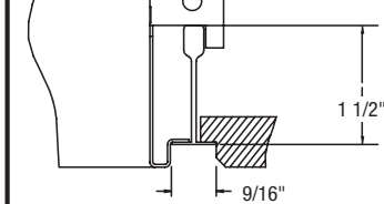
Lay-In Ceilings, 9/16" (ML4U) (tegular ceiling)
