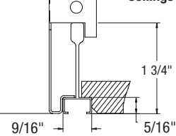
Slot-Grid Ceilings (ML4U)
