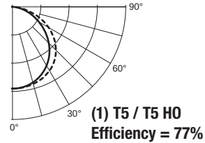
Slot-Grid Ceilings (ML4U)
