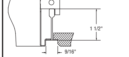
Lay-In Ceilings, 9/16" (ML4U) (tegular ceiling)
