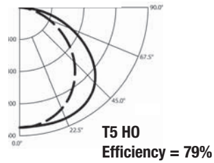
Photometric Data
