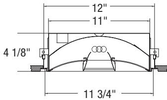
Lay-In Ceilings, 15/16" (ML4U)
