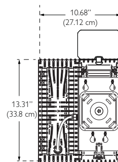
1 LED Array Top View
