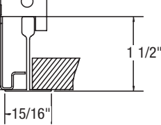
Lay-In Ceilings, 15/16" (ML4U)
