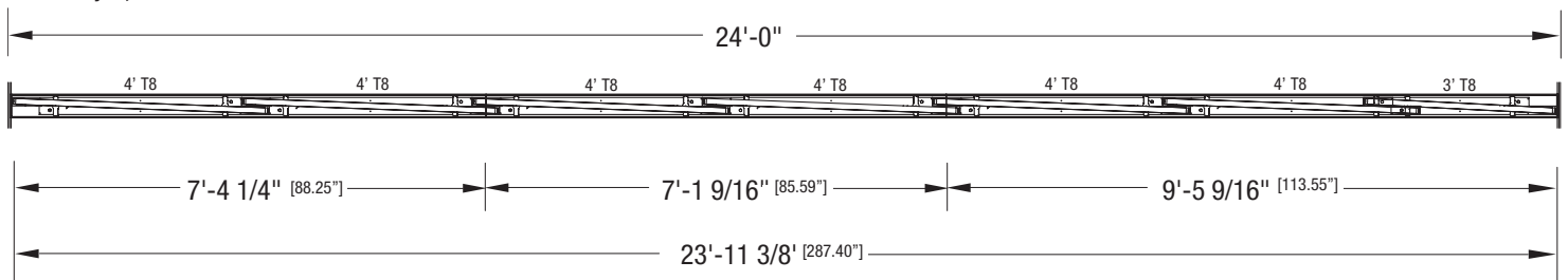
24' T8 - Lay-In, Flush/Slot Grid
