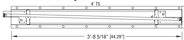
4' T5 End - After Sheetrock Flangeless
