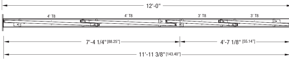
16' T8 Individual - Lay-In, Flush/Slot Grid
