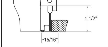
Lay-In Ceilings, 15/16" (ML4U)
