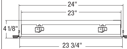
ML4U Side View
