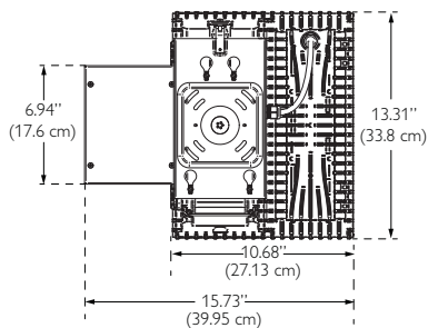
1 LED Array Side View
