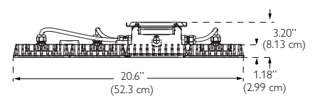
3 LED Array Side View
