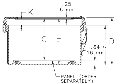
SECTION X-X
