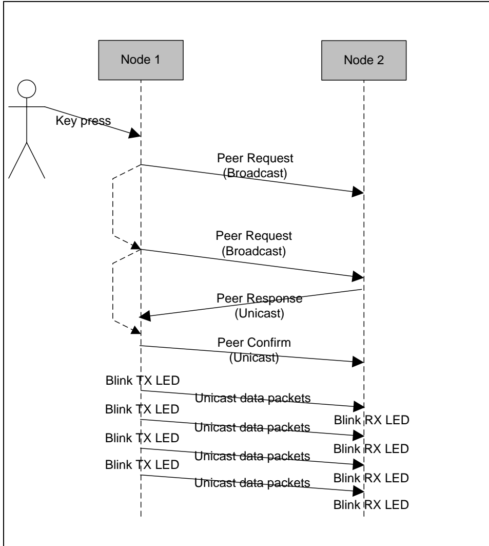
Figure 10-2. Sequence diagram of Range measurement
