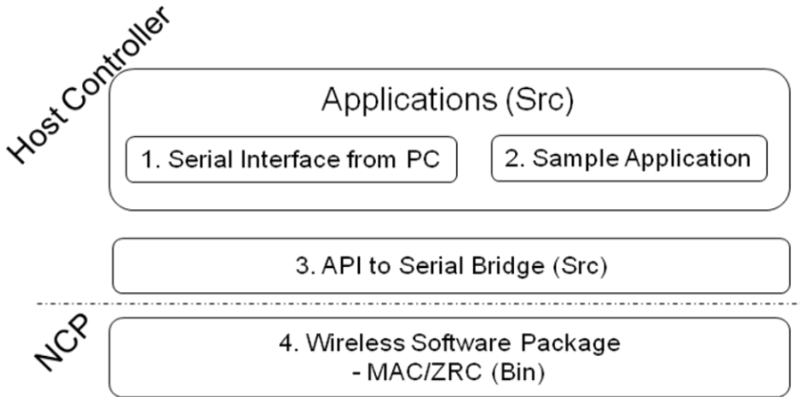
Figure 3-2. Host NCP approach
