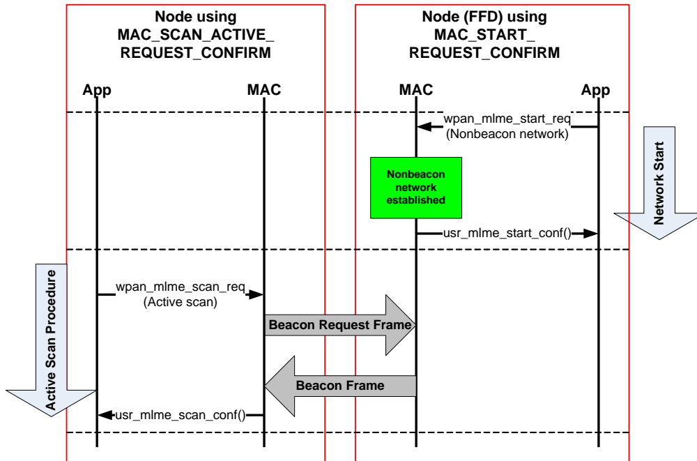
Figure 5-13. Start of non-beacon network and active scan.
