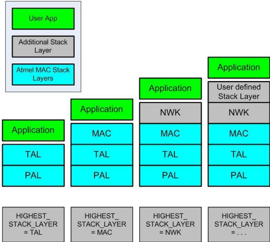
Figure 2-2. Stack usage.
