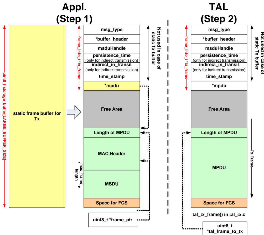
Figure 5-6. Frame buffer handling during frame transmission using TAL-API.
