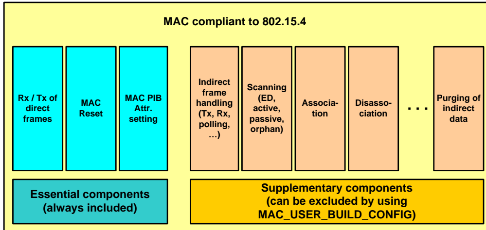
Figure 5-9. Essential and supplementary MAC components.
