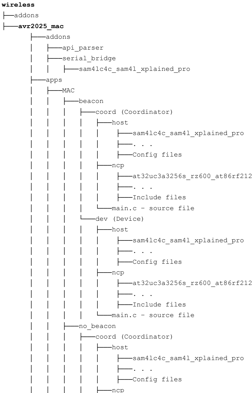
Figure 3-1. Avr2025_mac package directory Structure
