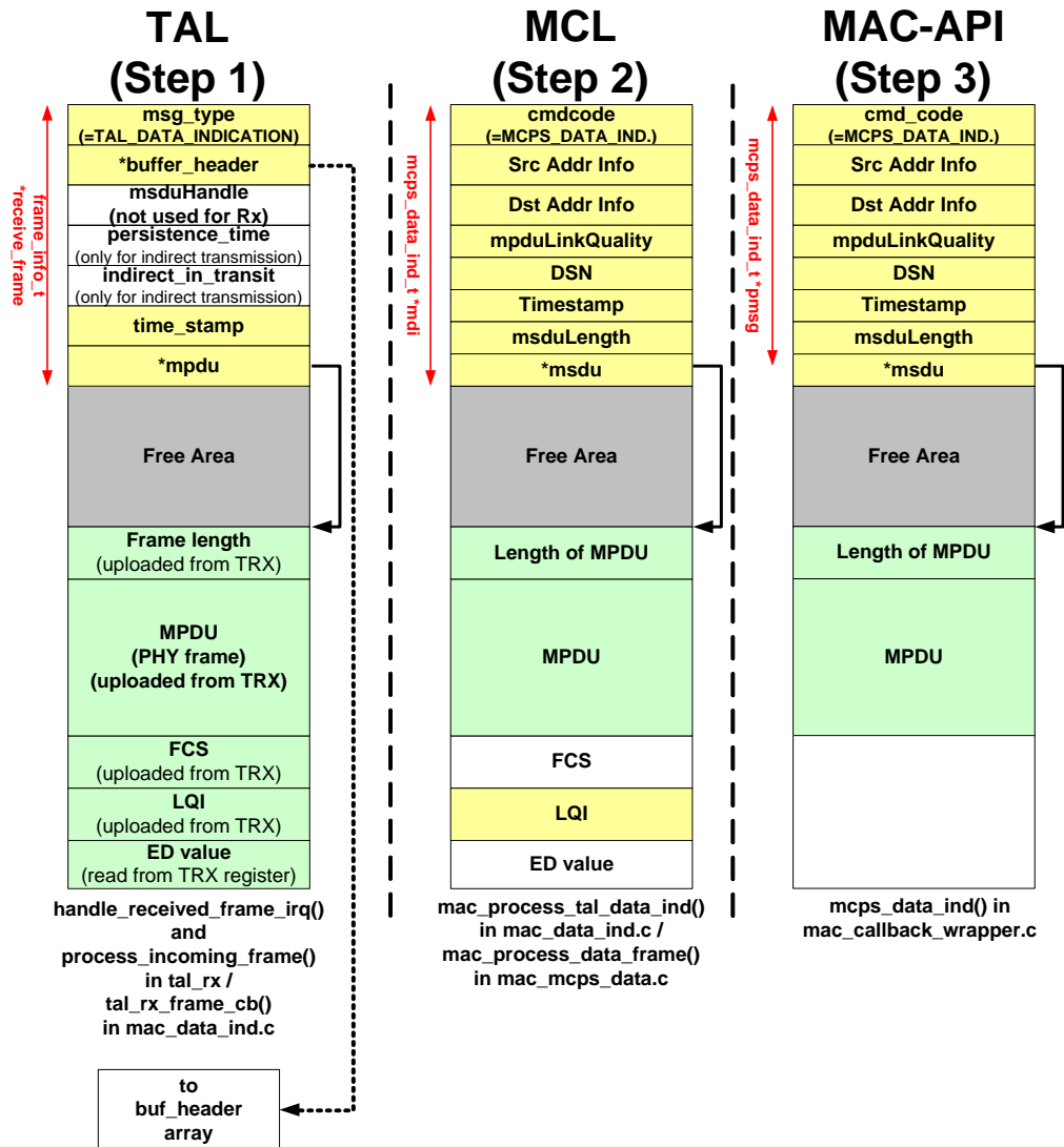
Figure 5-5. Frame buffer handling during data frame reception.
