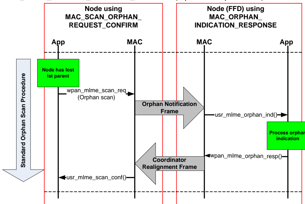
Figure 5-12. Provided functionality for MAC_ORPHAN_INDICATION_RESPONSE and MAC_SCAN_ORPHAN_REQUEST_CONFIRM (orphan scan procedure).
