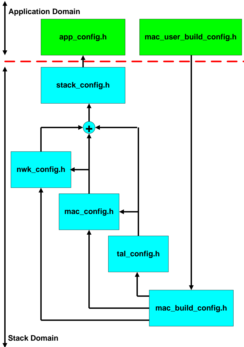
Figure 5-8. Configuration file #include-hierarchy.
