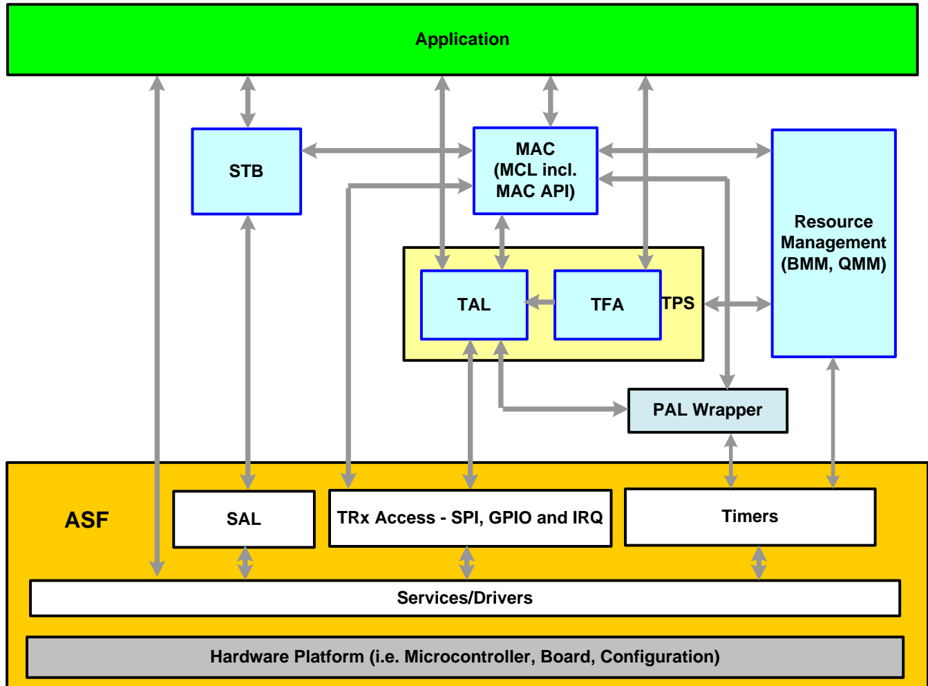
Figure 2-1. MAC architecture.
