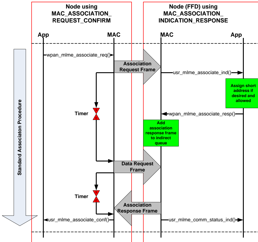
Figure 5-11. Provided functionality for MAC_ASSOCIATION_INDICATION_RESPONSE and MAC_ASSOCIATION_REQUEST_CONFIRM .
