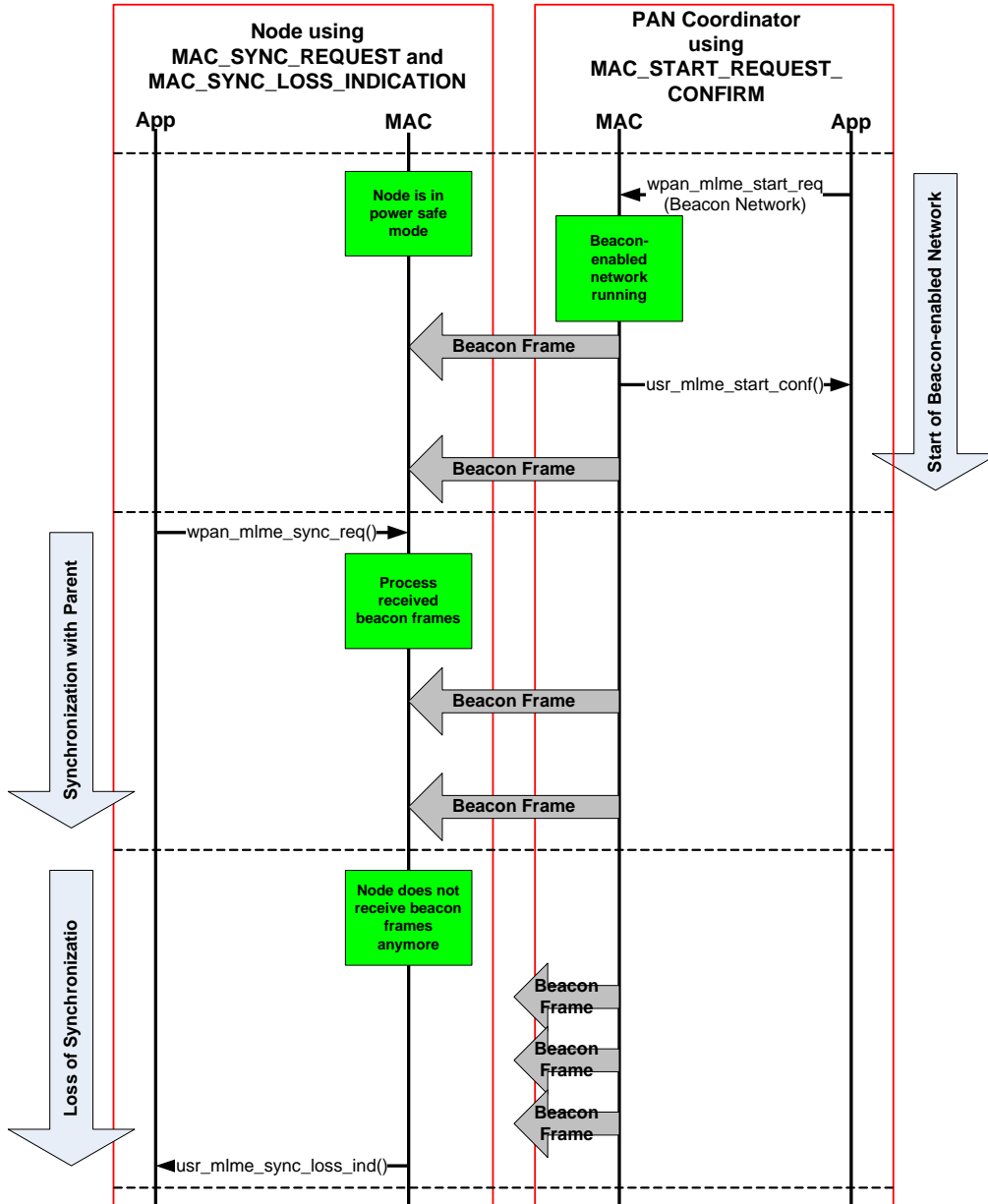
Figure 5-15. Synchronization and loss of synchronization.
