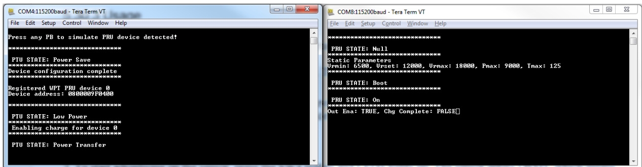
Figure 33. PTU and PRU after connecting, registering and enabling charge
