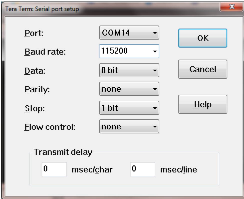
Figure 6. Tera Term – mbed serial port configuration
