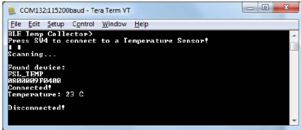
Figure 22. Tera Term – Output Console on Temperature Collector
