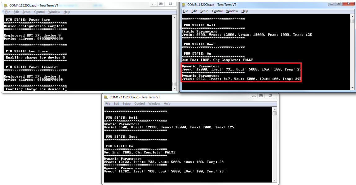
Figure 37. Power sharing support on one PRU
