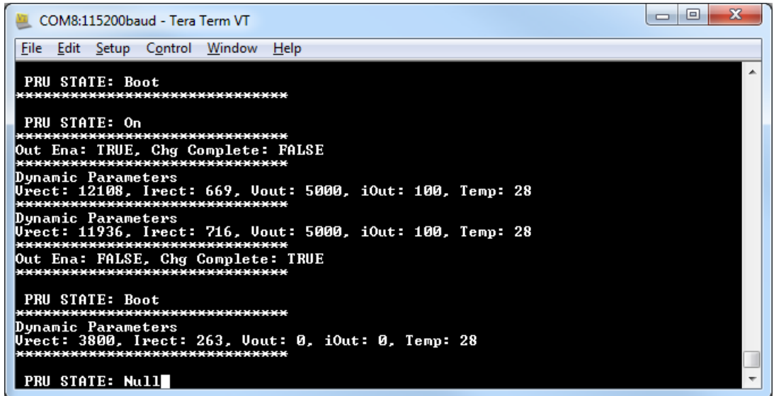
Figure 36. PRU power removed
