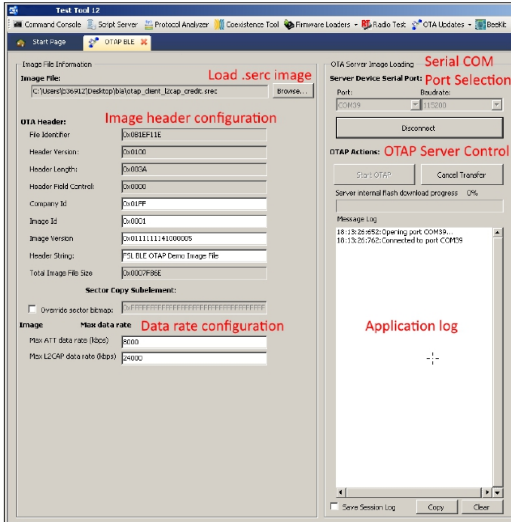
Figure 28. Test Tool BLE OTAP Application Overview
