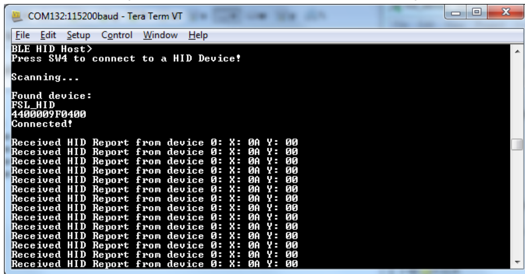
Figure 15. Tera Term – Output Console on HID Host with 1 peripheral connected
