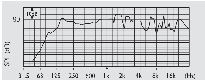
Frequency response
