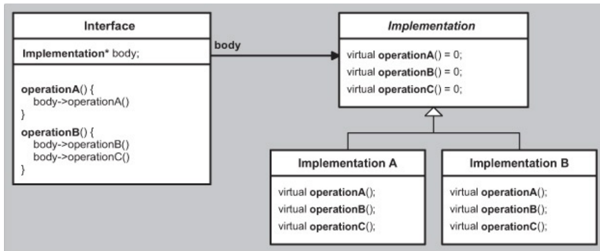
Figure 18.3. Bridge pattern implemented using inheritance
