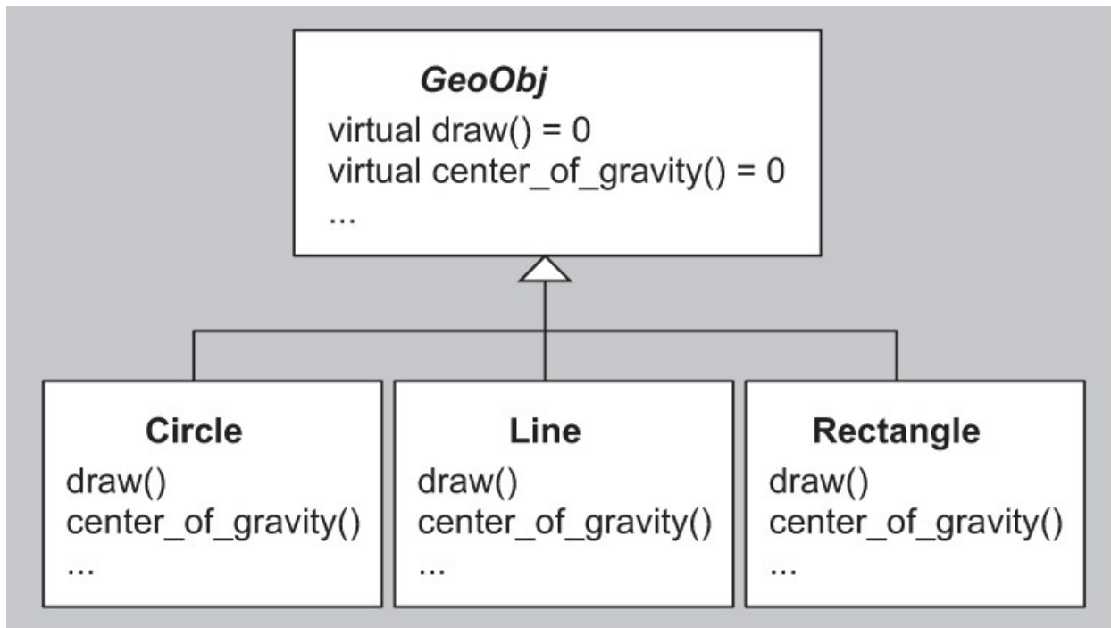
Figure 18.1. Polymorphism implemented via inheritance
