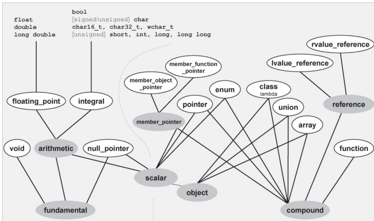
Figure D.1. Primary and Composite Type Categories
