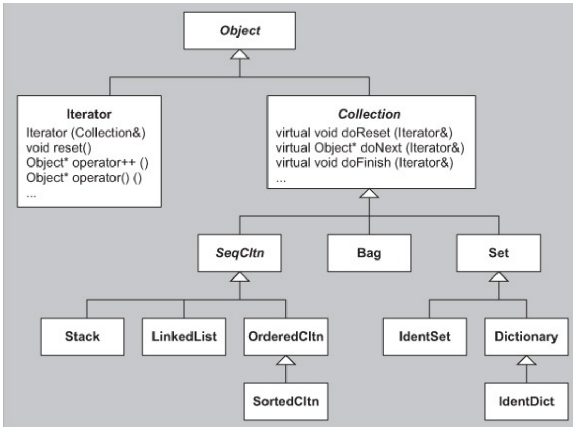
Figure 18.5. Class hierarchy of the NIHCL
