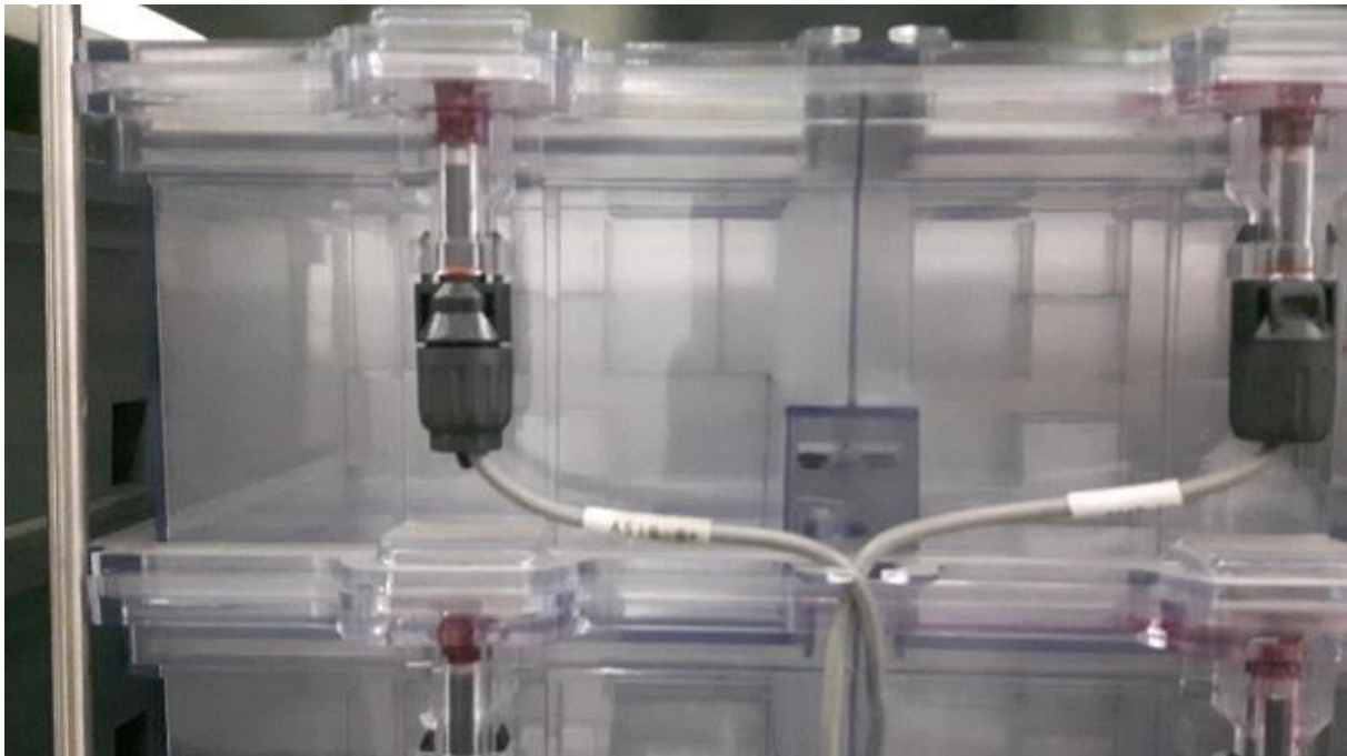
Figure: transparent battery cell (modular building block) and its connections
