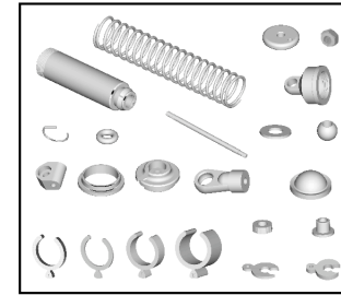
PD0560-T REAR SHOCK SET
