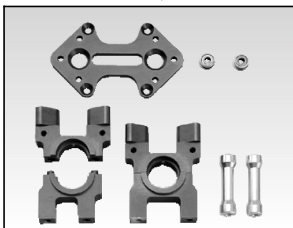
PD0787 ERGAL DECOMPOSABLE CENTER DIFF. MOUNT
