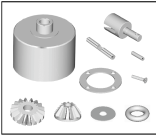
PD0548 FR / RR DIFFERENTIAL SET
