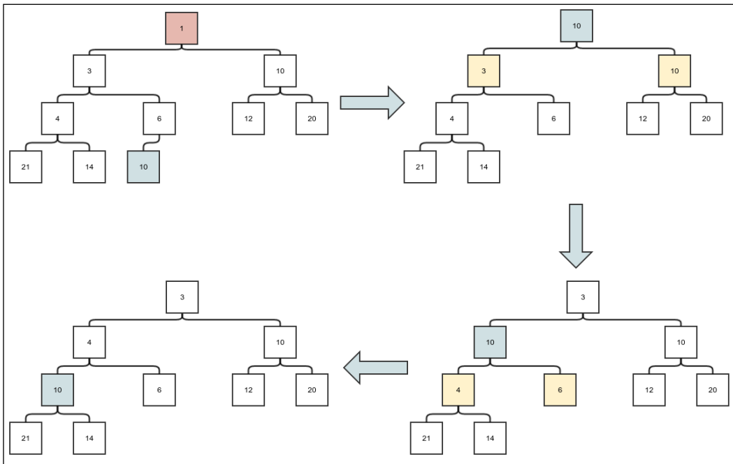
Heap deletion
