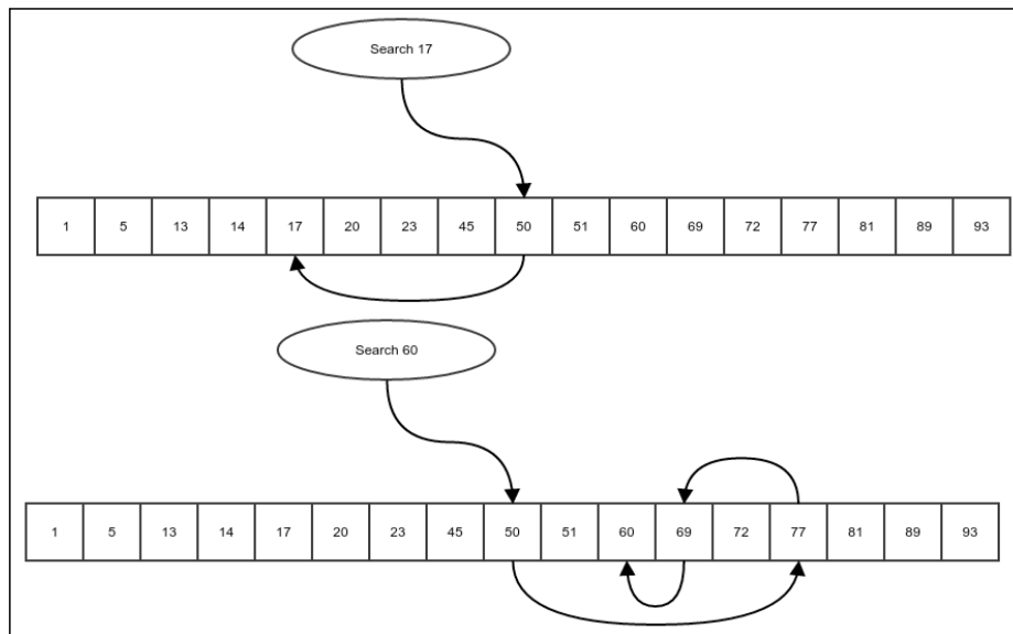
Figure 1: Binary Search.
