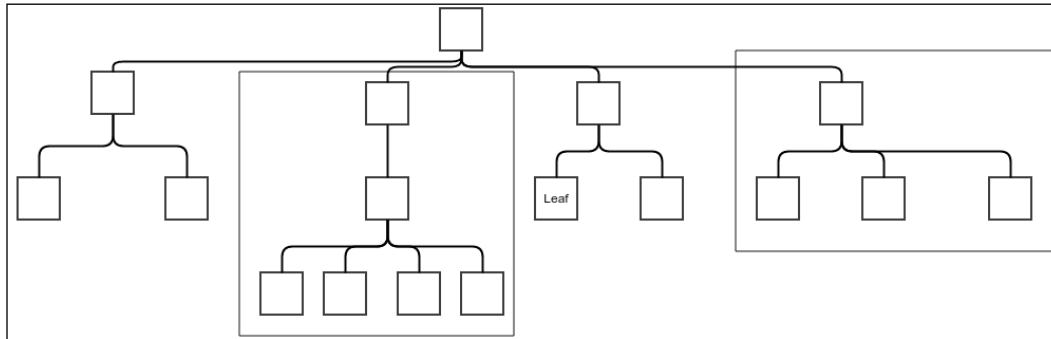
Examplesubtrees
