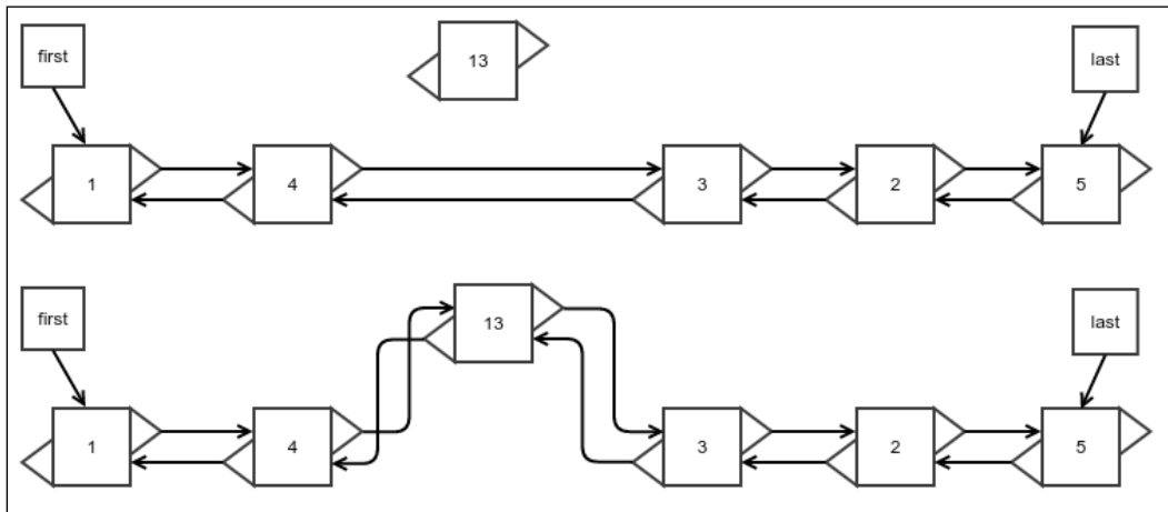
Figure 11: Insertion at an arbitrary location of a doubly linked list
