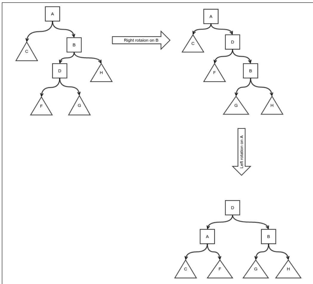
AVL tree double rotation
